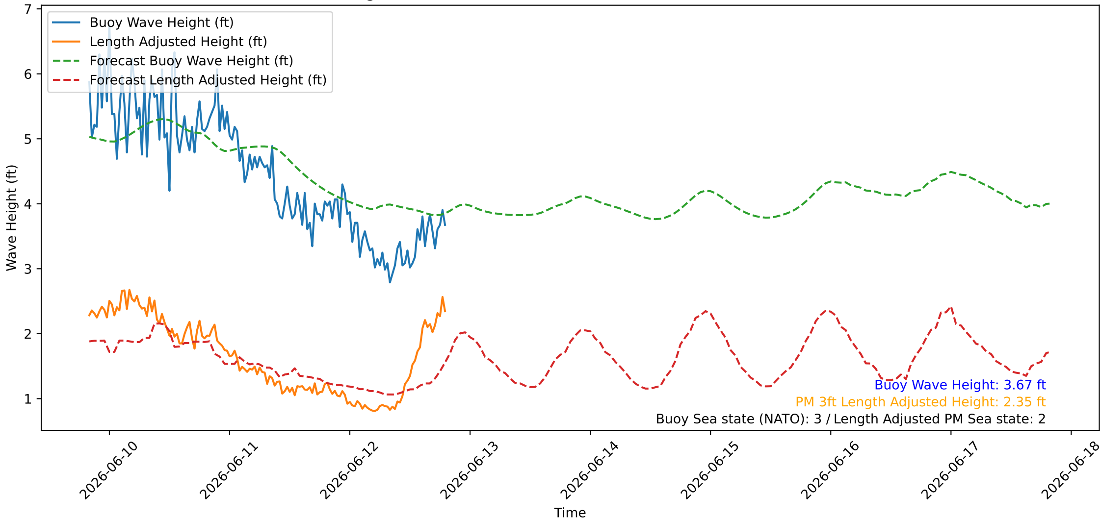
Wave Heights over Time for Oceanside Harbor at 2026-06-12 20:00:26
