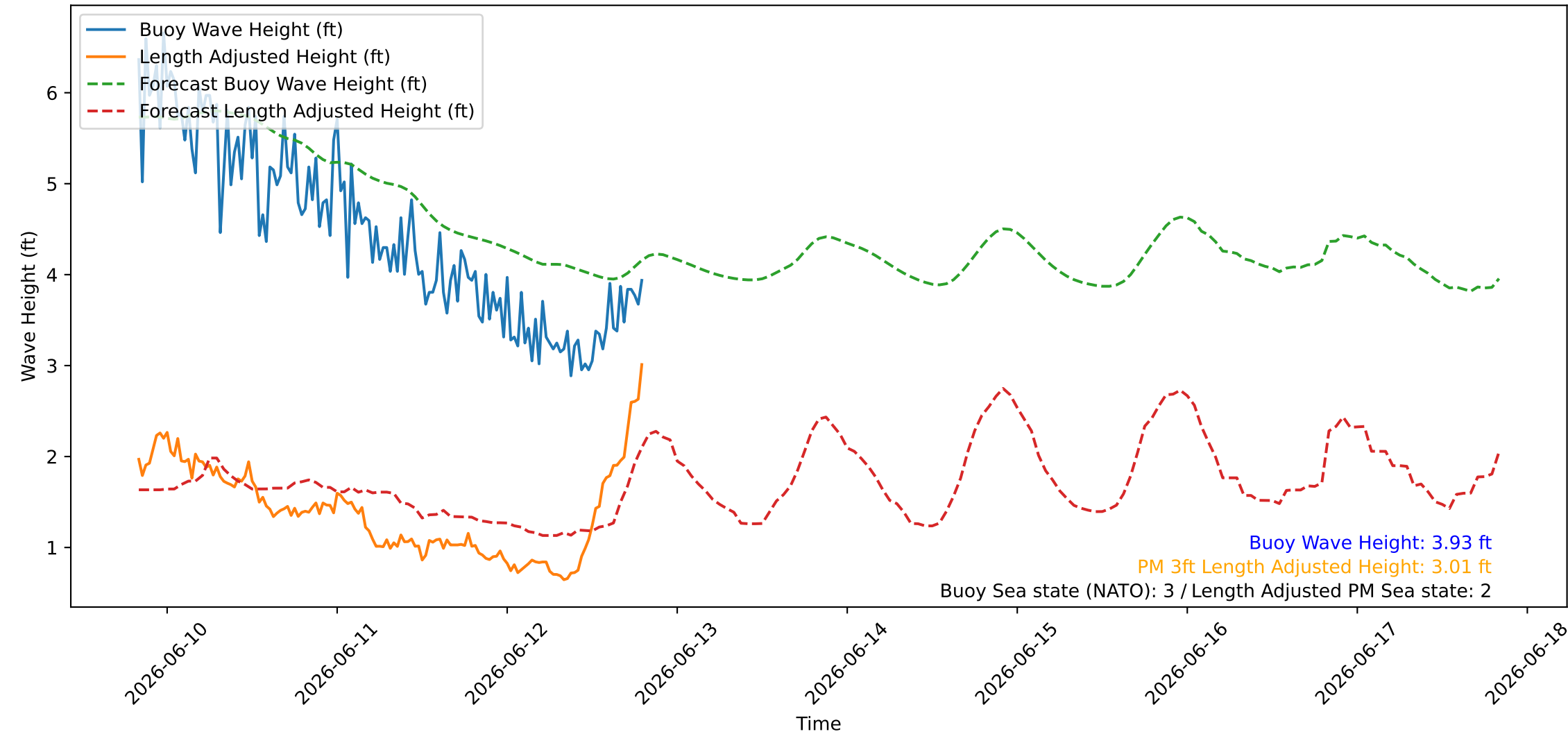
Wave Heights over Time for Green Beach at 2026-06-12 20:01:08
