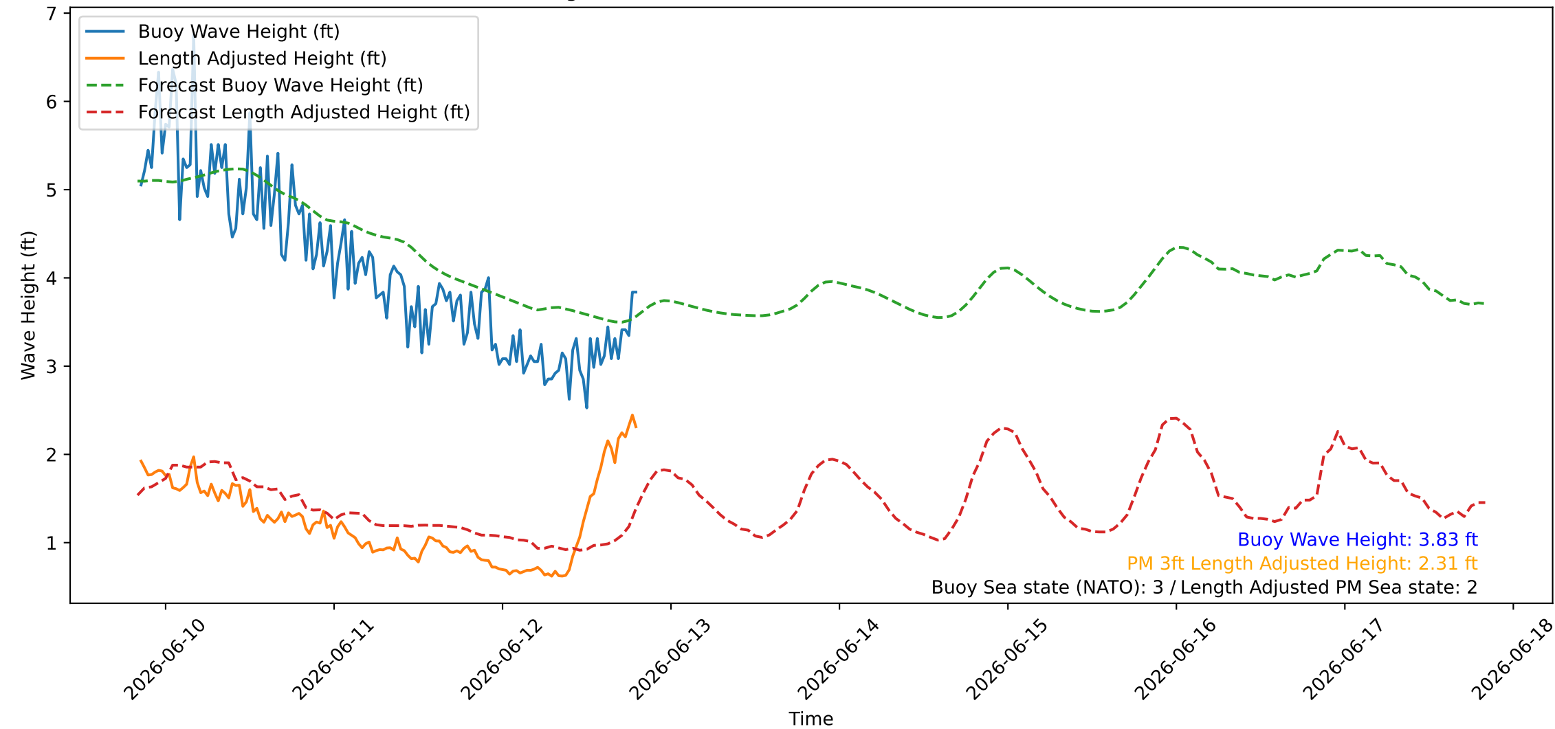
Wave Heights over Time for Red Beach at 2026-06-12 20:00:46
