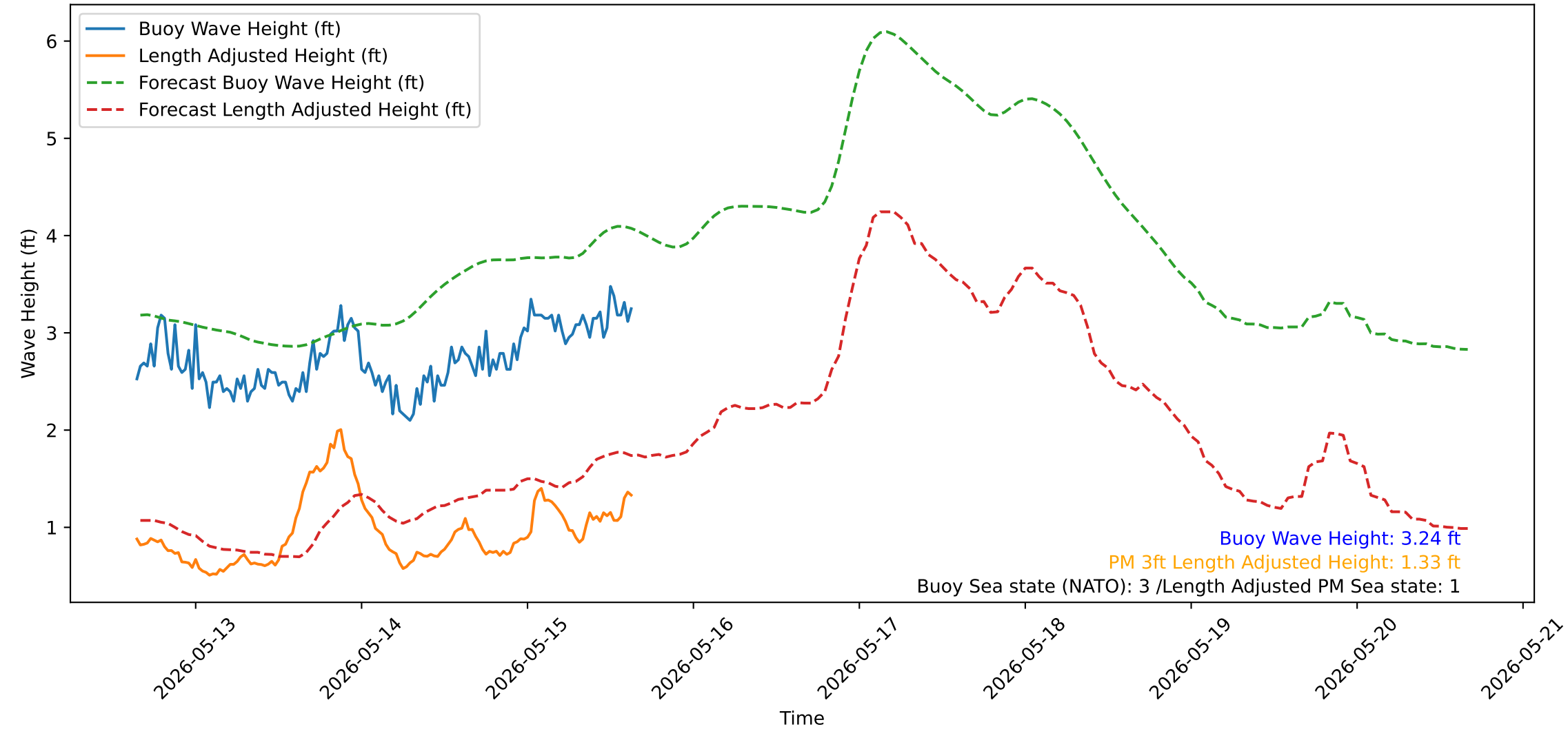
Wave Heights over Time for Green Beach at 2026-05-15 15:41:13
