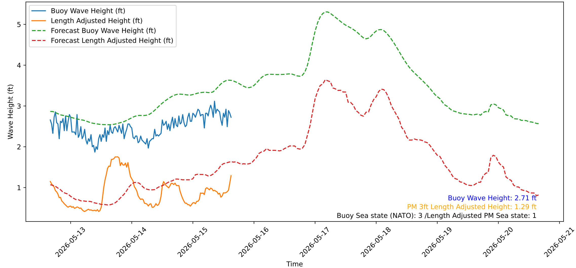
Wave Heights over Time for Red Beach at 2026-05-15 15:40:51
