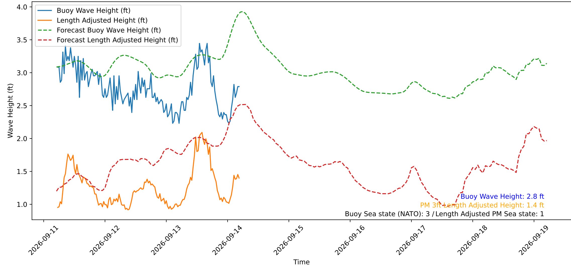
Wave Heights over Time for Red Beach at 2026-09-14 05:10:49
