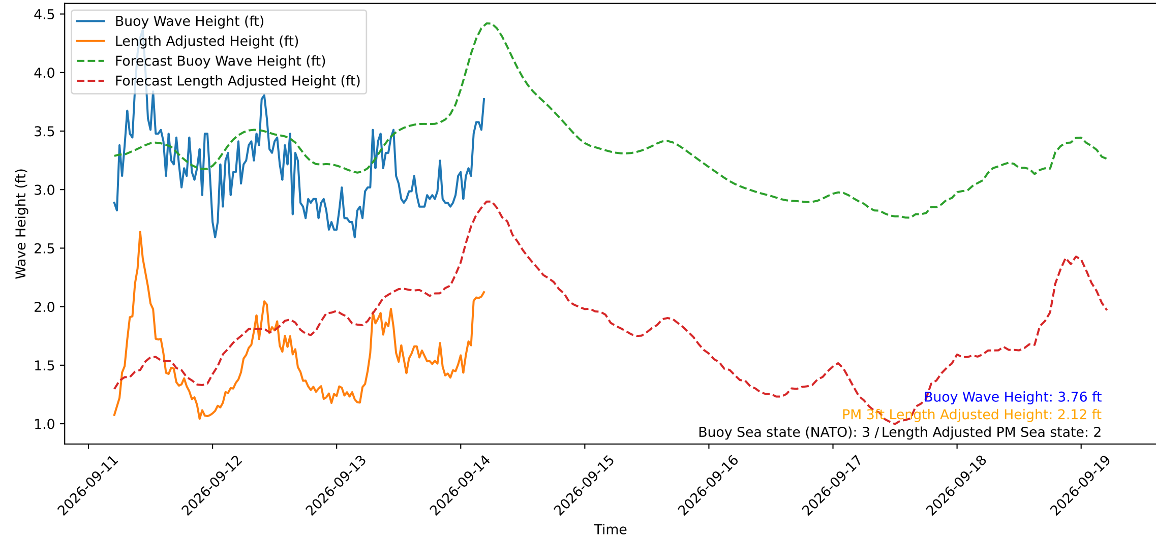
Wave Heights over Time for Oceanside Harbor at 2026-09-14 05:10:29
