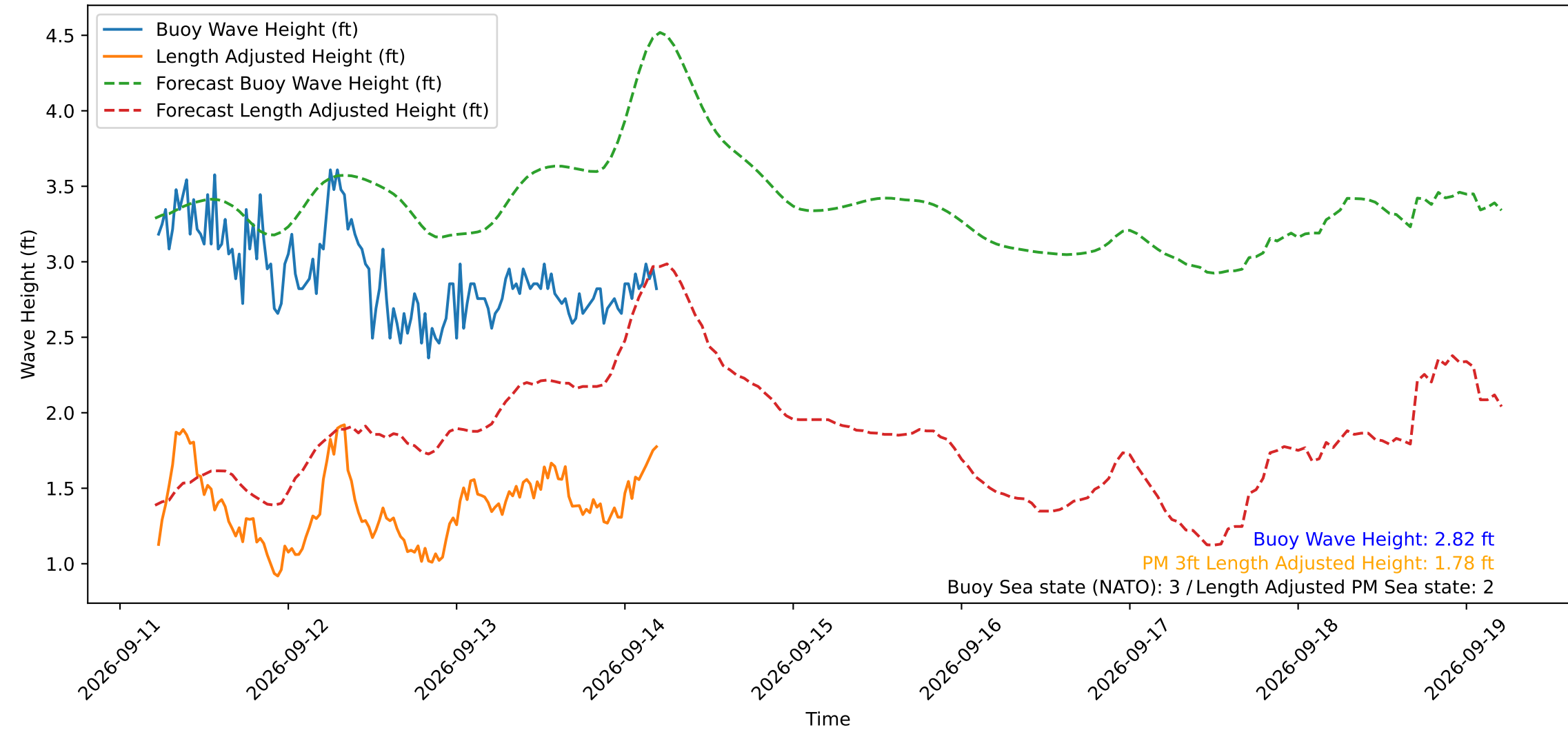
Wave Heights over Time for Green Beach at 2026-09-14 05:11:13
