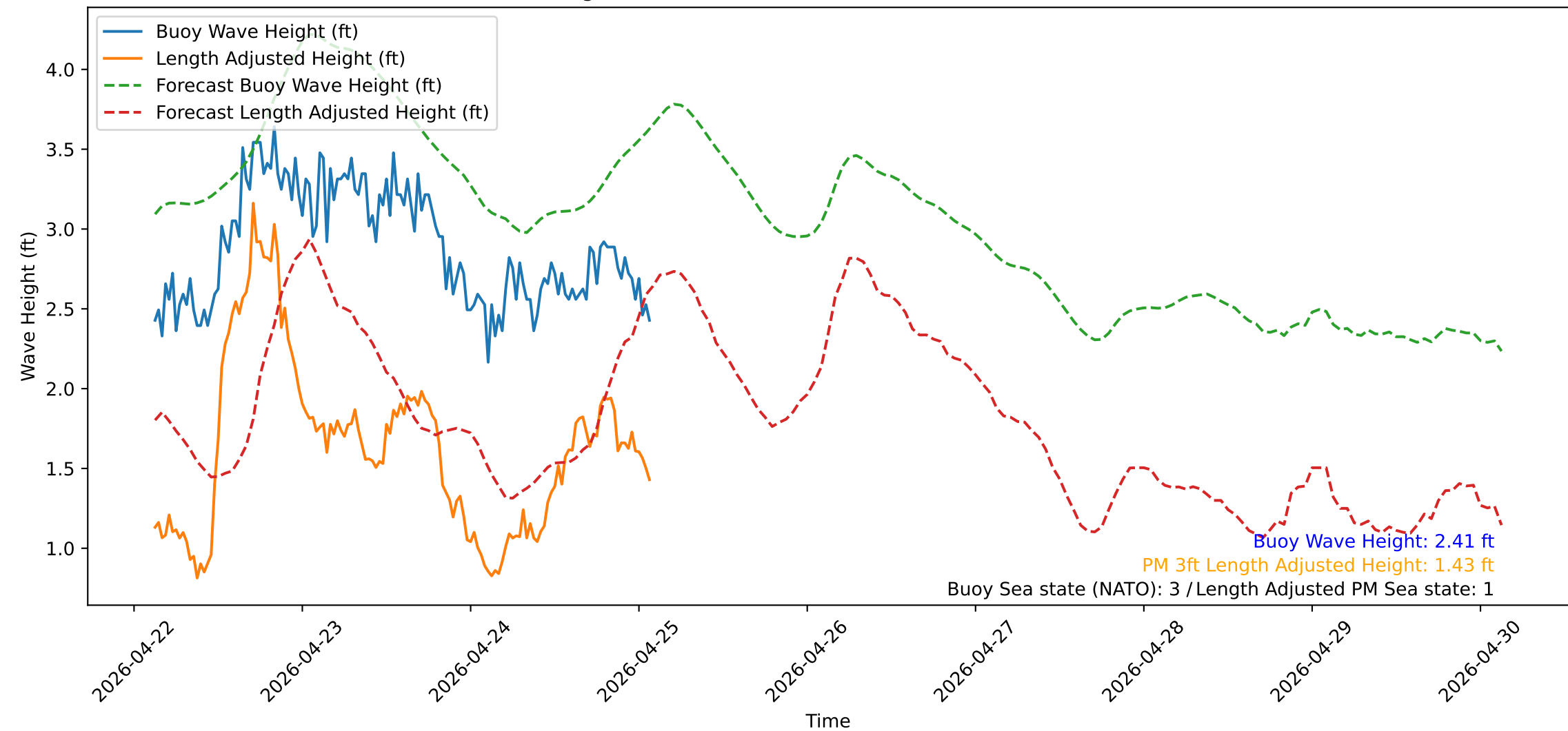
Wave Heights over Time for Red Beach at 2026-04-25 02:30:51
