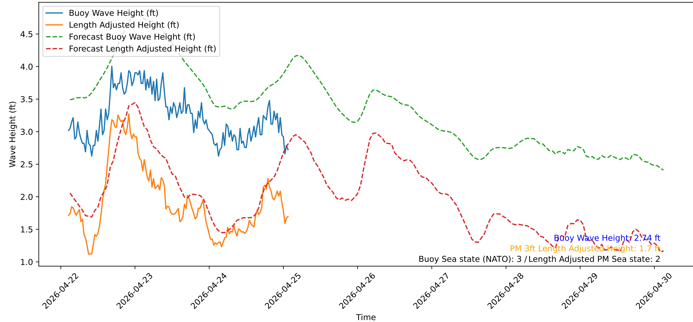
Wave Heights over Time for Green Beach at 2026-04-25 02:31:12
