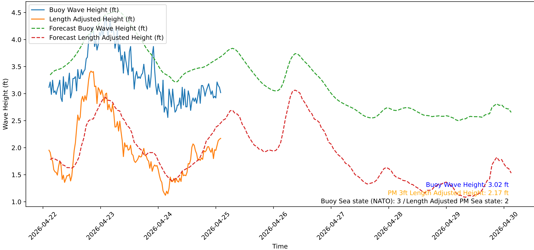
Wave Heights over Time for Oceanside Harbor at 2026-04-25 02:30:32
