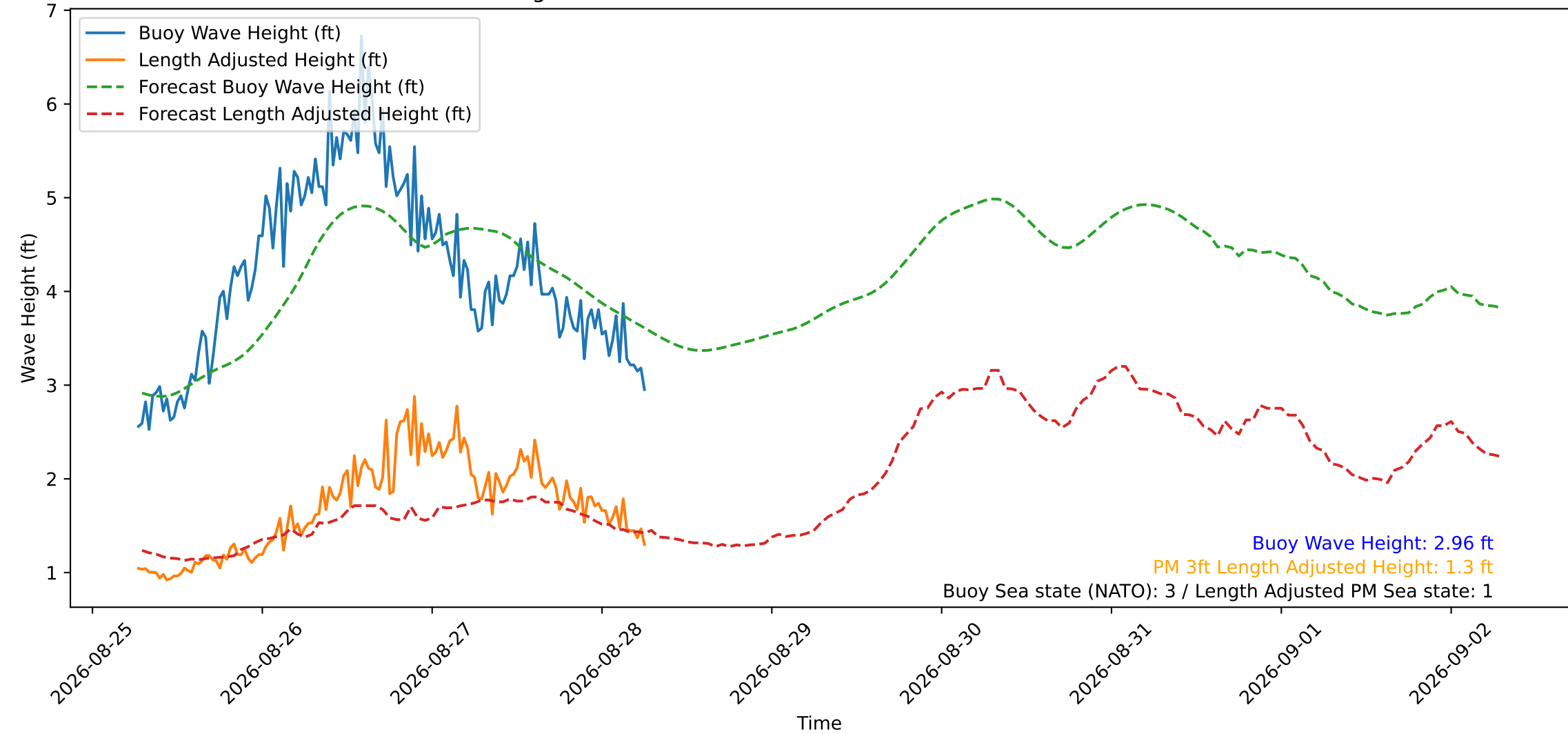
Wave Heights over Time for Oceanside Harbor at 2026-08-28 06:40:29
