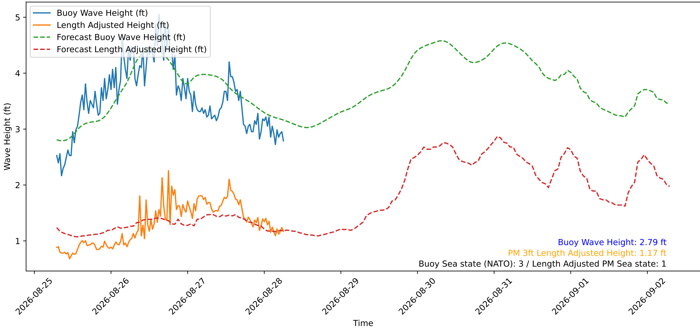
Wave Heights over Time for Red Beach at 2026-08-28 06:40:50
