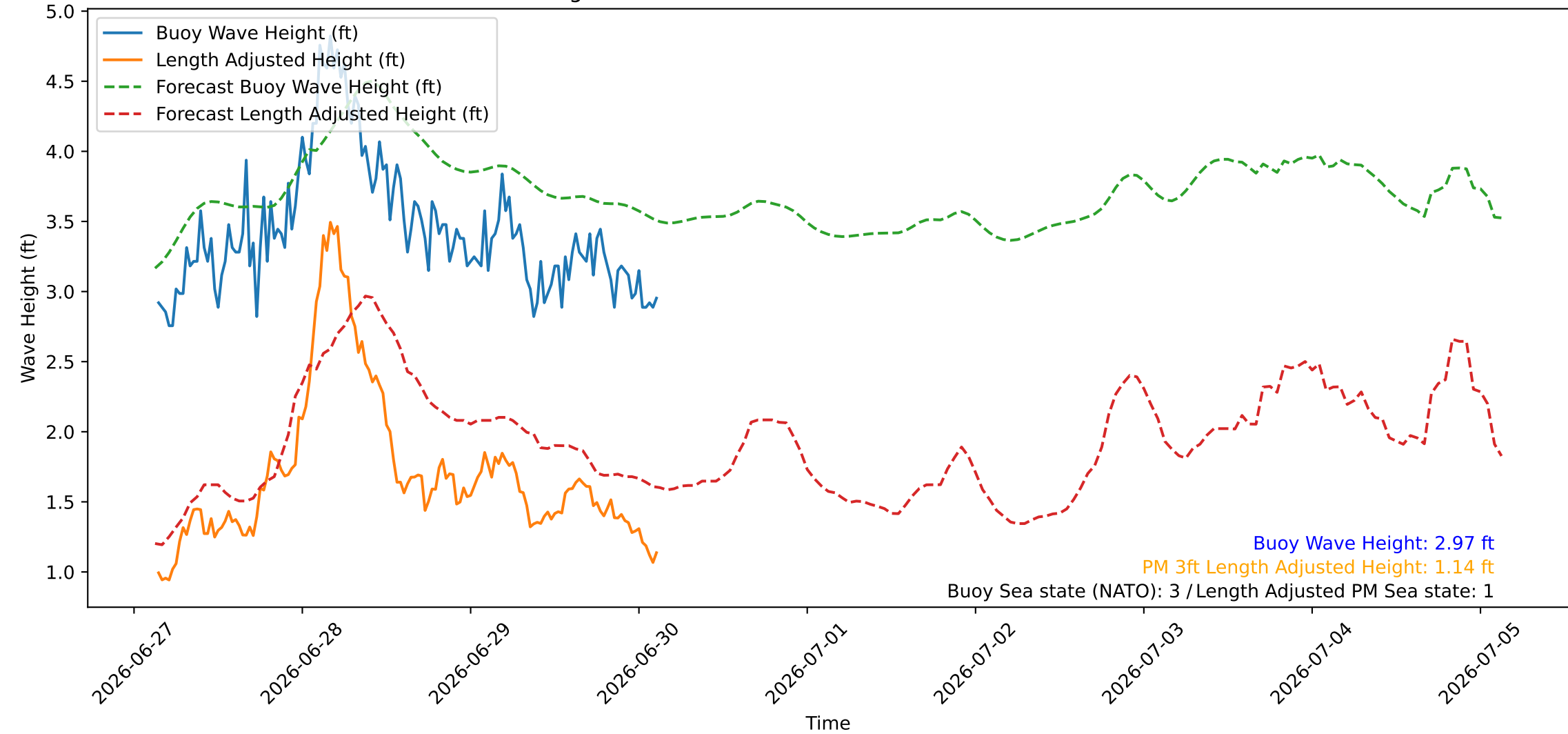
Wave Heights over Time for Green Beach at 2026-06-30 03:21:09
