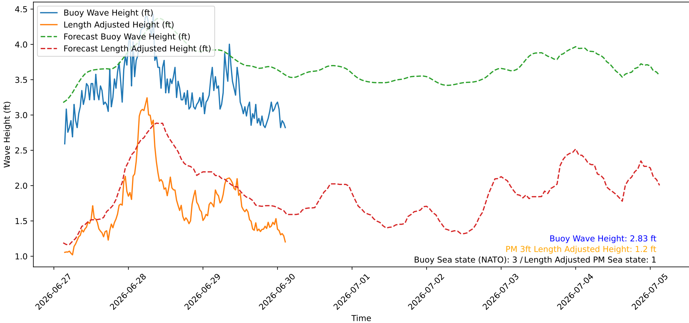
Wave Heights over Time for Oceanside Harbor at 2026-06-30 03:20:26
