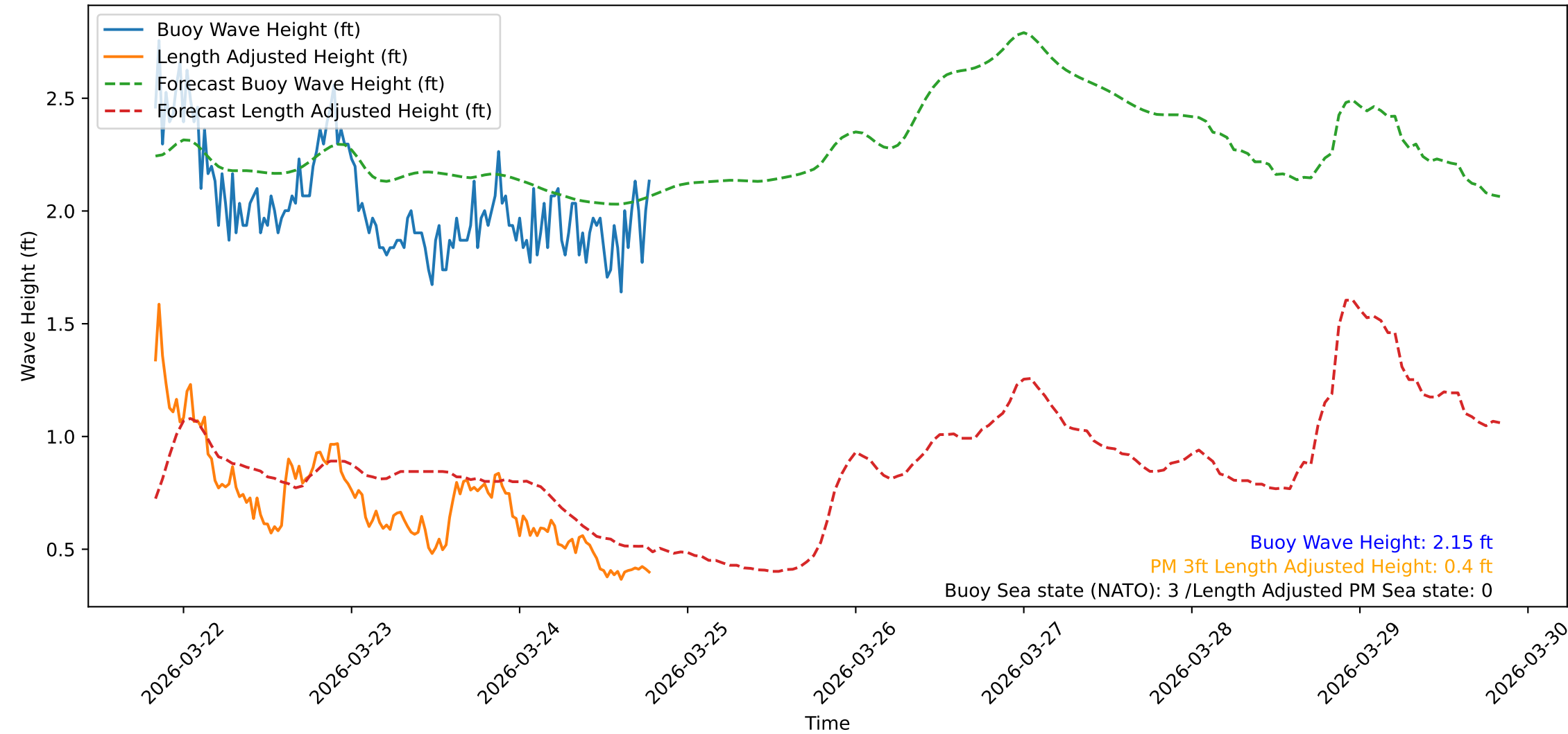
Wave Heights over Time for Red Beach at 2026-03-24 19:30:48
