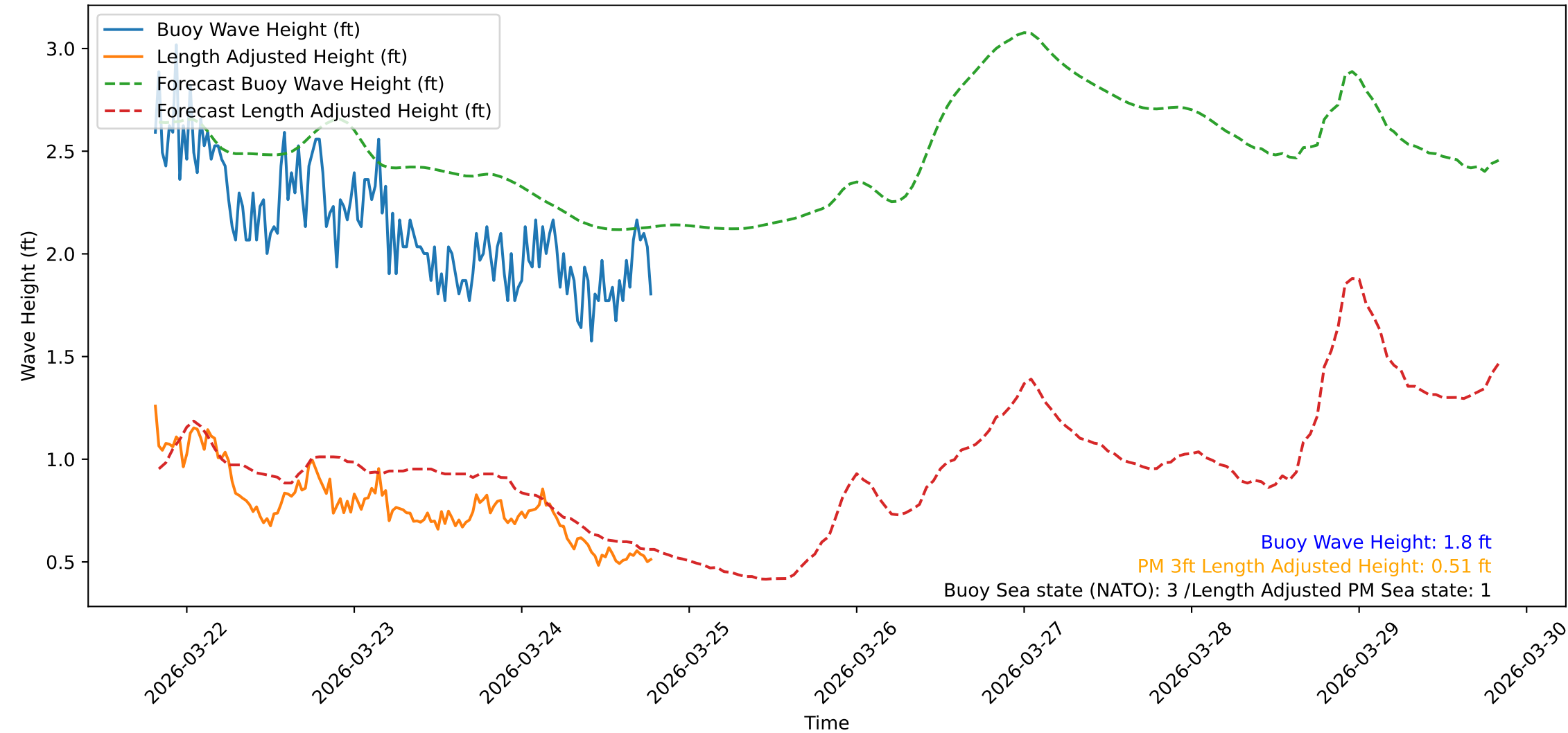
Wave Heights over Time for Oceanside Harbor at 2026-03-24 19:30:32
