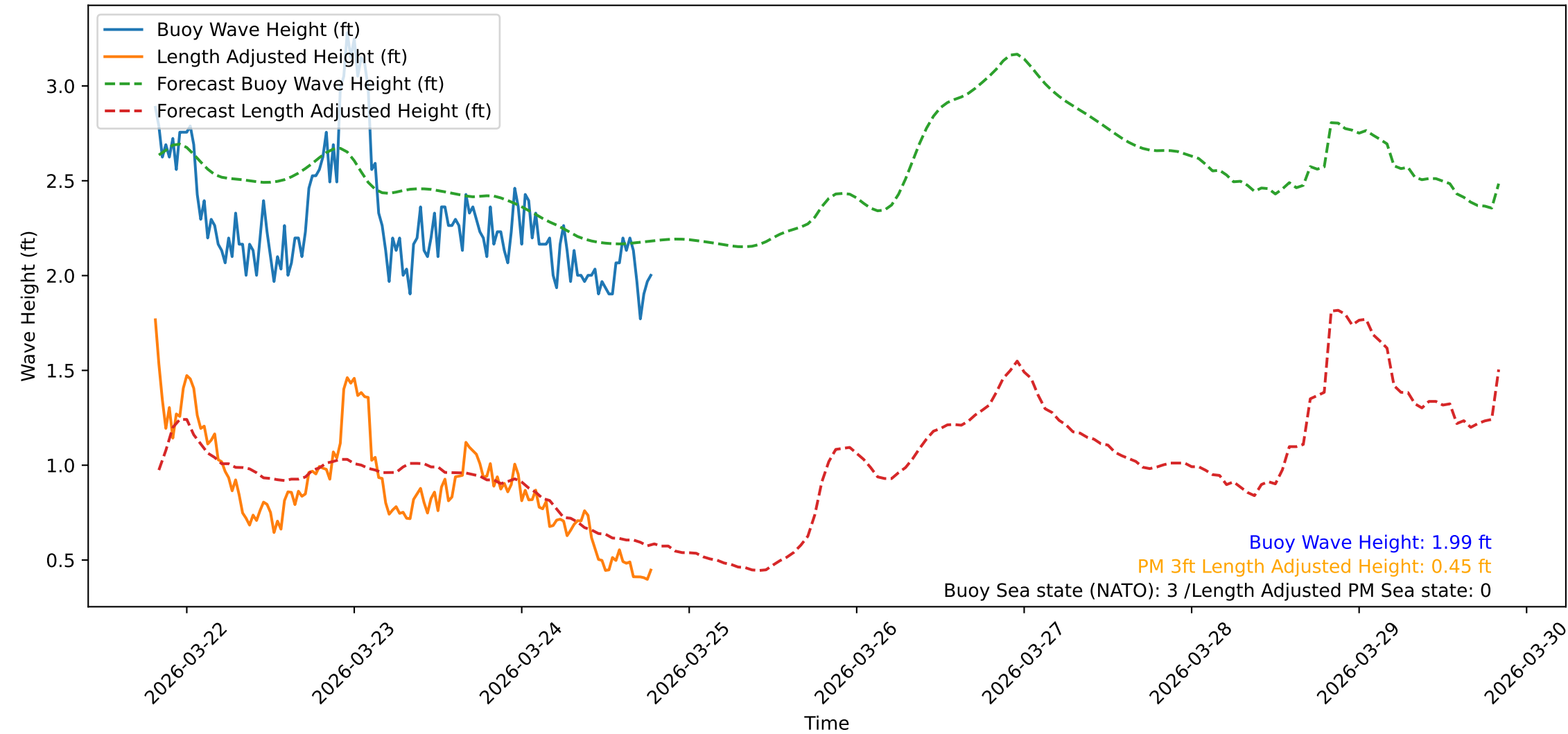
Wave Heights over Time for Green Beach at 2026-03-24 19:31:10
