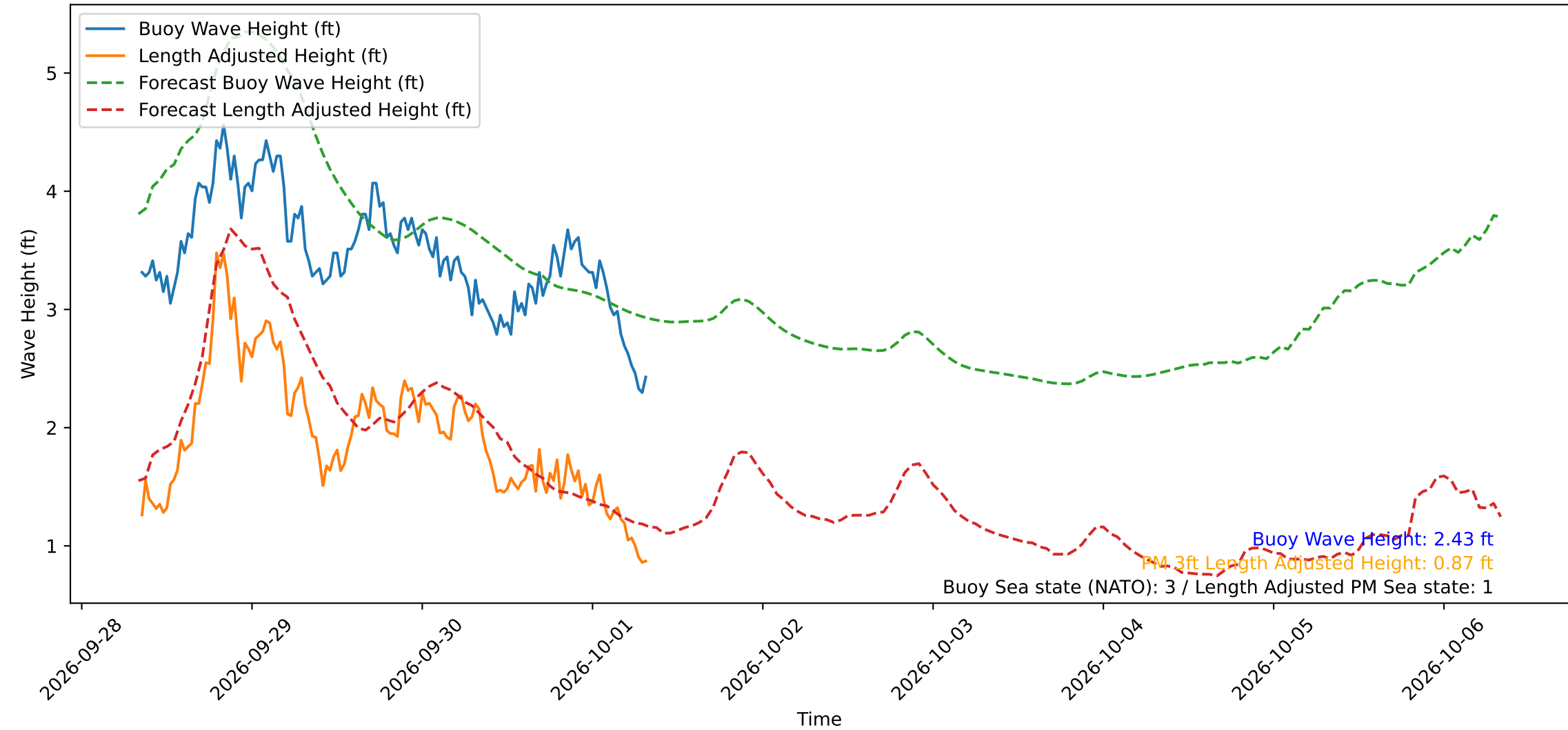
Wave Heights over Time for Green Beach at 2026-10-01 08:21:15
