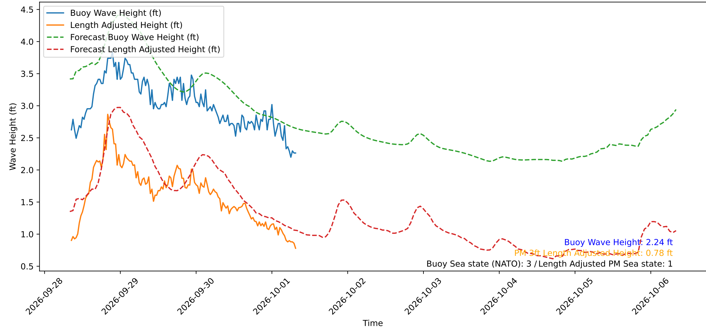
Wave Heights over Time for Red Beach at 2026-10-01 08:20:51
