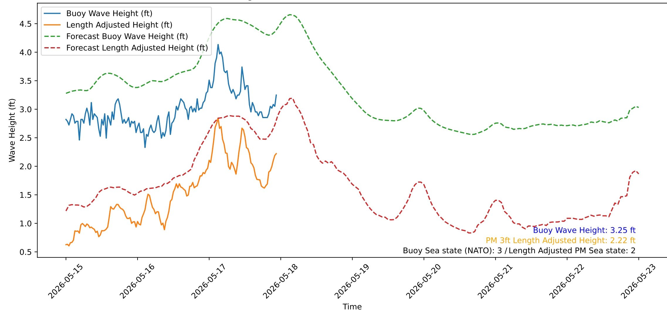
Wave Heights over Time for Red Beach at 2026-05-17 23:30:51
