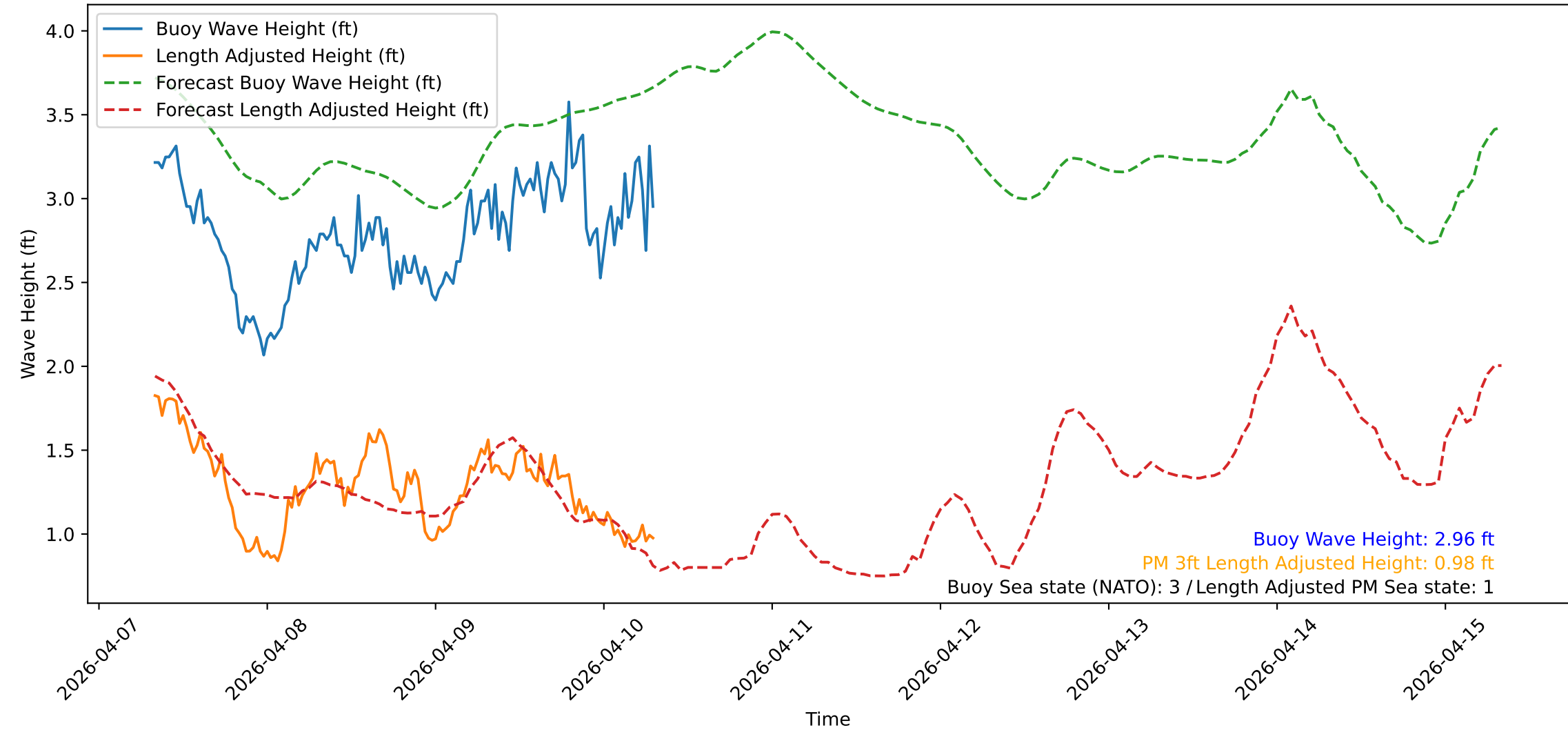
Wave Heights over Time for Red Beach at 2026-04-10 07:50:52
