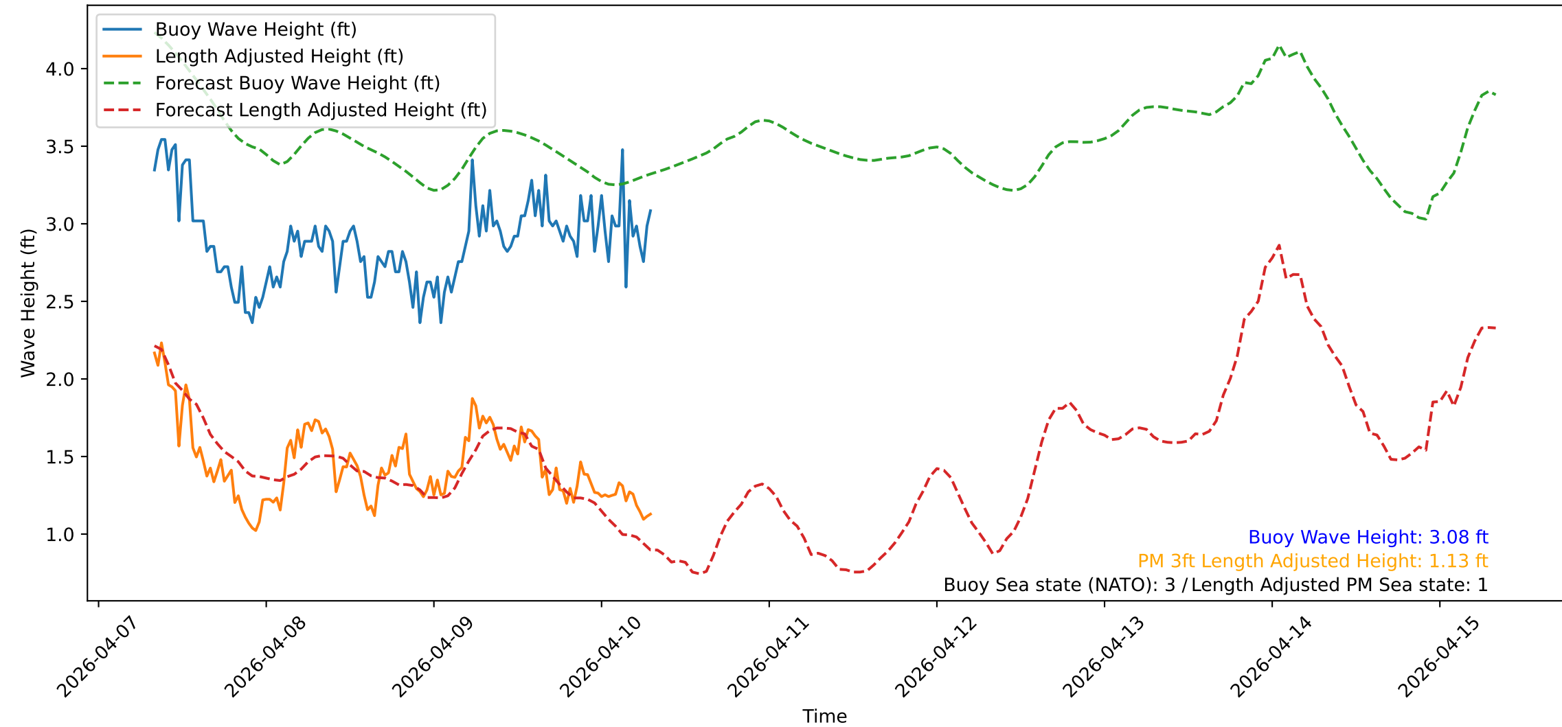
Wave Heights over Time for Green Beach at 2026-04-10 07:51:14
