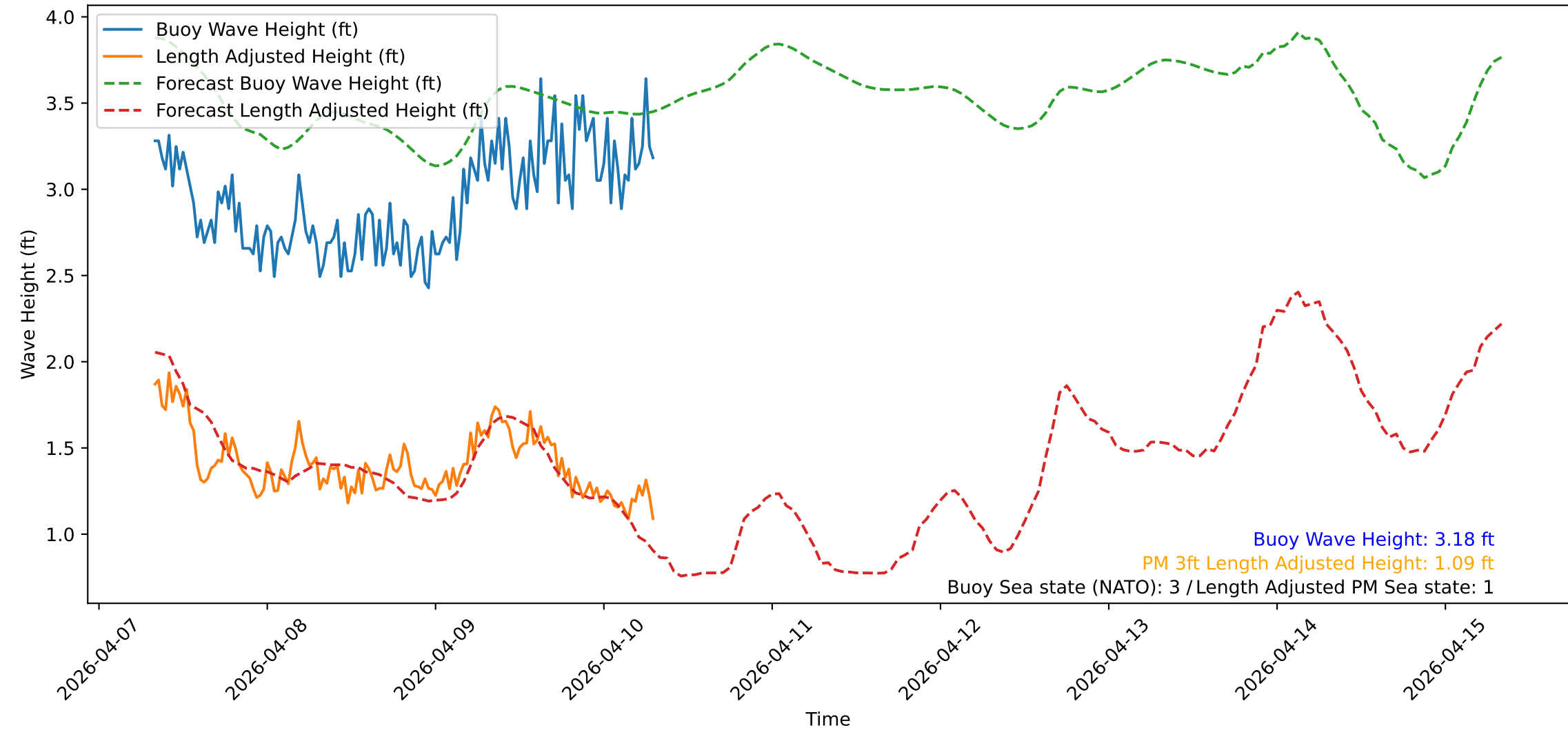
Wave Heights over Time for Oceanside Harbor at 2026-04-10 07:50:31
