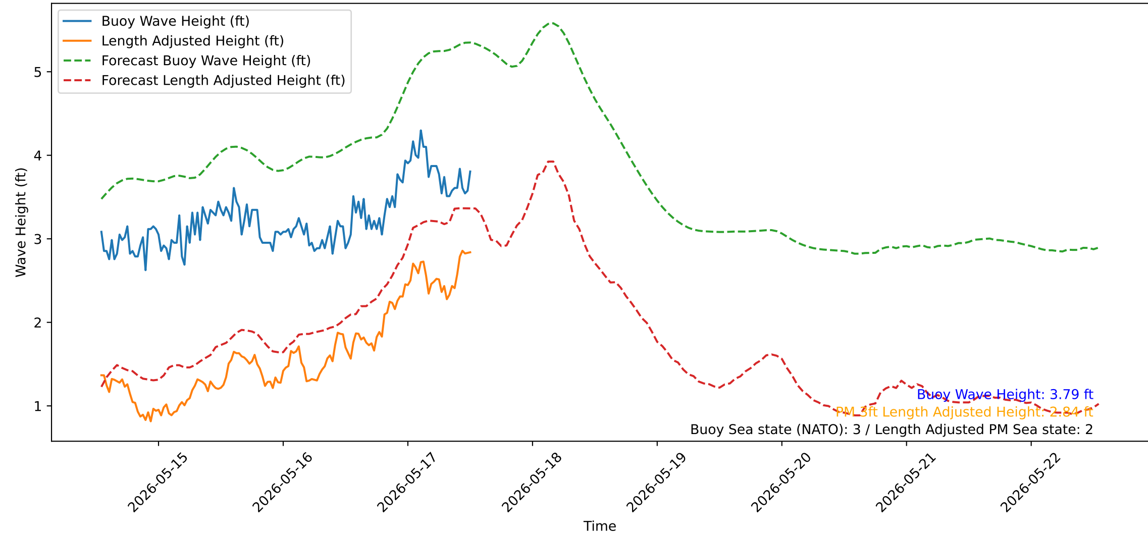
Wave Heights over Time for Oceanside Harbor at 2026-05-17 13:00:31
