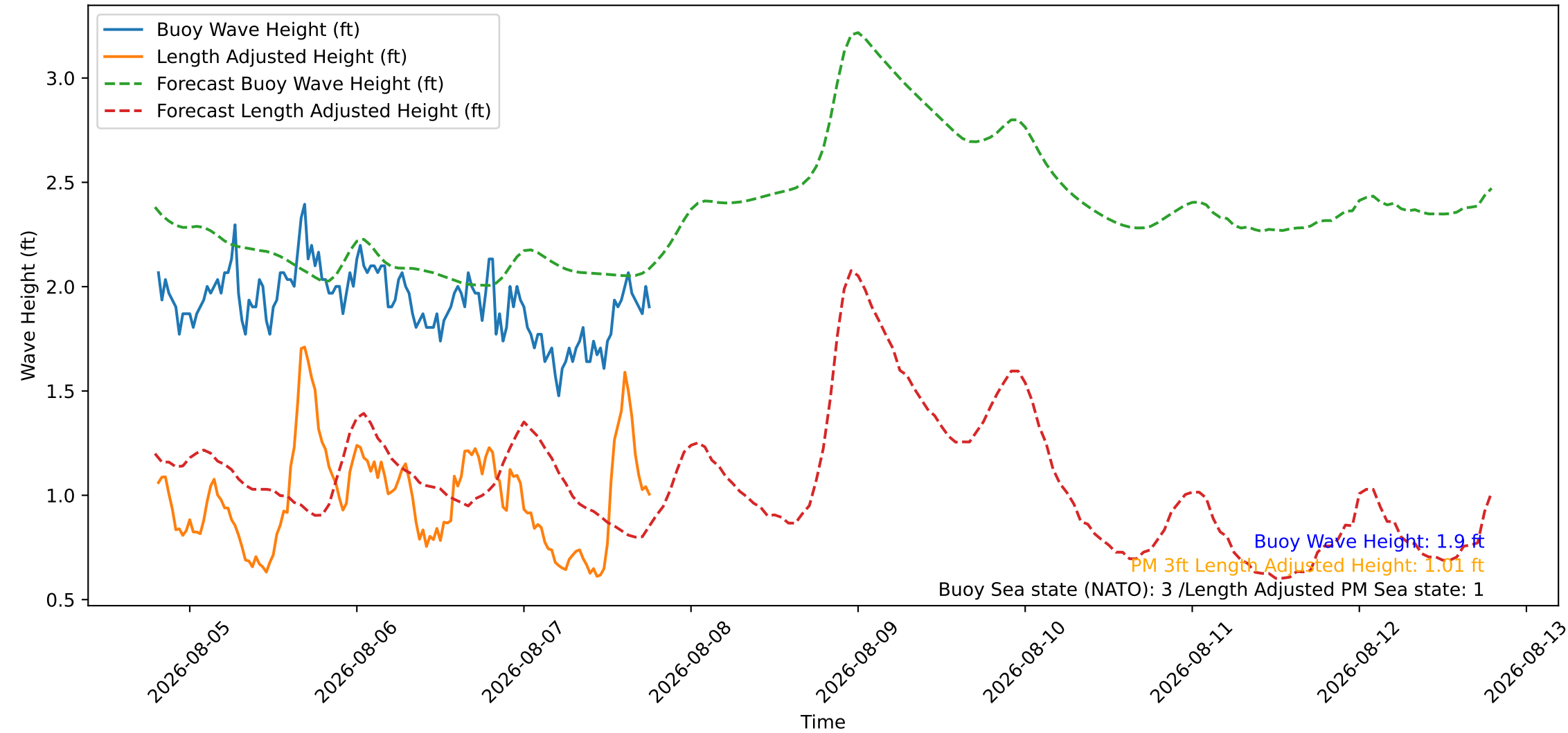
Wave Heights over Time for Red Beach at 2026-08-07 19:20:47
