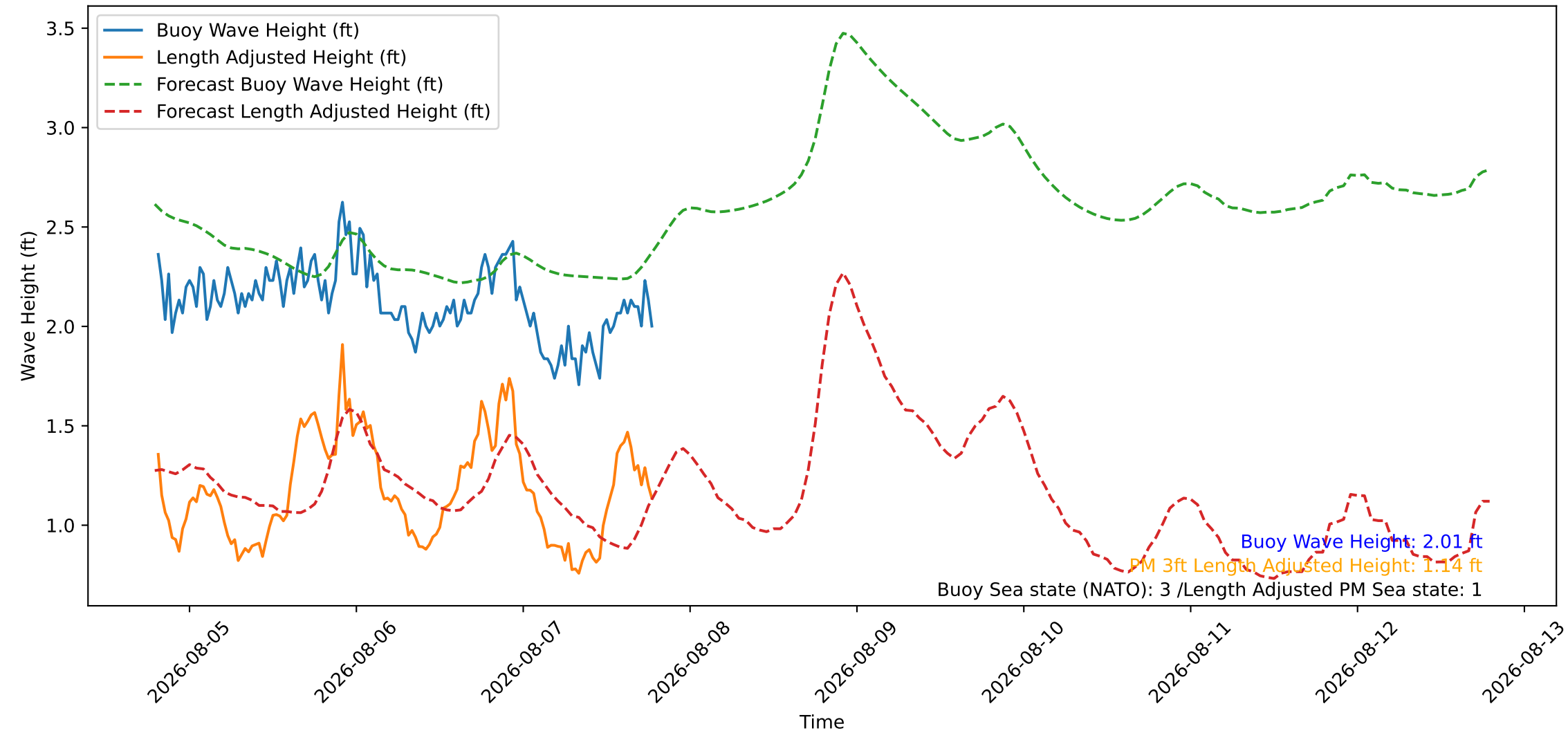
Wave Heights over Time for Green Beach at 2026-08-07 19:21:10
