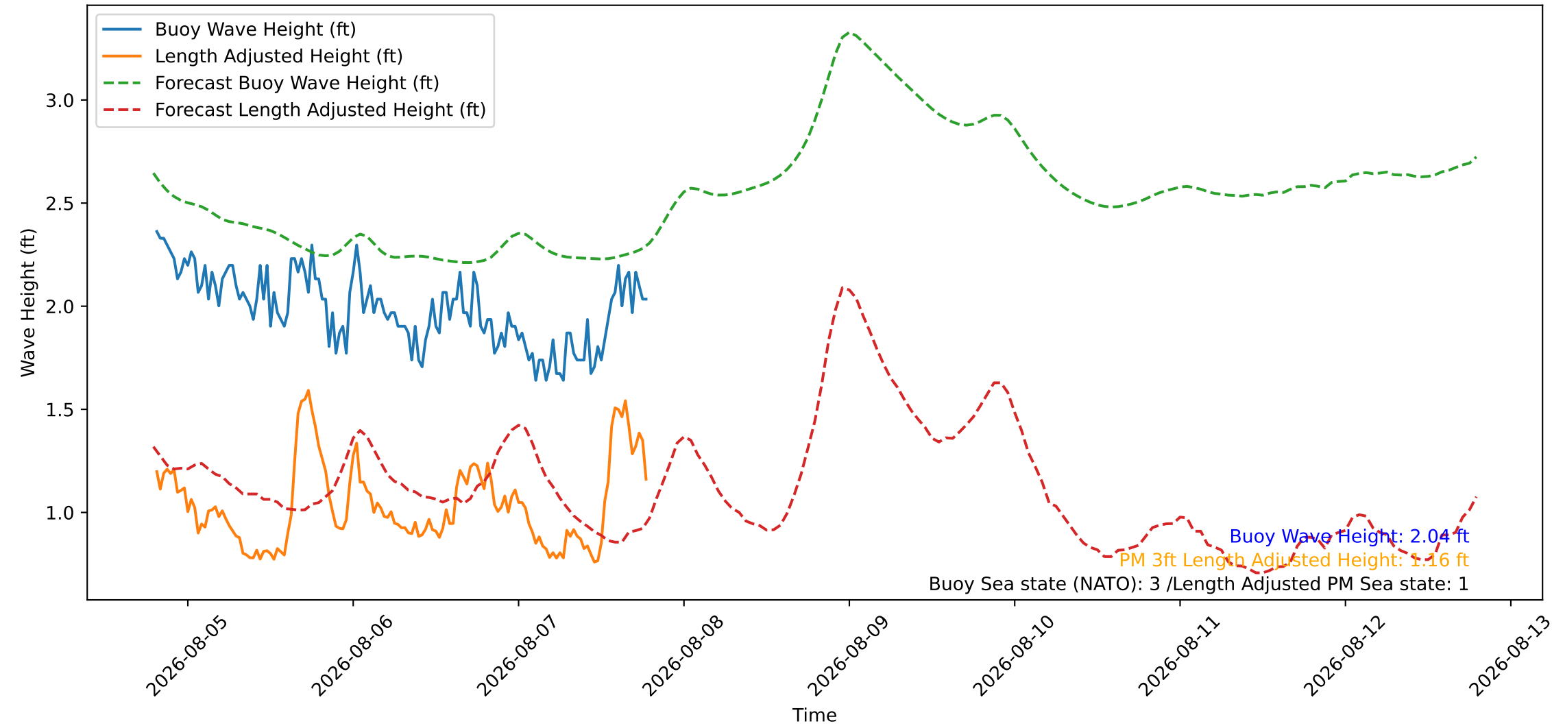
Wave Heights over Time for Oceanside Harbor at 2026-08-07 19:20:26
