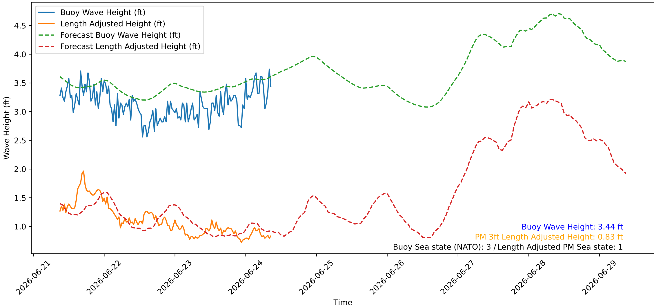
Wave Heights over Time for Oceanside Harbor at 2026-06-24 09:10:26
