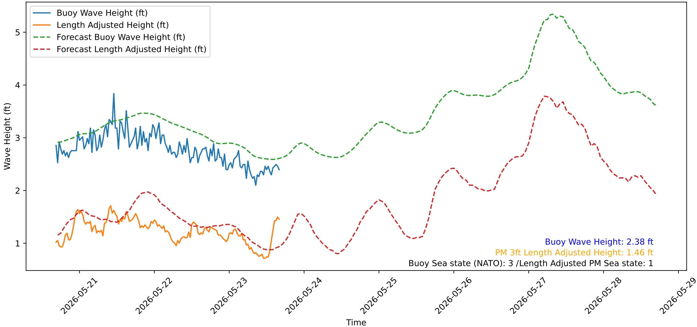
Wave Heights over Time for Oceanside Harbor at 2026-05-23 16:40:32
