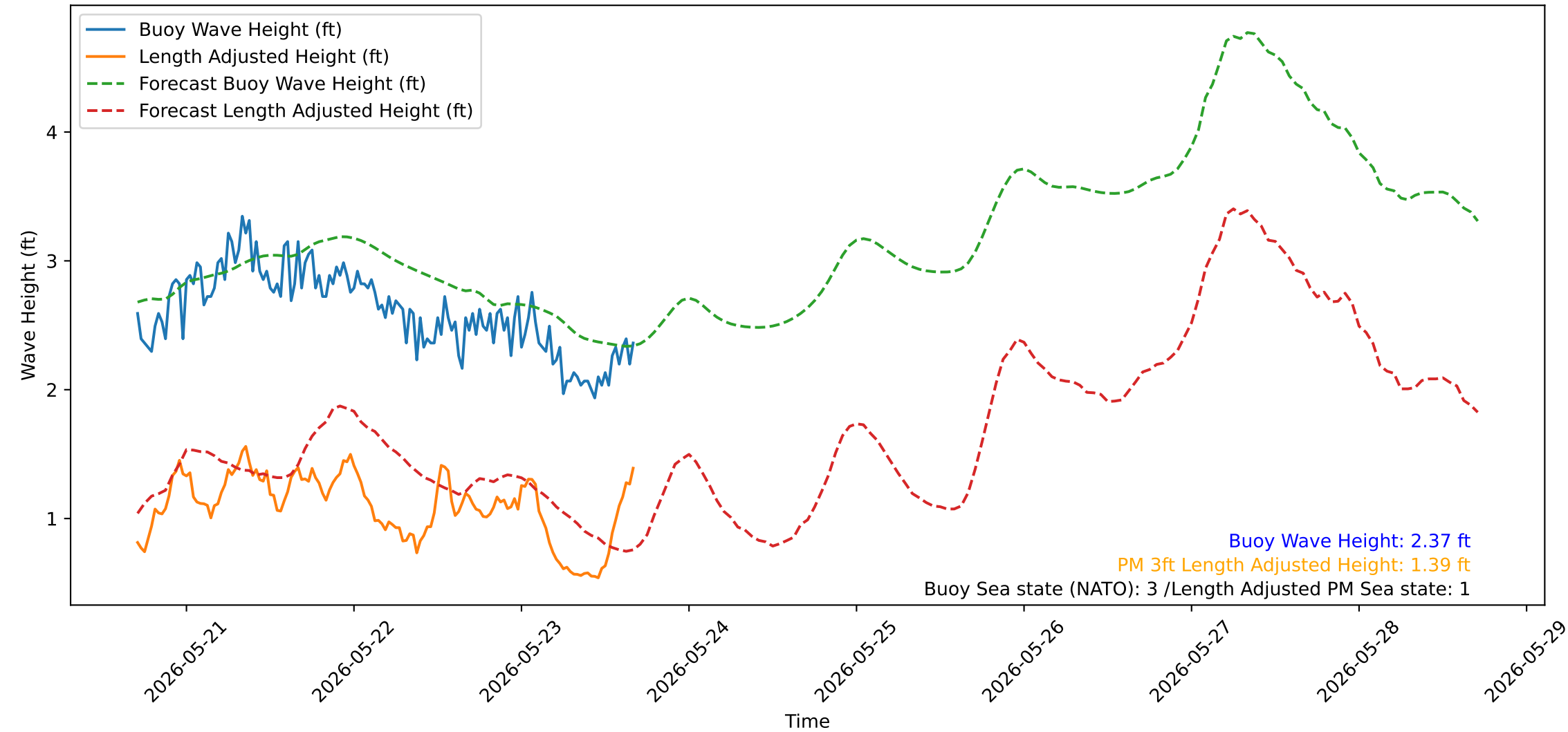
Wave Heights over Time for Red Beach at 2026-05-23 16:40:51
