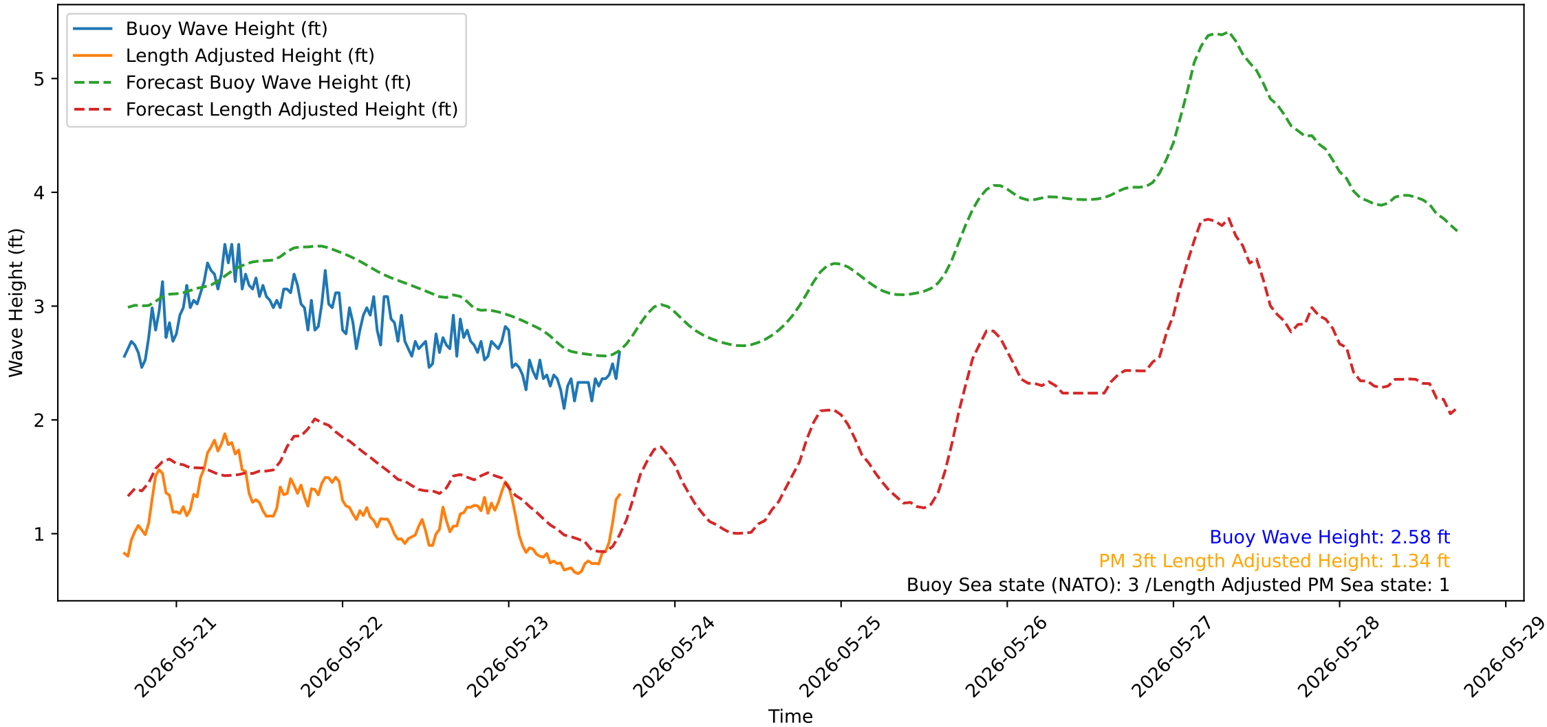
Wave Heights over Time for Green Beach at 2026-05-23 16:41:14
