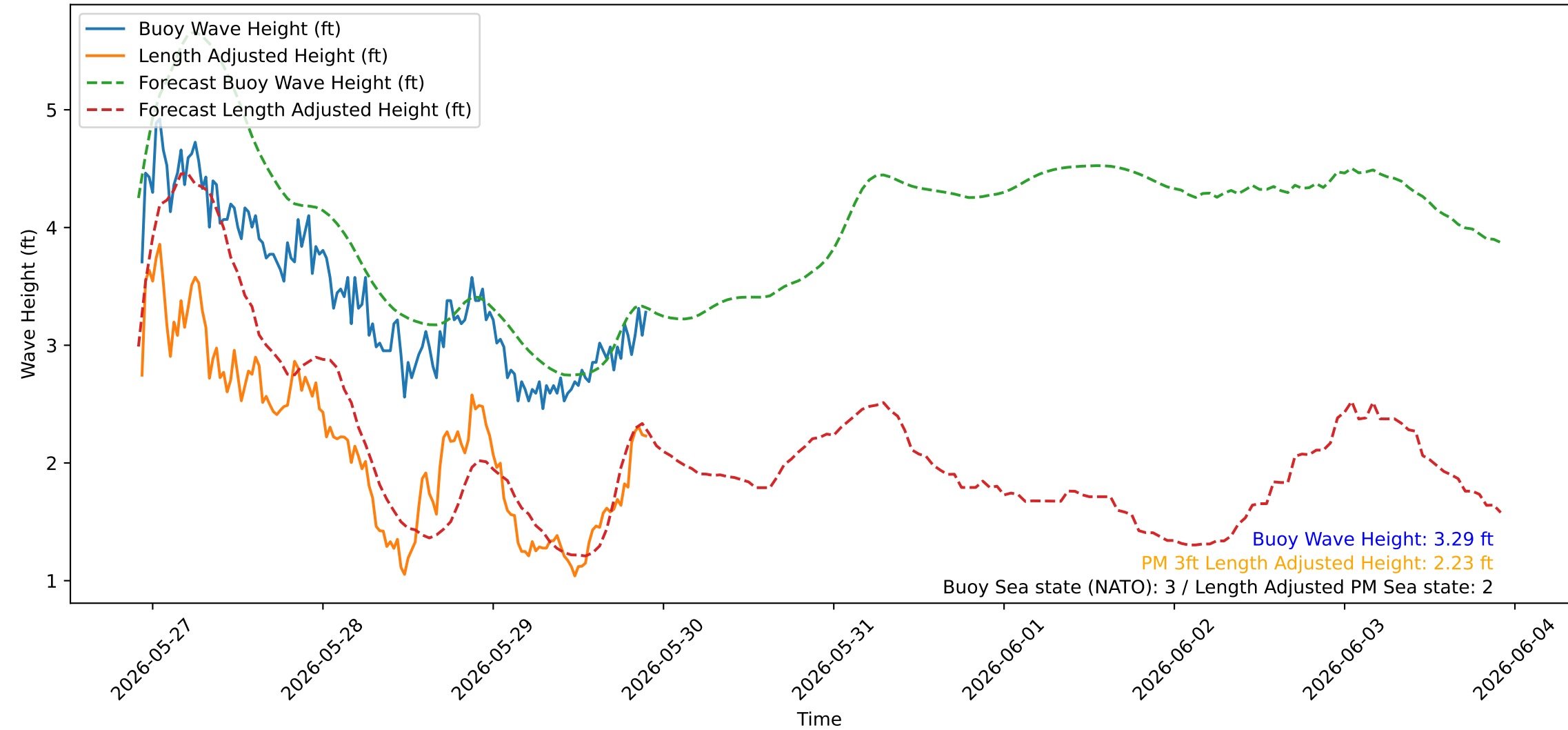
Wave Heights over Time for Green Beach at 2026-05-29 22:21:05
