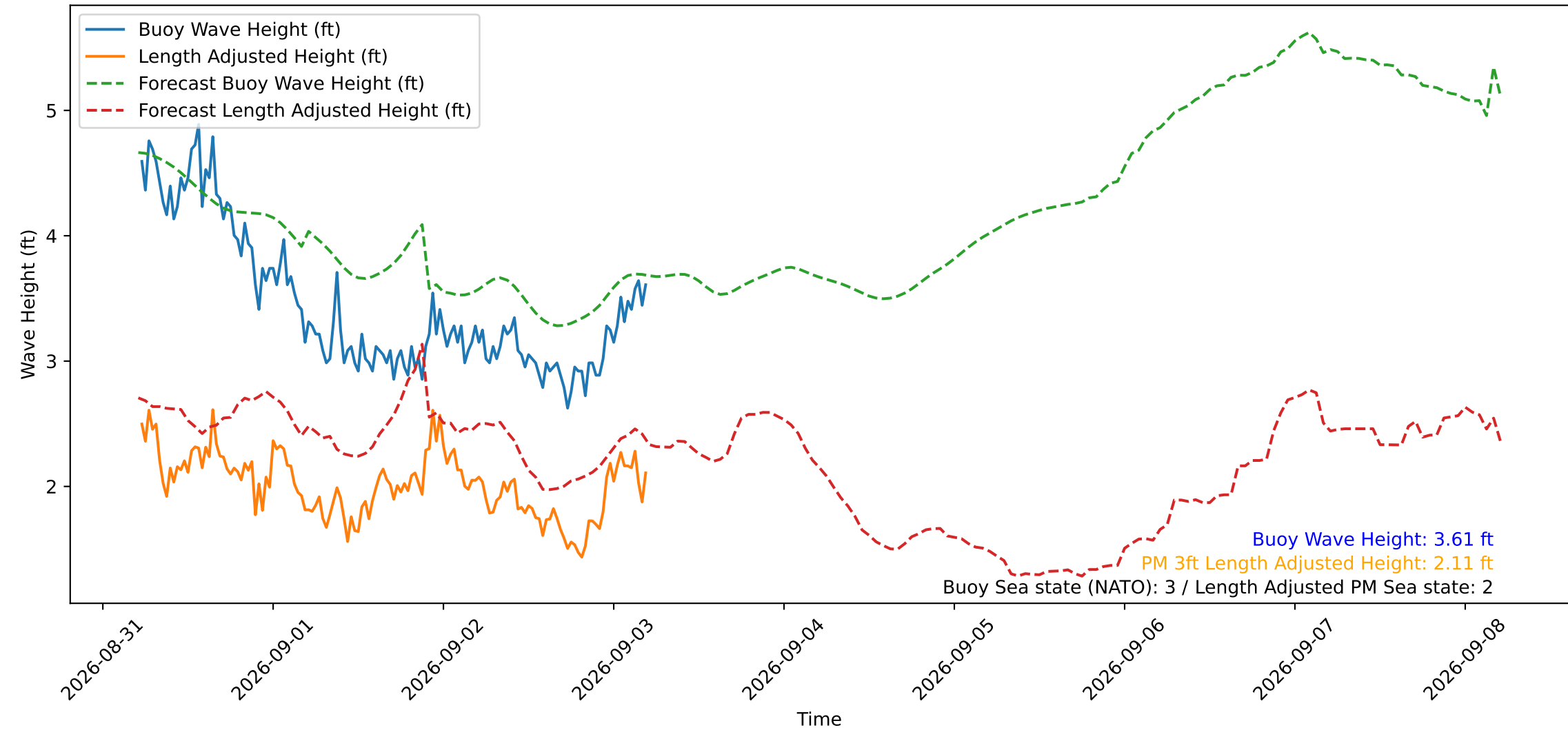
Wave Heights over Time for Oceanside Harbor at 2026-09-03 05:20:29
