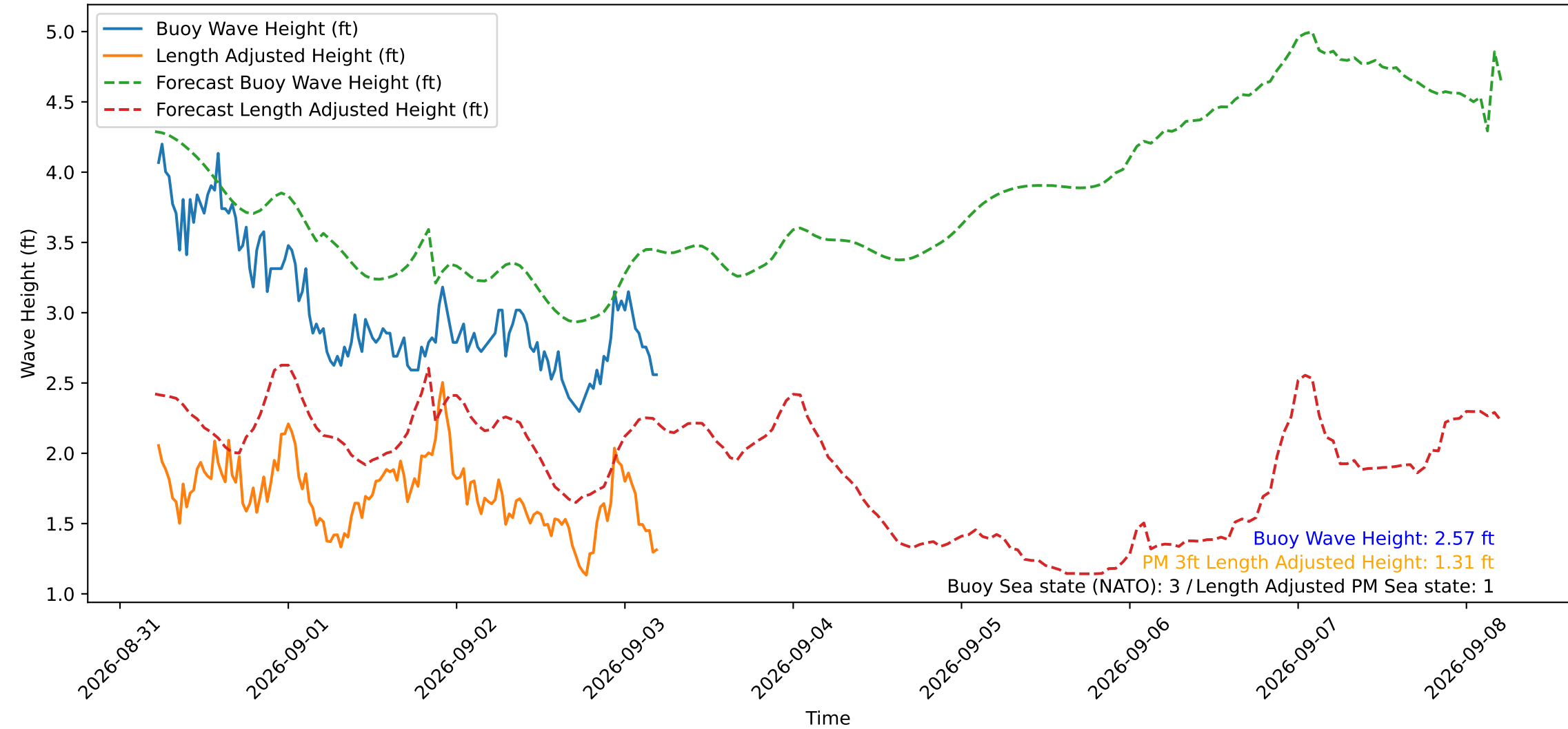
Wave Heights over Time for Red Beach at 2026-09-03 05:20:50
