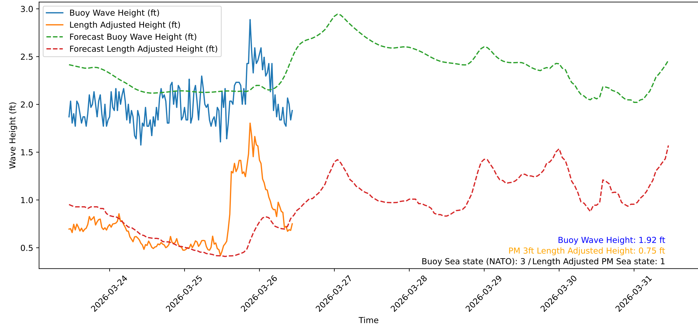
Wave Heights over Time for Oceanside Harbor at 2026-03-26 11:10:32
