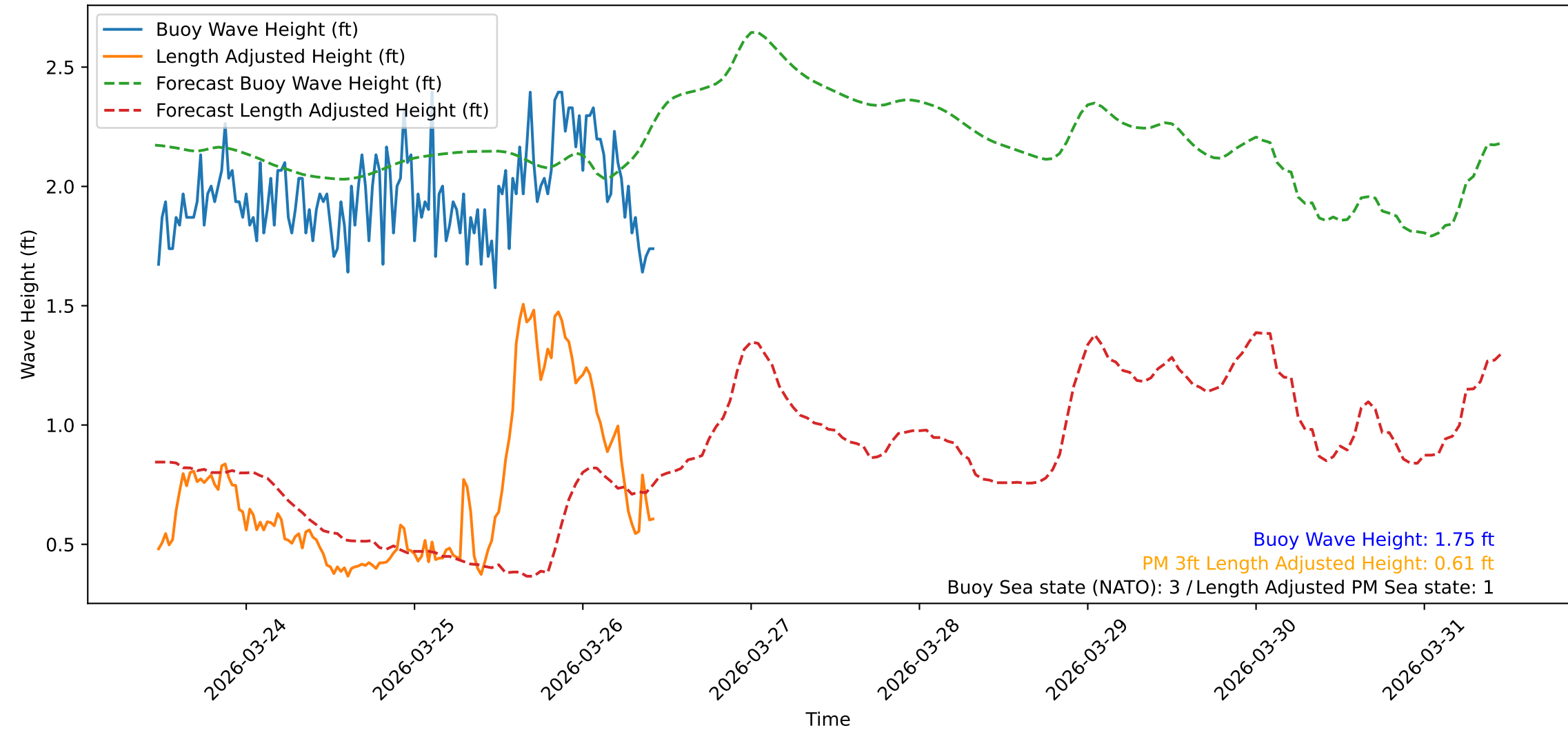
Wave Heights over Time for Red Beach at 2026-03-26 11:10:48
