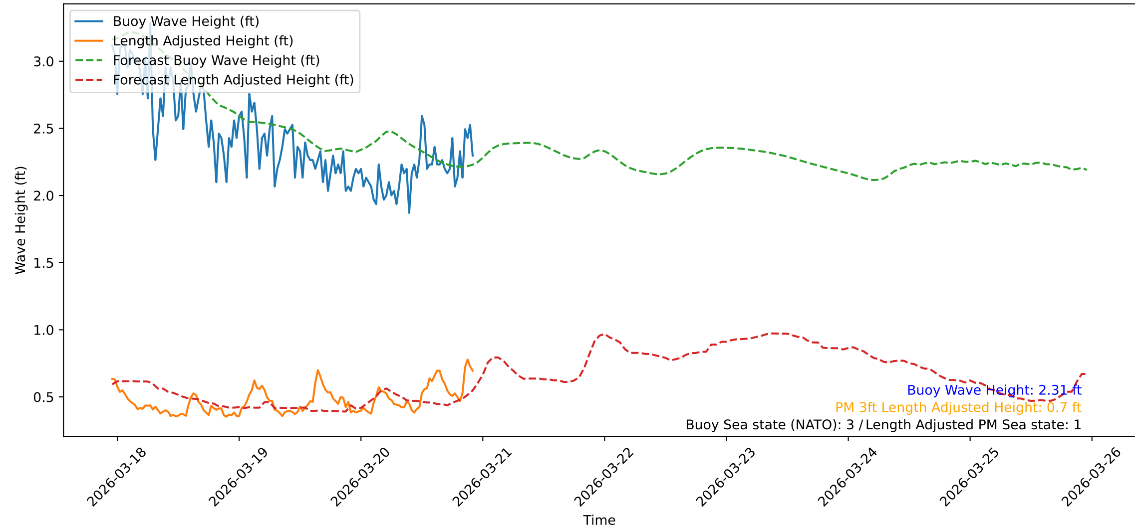
Wave Heights over Time for Red Beach at 2026-03-20 22:40:49
