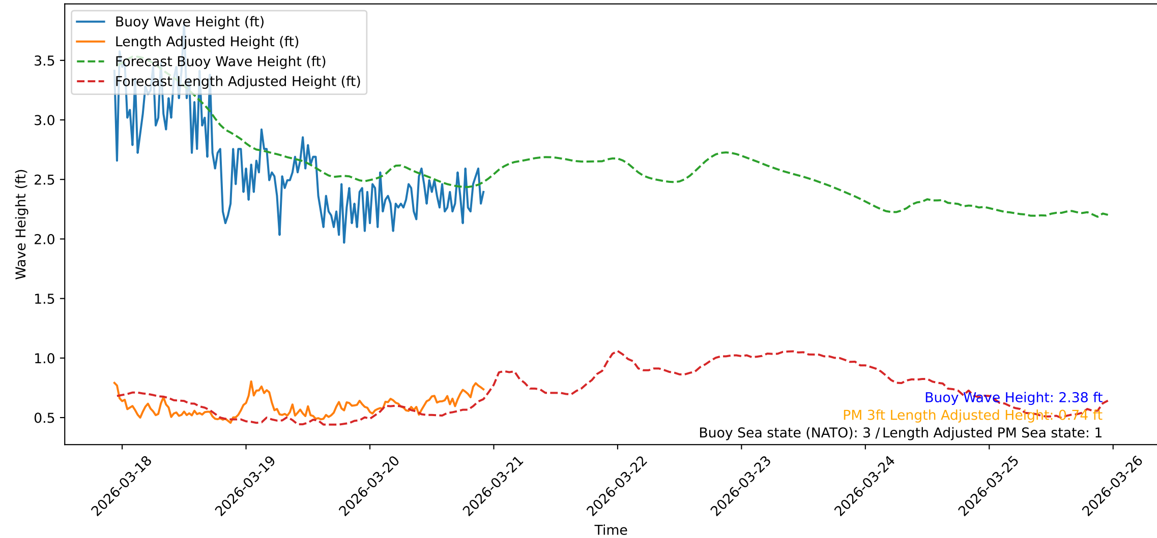
Wave Heights over Time for Oceanside Harbor at 2026-03-20 22:40:32
