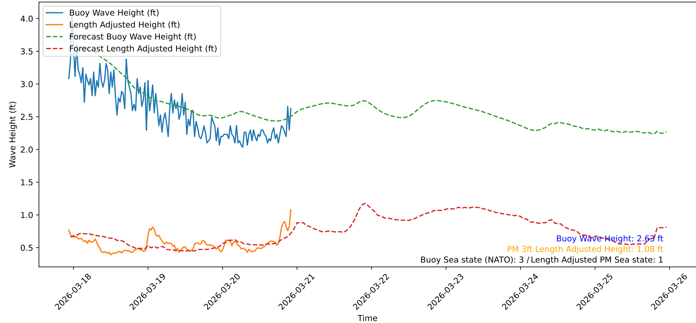
Wave Heights over Time for Green Beach at 2026-03-20 22:41:12
