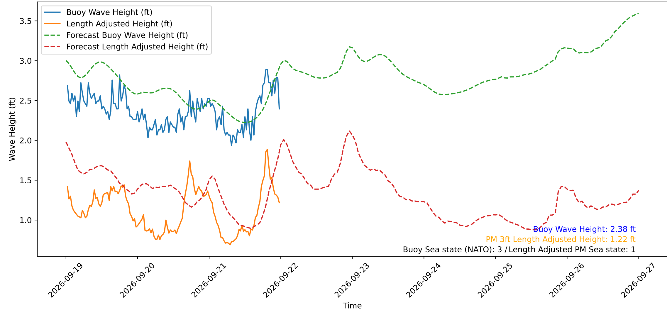
Wave Heights over Time for Red Beach at 2026-09-22 00:10:49
