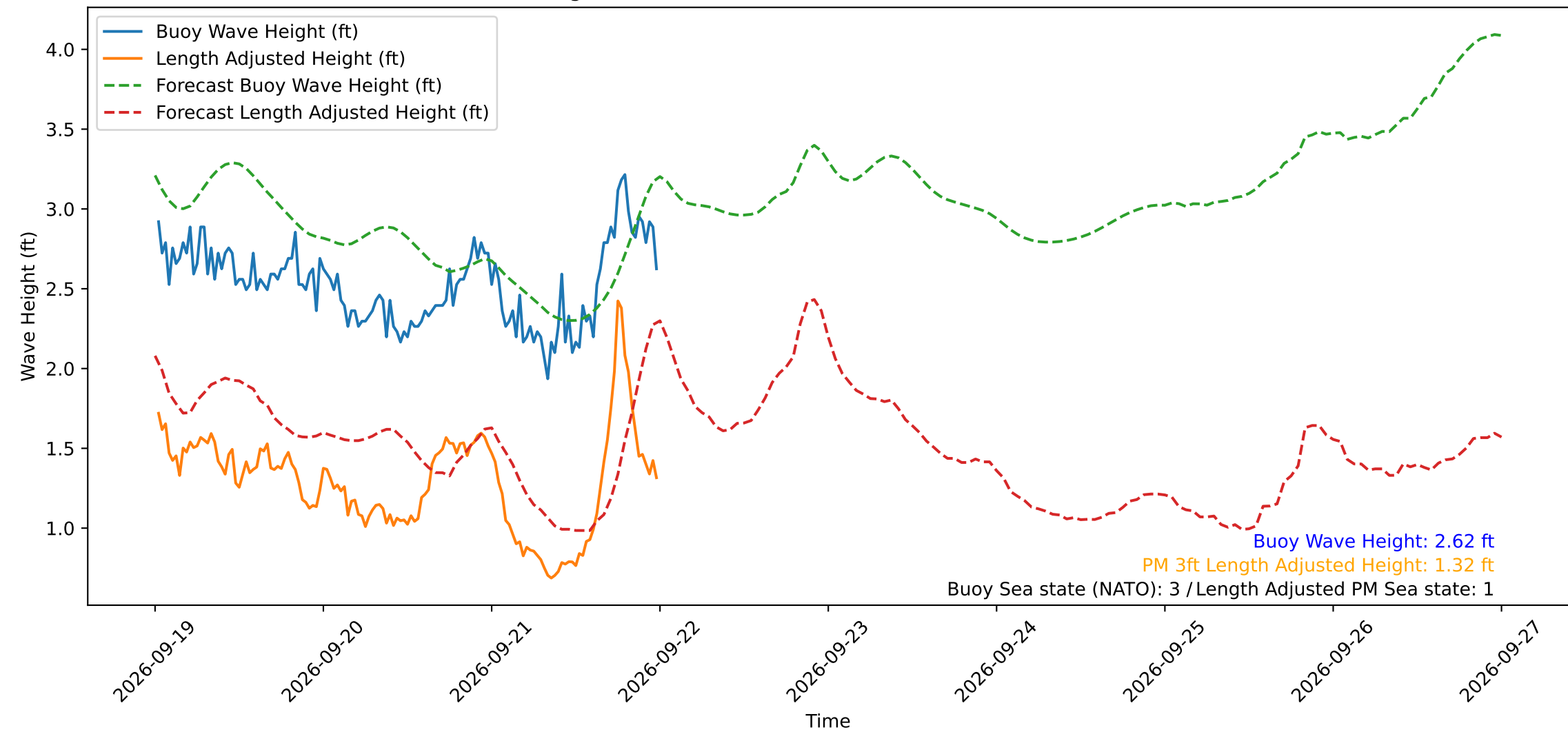
Wave Heights over Time for Green Beach at 2026-09-22 00:11:10
