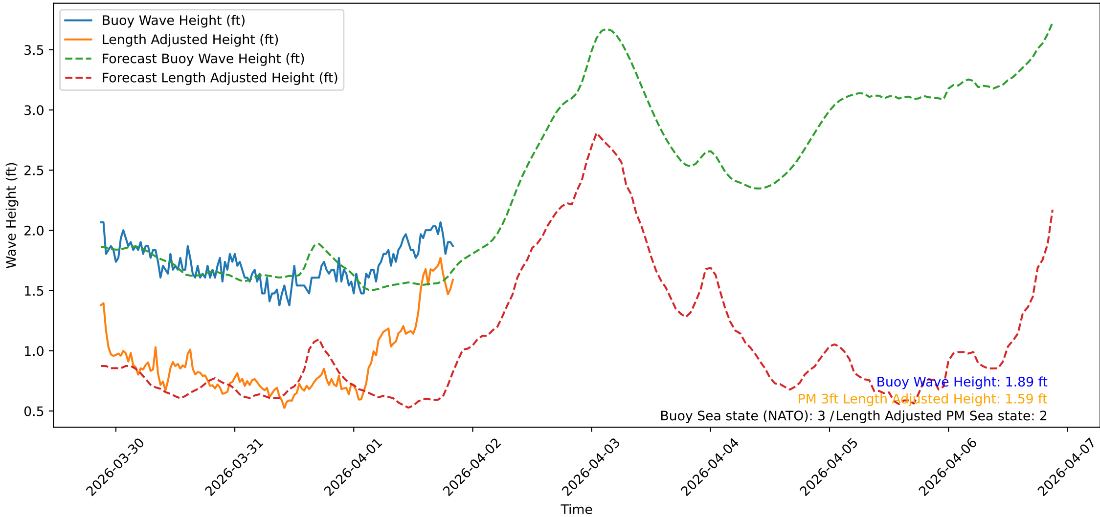
Wave Heights over Time for Red Beach at 2026-04-01 20:50:47
