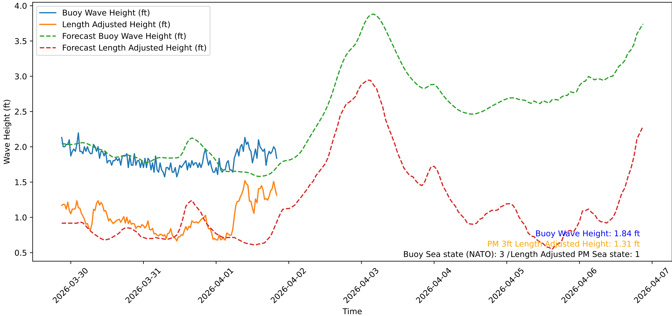
Wave Heights over Time for Oceanside Harbor at 2026-04-01 20:50:31
