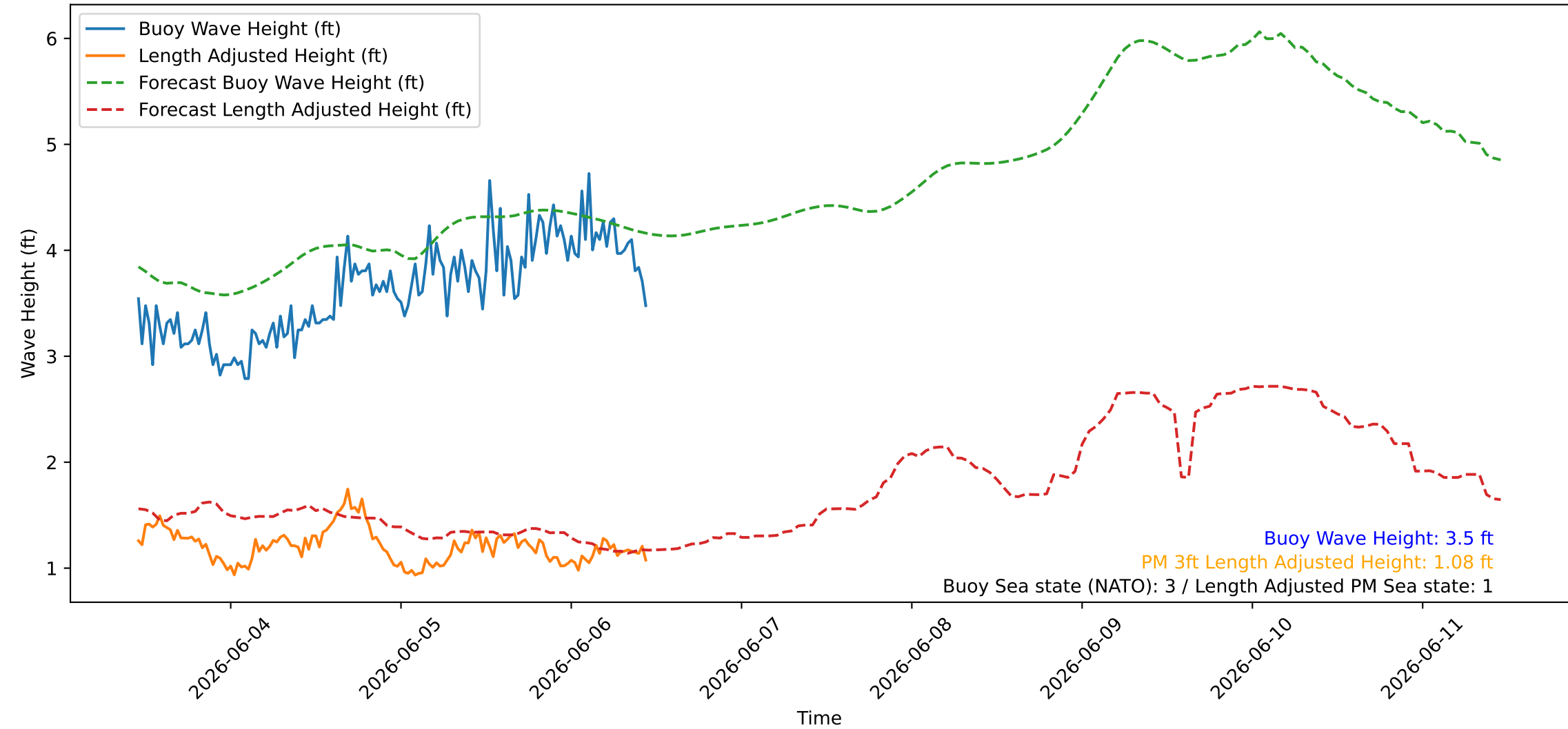
Wave Heights over Time for Green Beach at 2026-06-06 11:11:09
