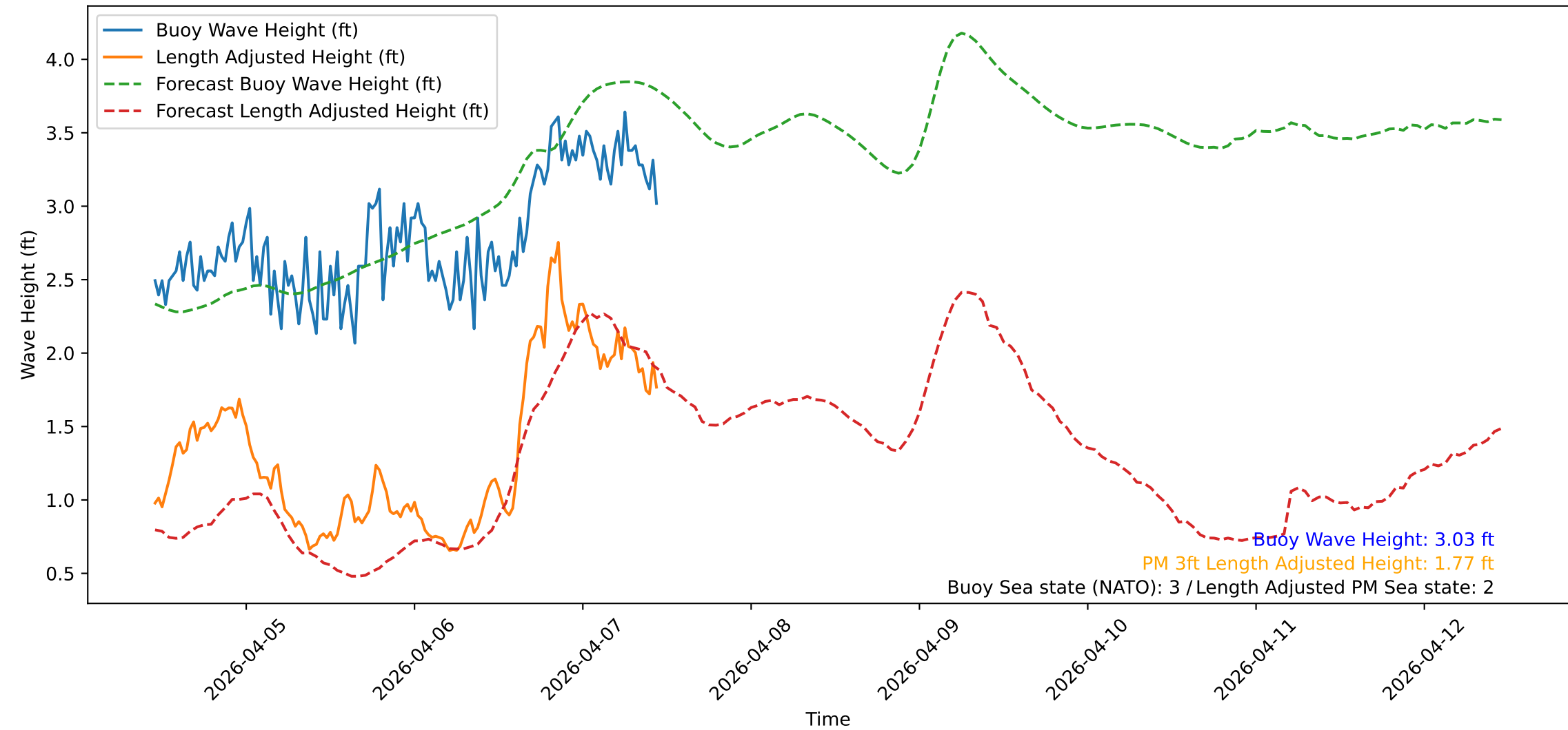
Wave Heights over Time for Oceanside Harbor at 2026-04-07 11:10:33
