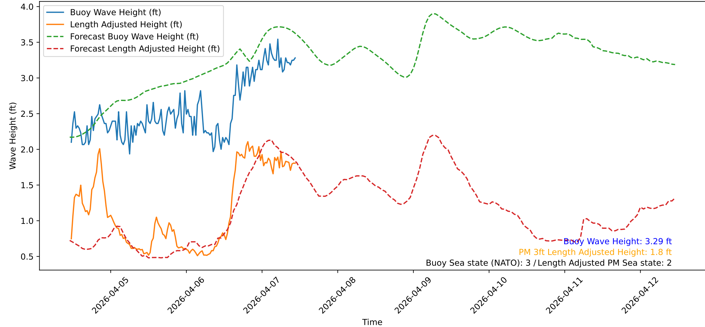
Wave Heights over Time for Red Beach at 2026-04-07 11:10:49
