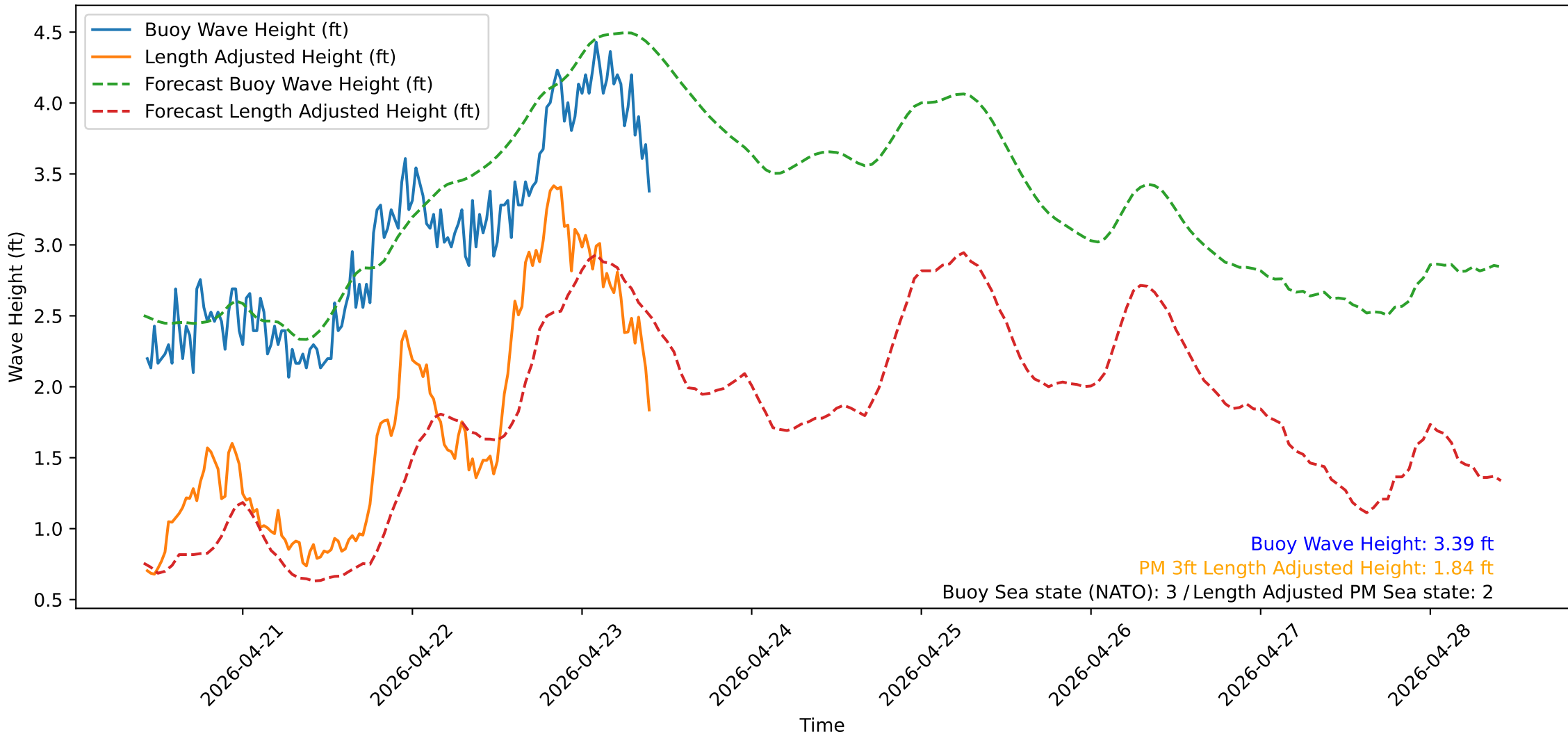
Wave Heights over Time for Oceanside Harbor at 2026-04-23 10:20:31
