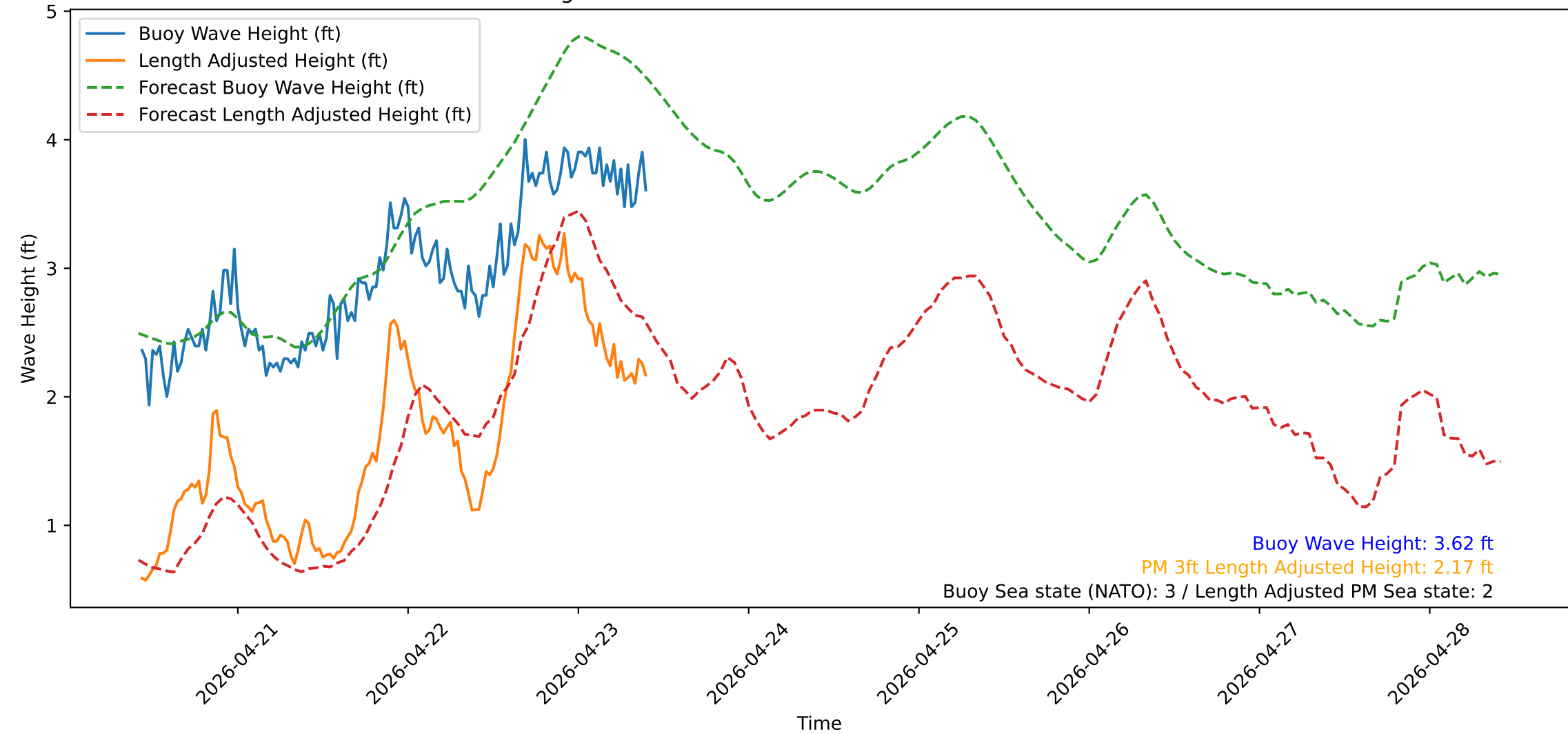
Wave Heights over Time for Green Beach at 2026-04-23 10:21:13
