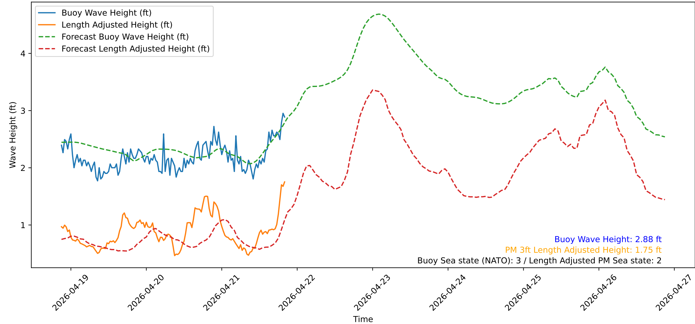
Wave Heights over Time for Red Beach at 2026-04-21 20:50:52
