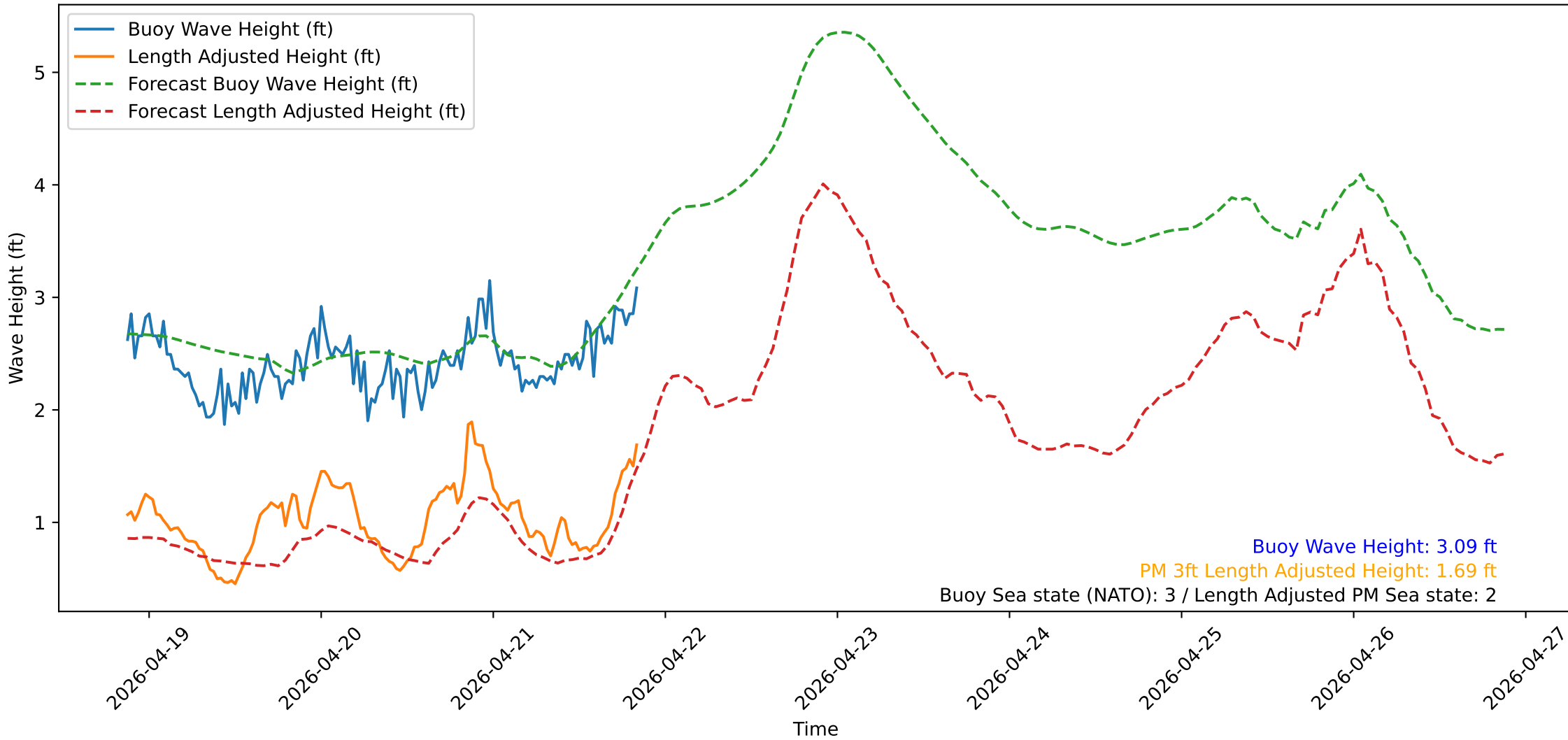
Wave Heights over Time for Green Beach at 2026-04-21 20:51:14
