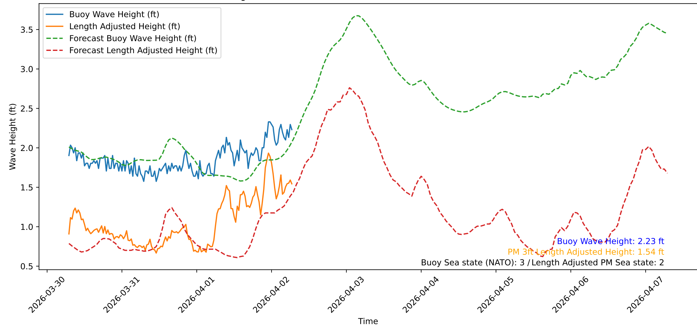
Wave Heights over Time for Oceanside Harbor at 2026-04-02 07:00:31
