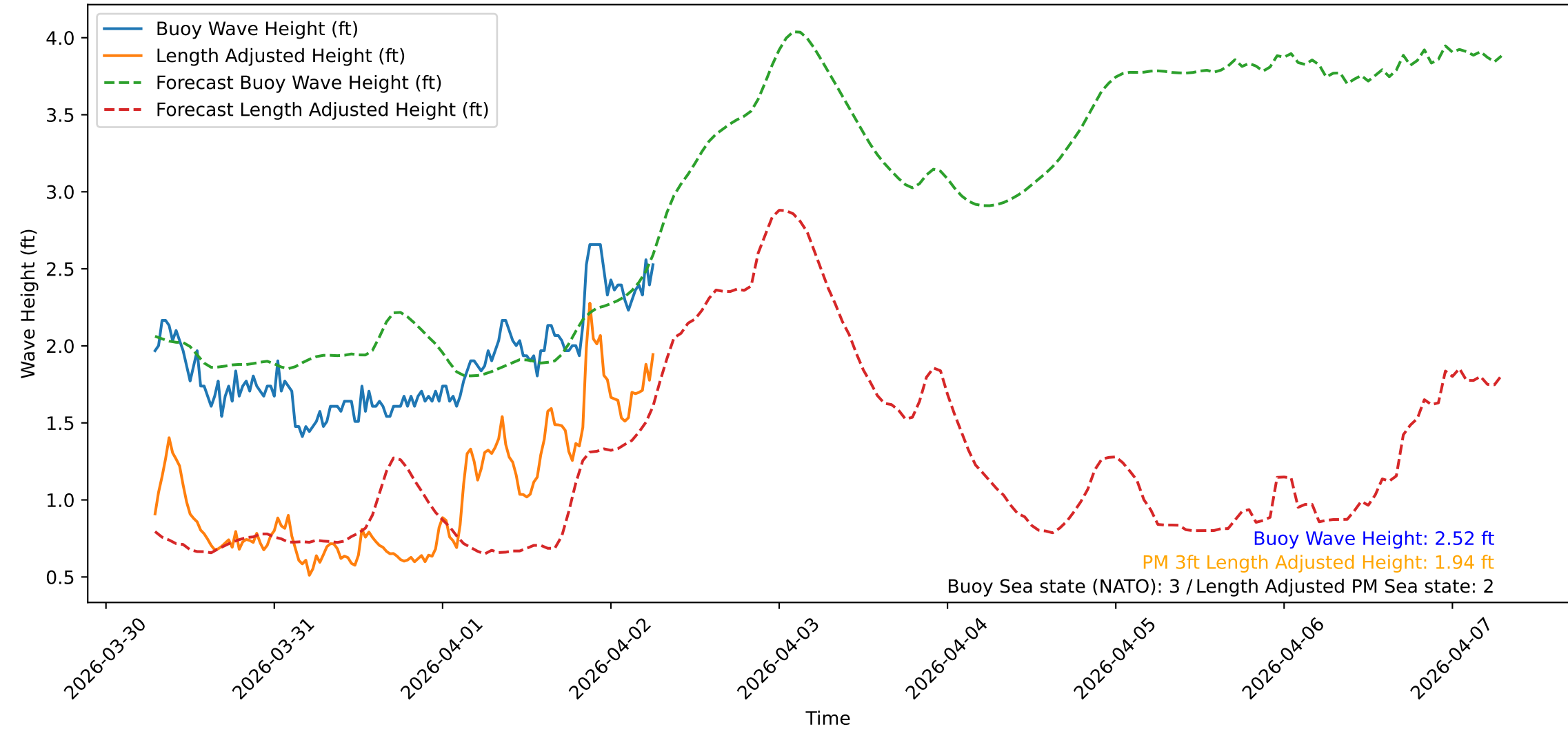
Wave Heights over Time for Green Beach at 2026-04-02 07:01:10
