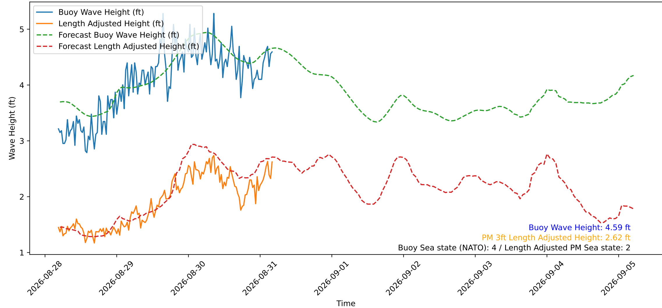
Wave Heights over Time for Oceanside Harbor at 2026-08-31 04:40:30
