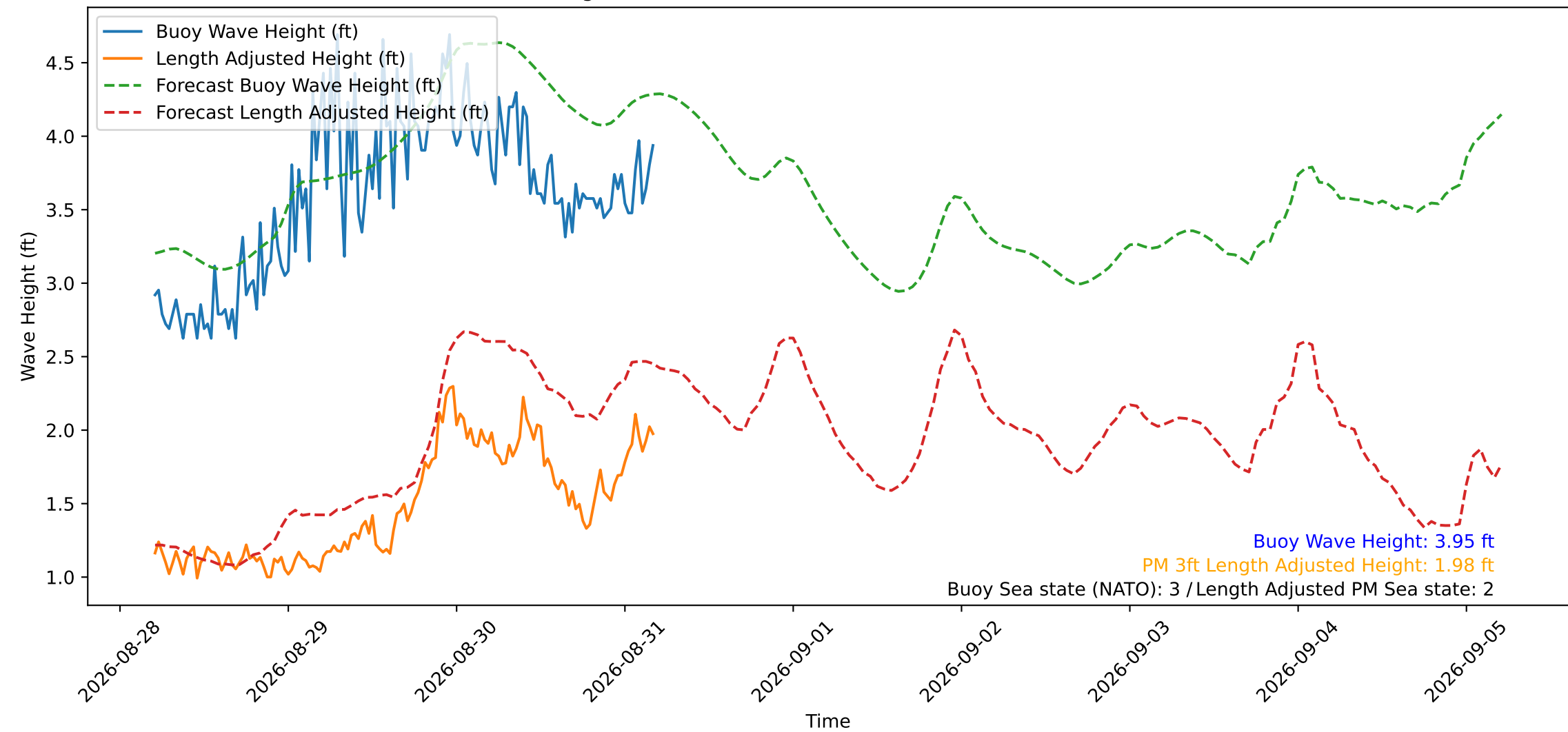
Wave Heights over Time for Red Beach at 2026-08-31 04:40:49
