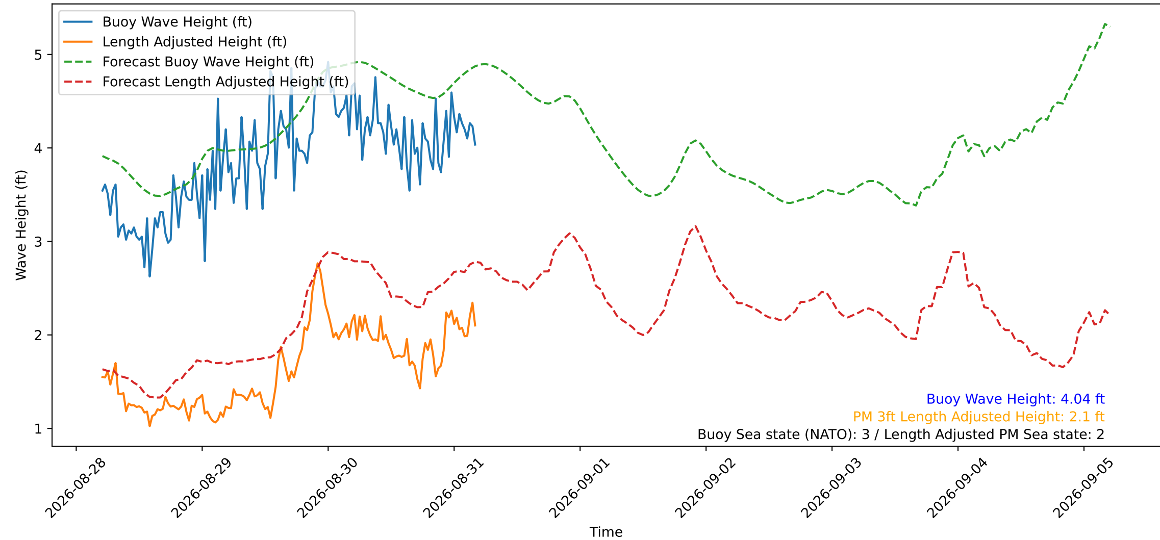
Wave Heights over Time for Green Beach at 2026-08-31 04:41:12
