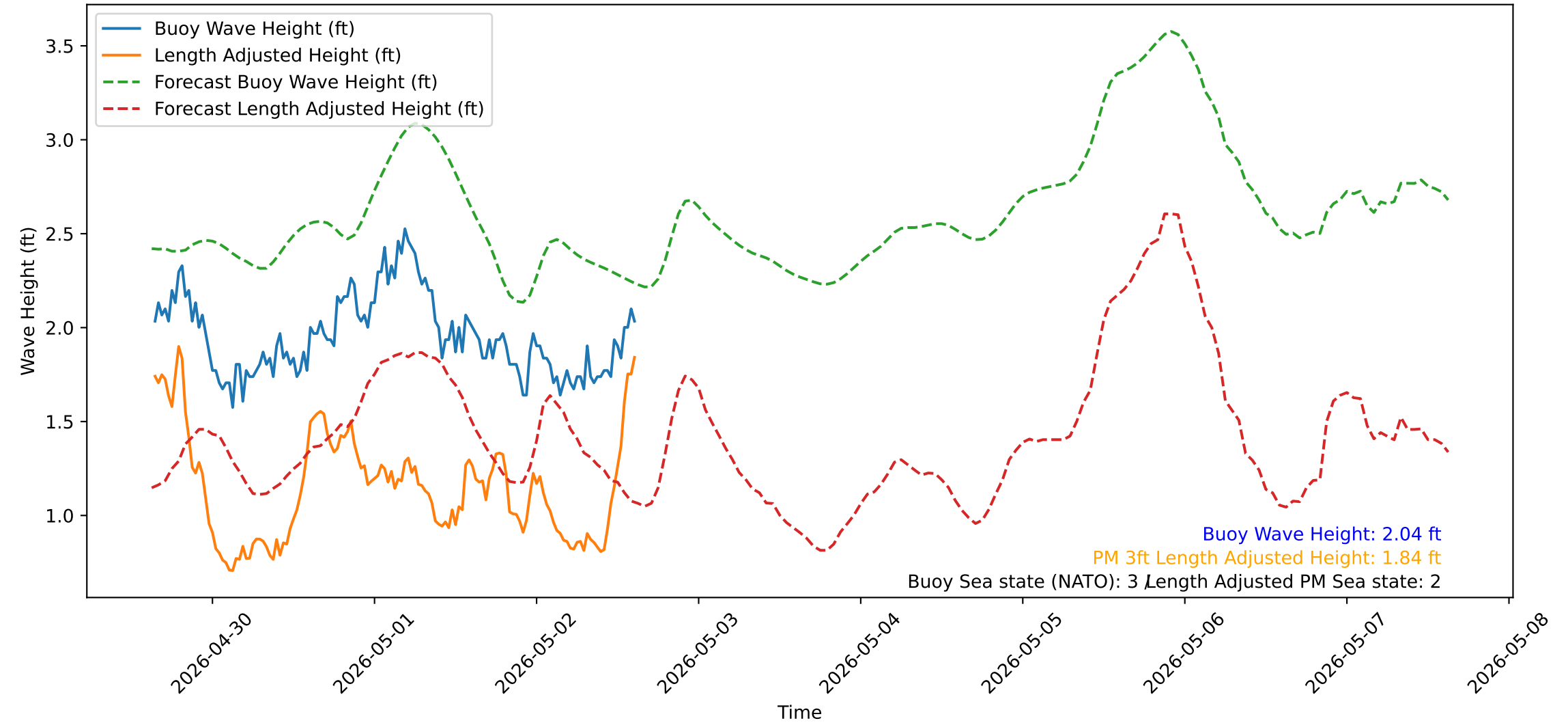
Wave Heights over Time for Red Beach at 2026-05-02 15:20:51
