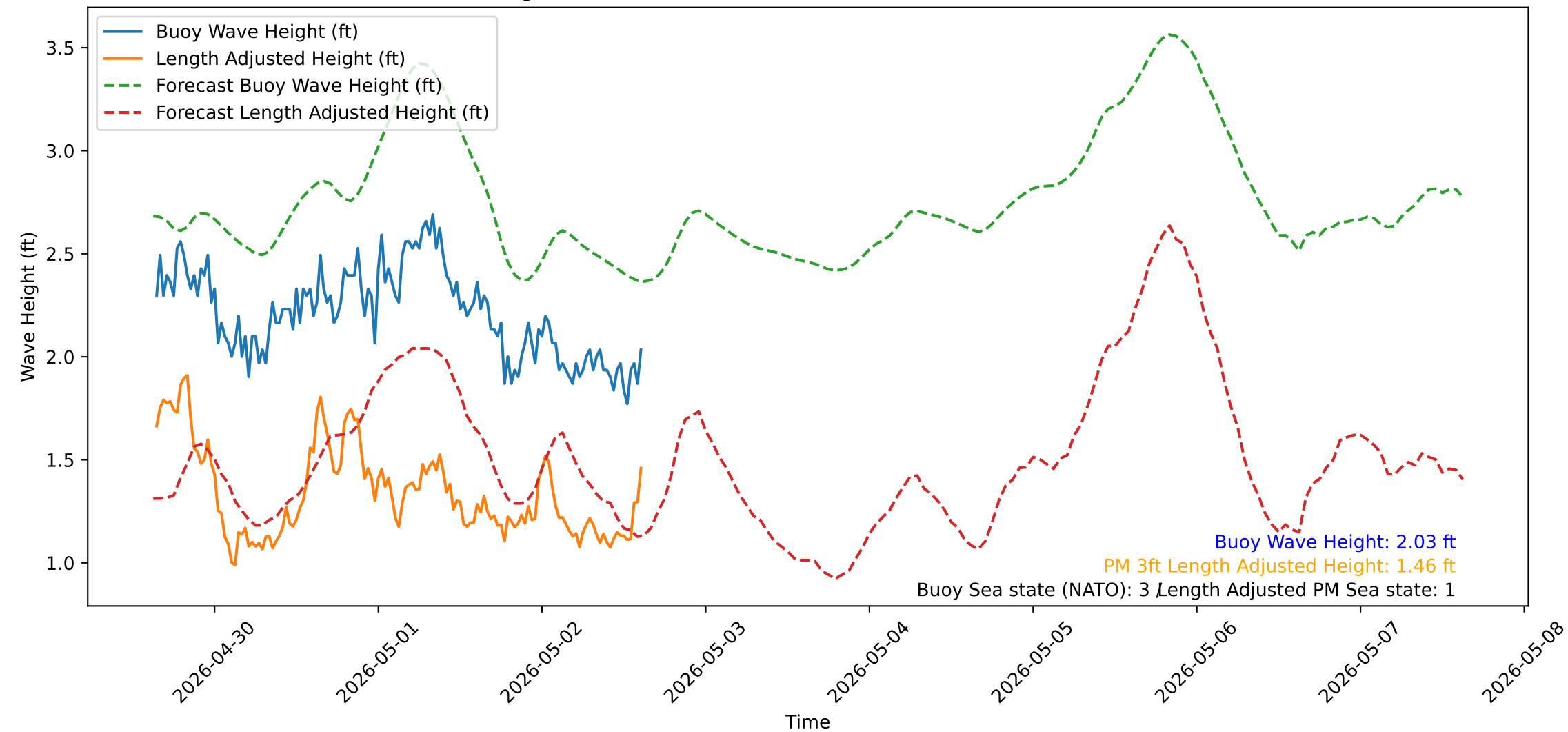
Wave Heights over Time for Oceanside Harbor at 2026-05-02 15:20:31
