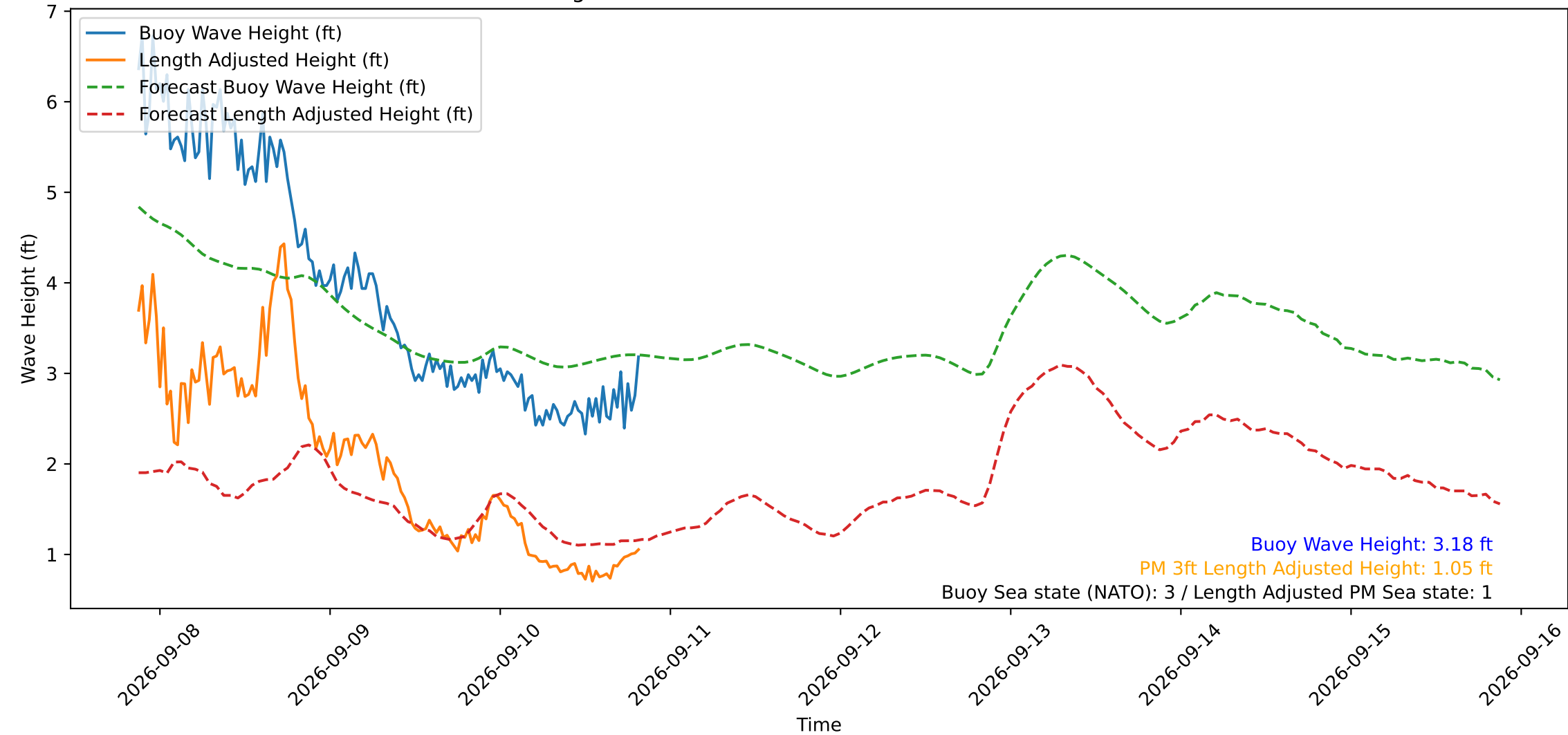
Wave Heights over Time for Red Beach at 2026-09-10 20:40:49
