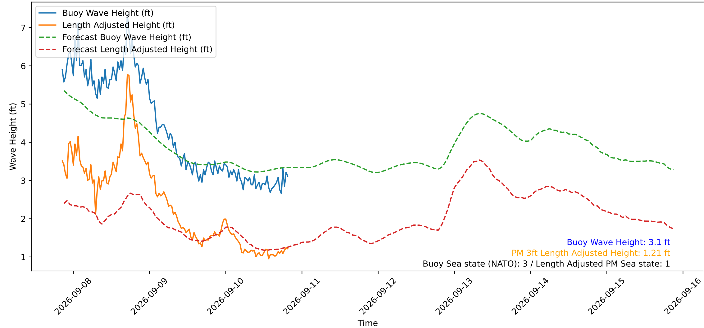
Wave Heights over Time for Oceanside Harbor at 2026-09-10 20:40:29
