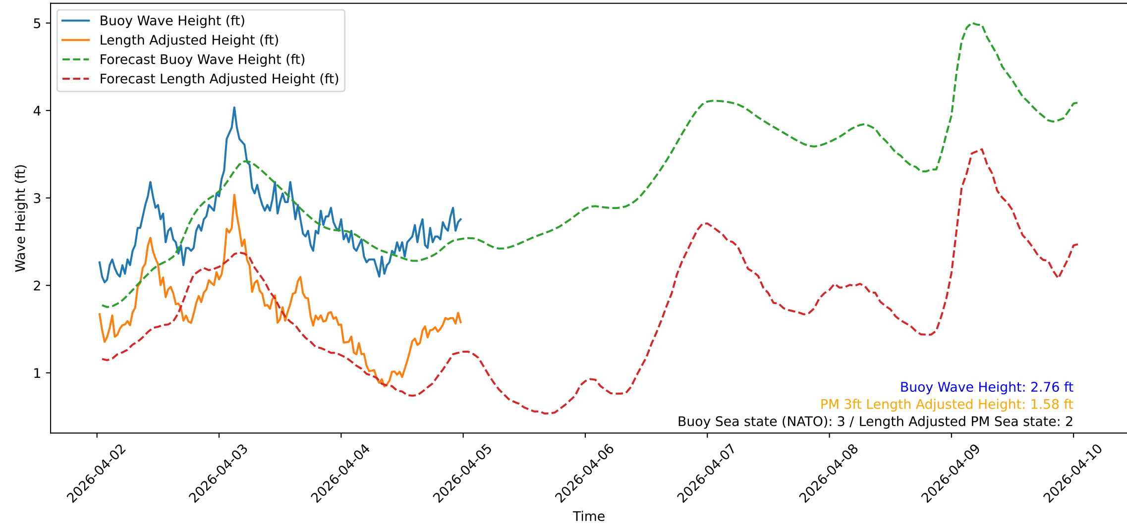
Wave Heights over Time for Oceanside Harbor at 2026-04-05 00:30:32
