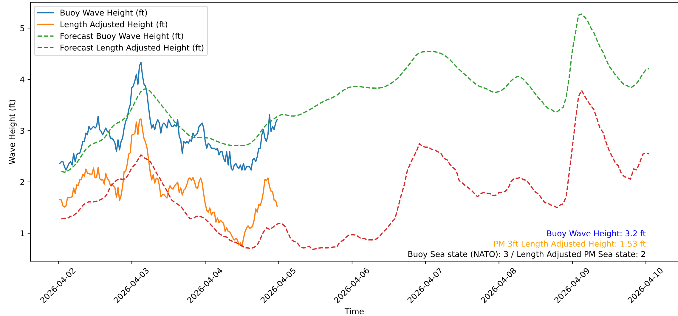
Wave Heights over Time for Green Beach at 2026-04-05 00:31:09
