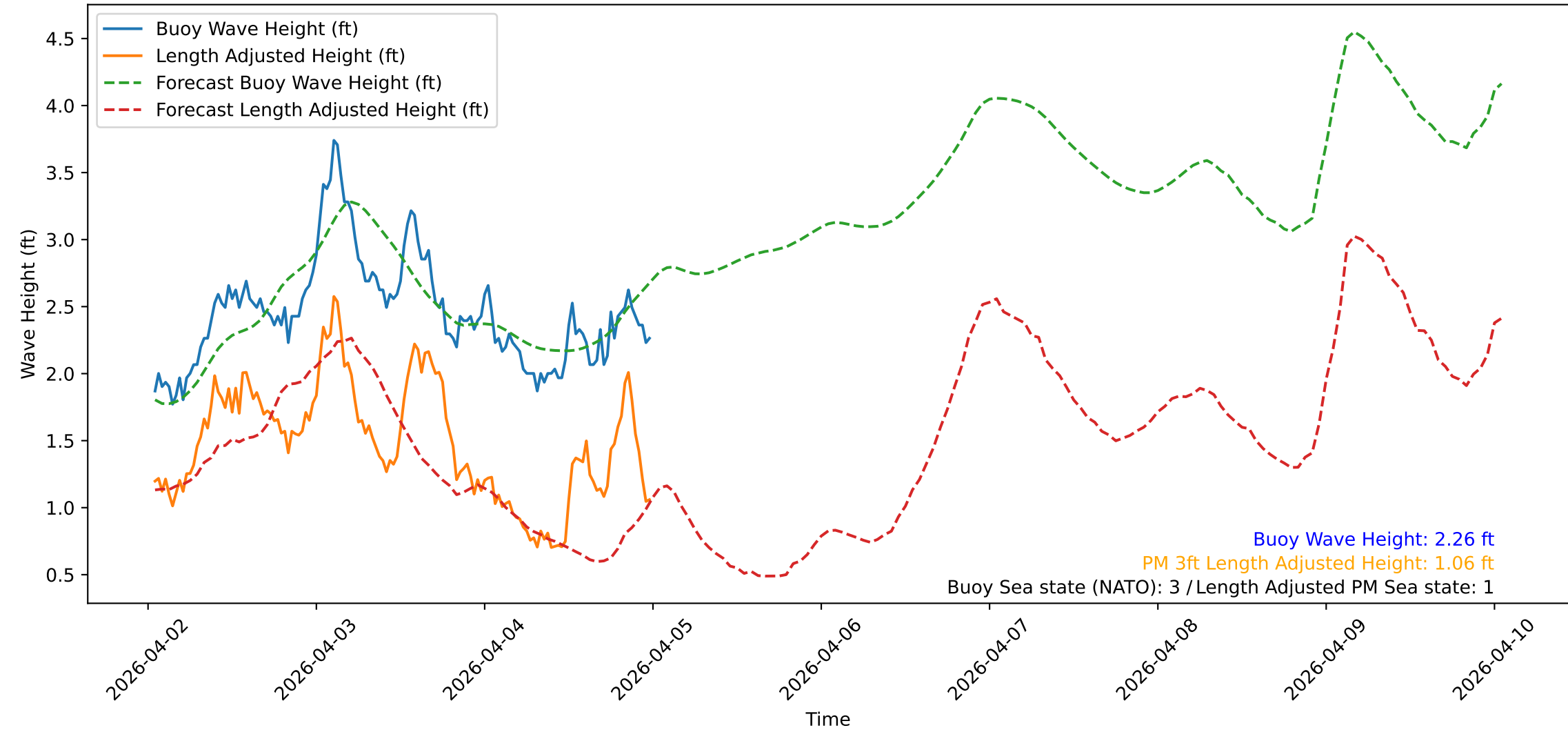
Wave Heights over Time for Red Beach at 2026-04-05 00:30:47
