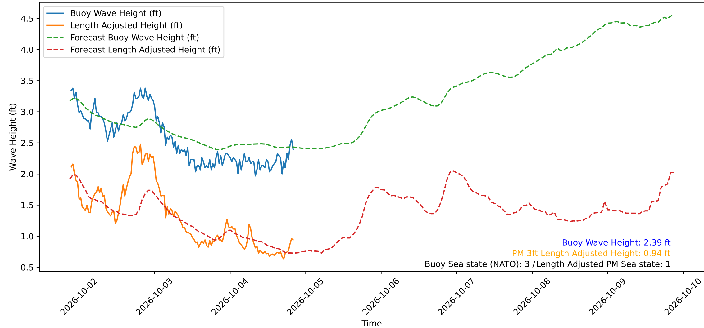
Wave Heights over Time for Green Beach at 2026-10-04 21:01:11
