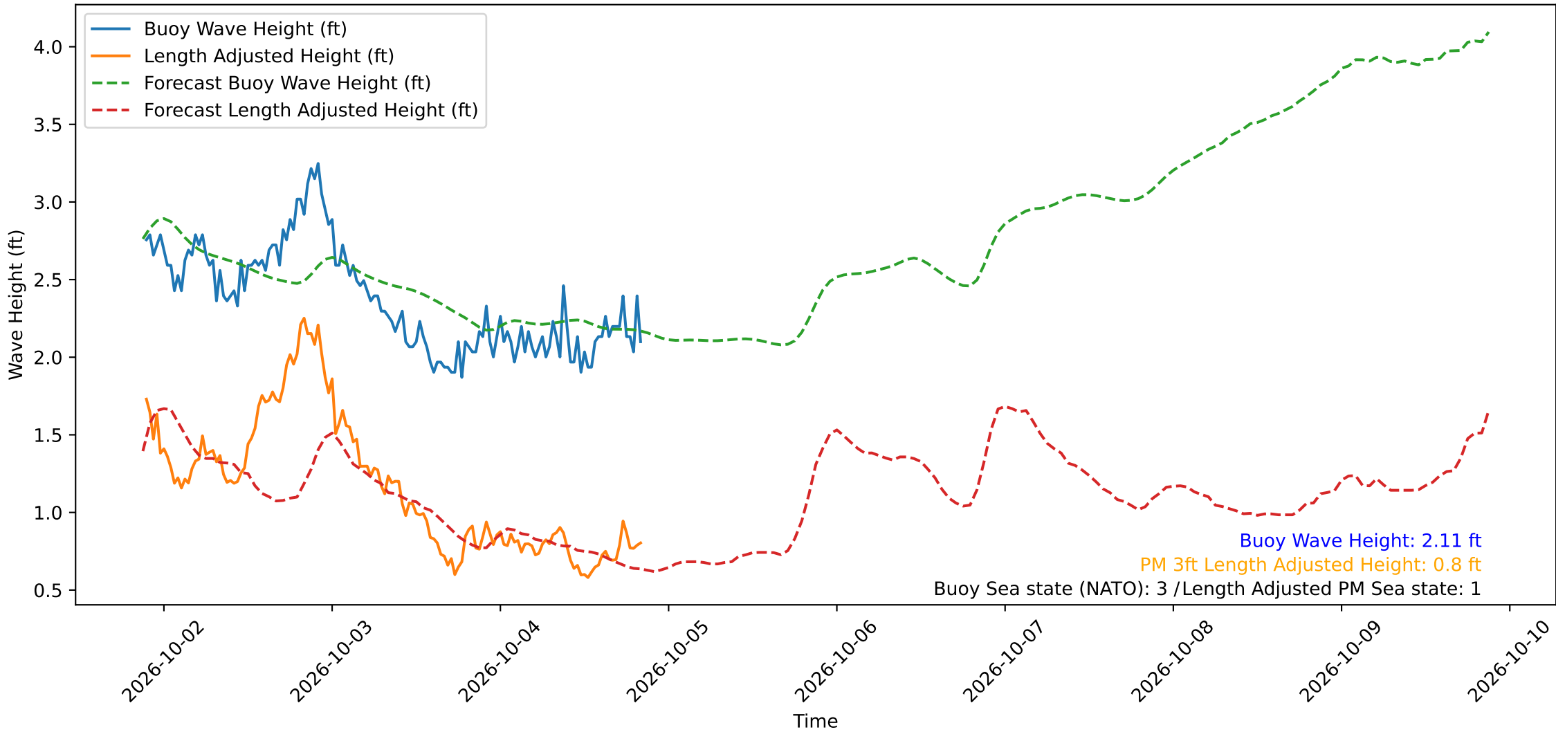
Wave Heights over Time for Red Beach at 2026-10-04 21:00:48
