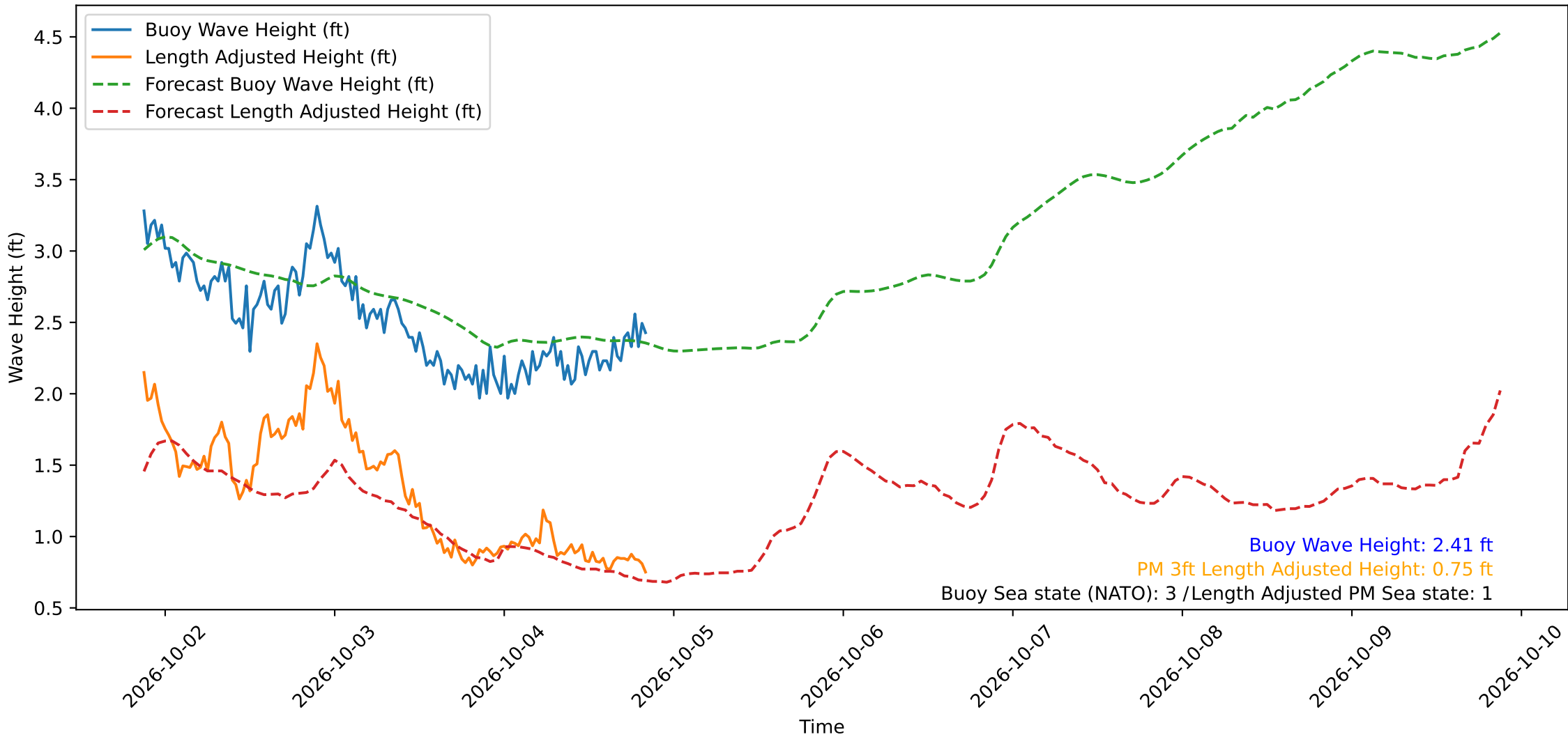
Wave Heights over Time for Oceanside Harbor at 2026-10-04 21:00:29
