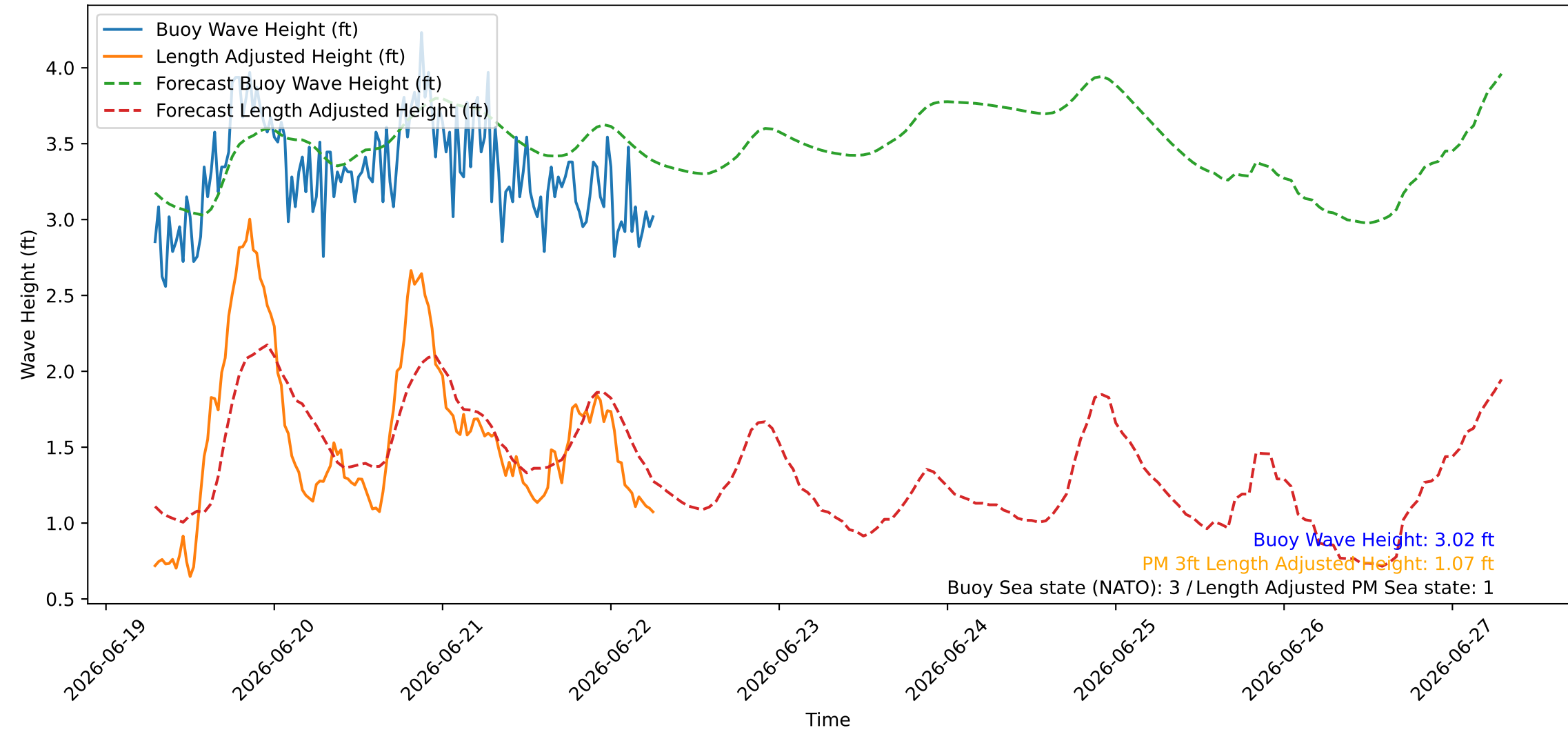
Wave Heights over Time for Green Beach at 2026-06-22 06:51:09
