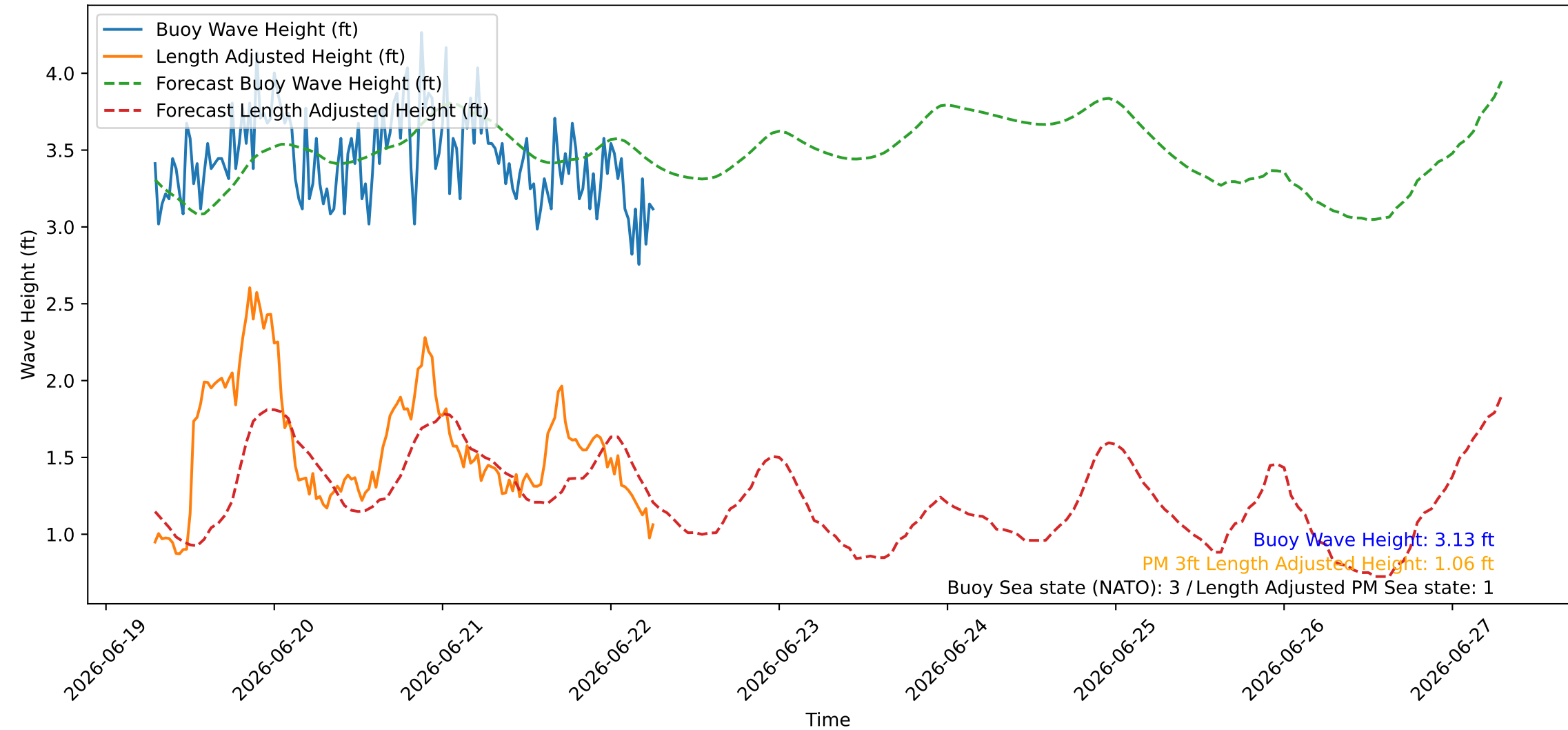
Wave Heights over Time for Oceanside Harbor at 2026-06-22 06:50:26
