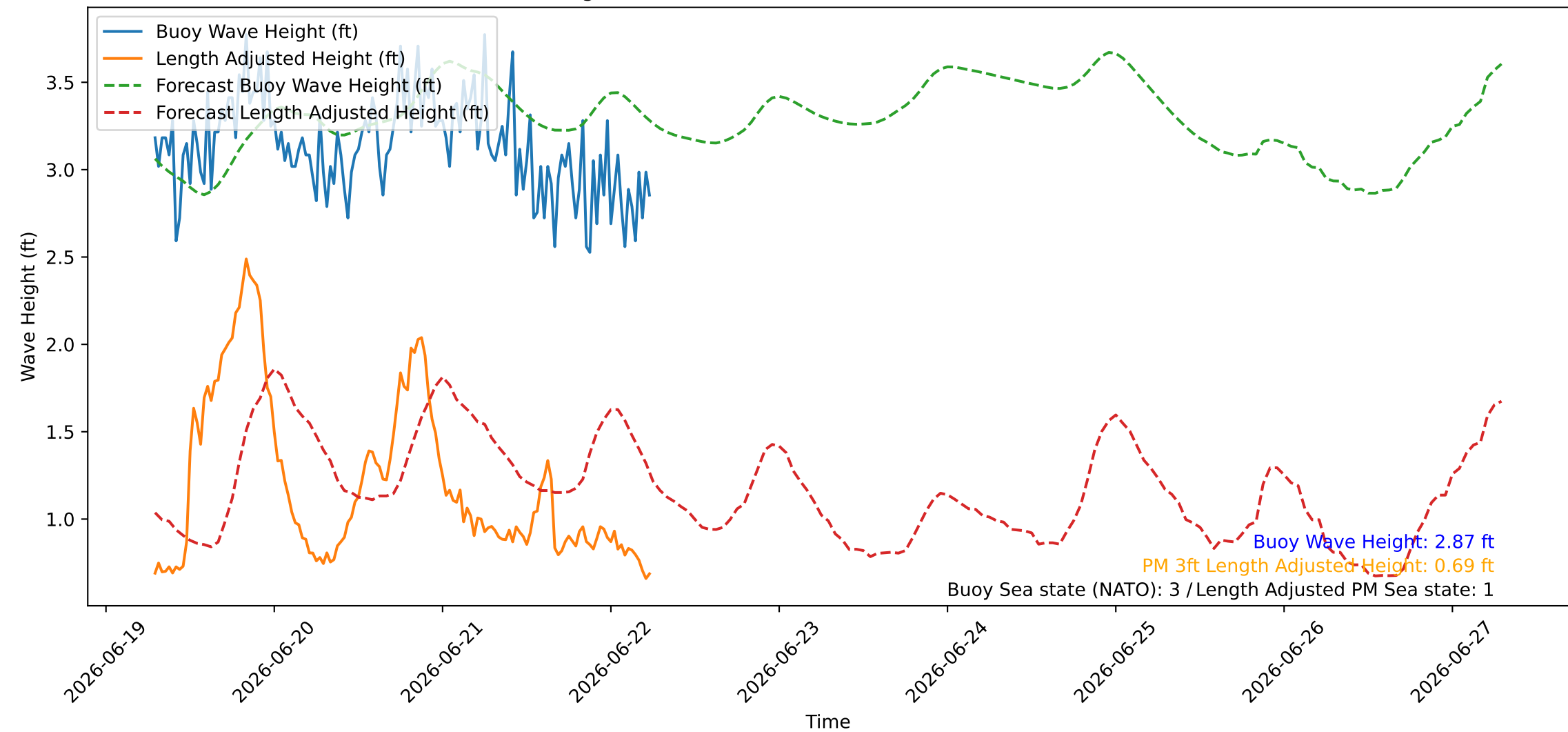
Wave Heights over Time for Red Beach at 2026-06-22 06:50:47
