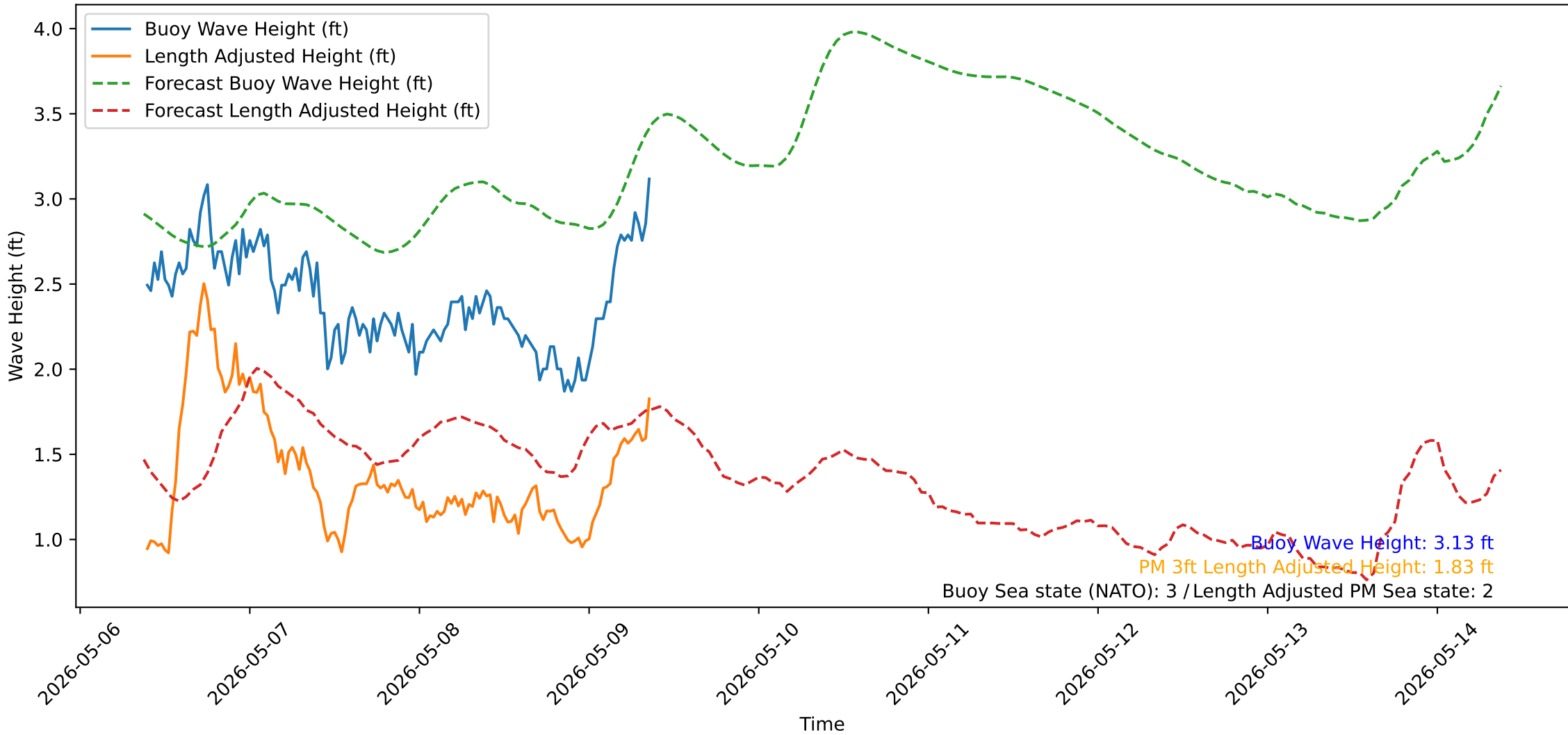
Wave Heights over Time for Oceanside Harbor at 2026-05-09 09:20:32
