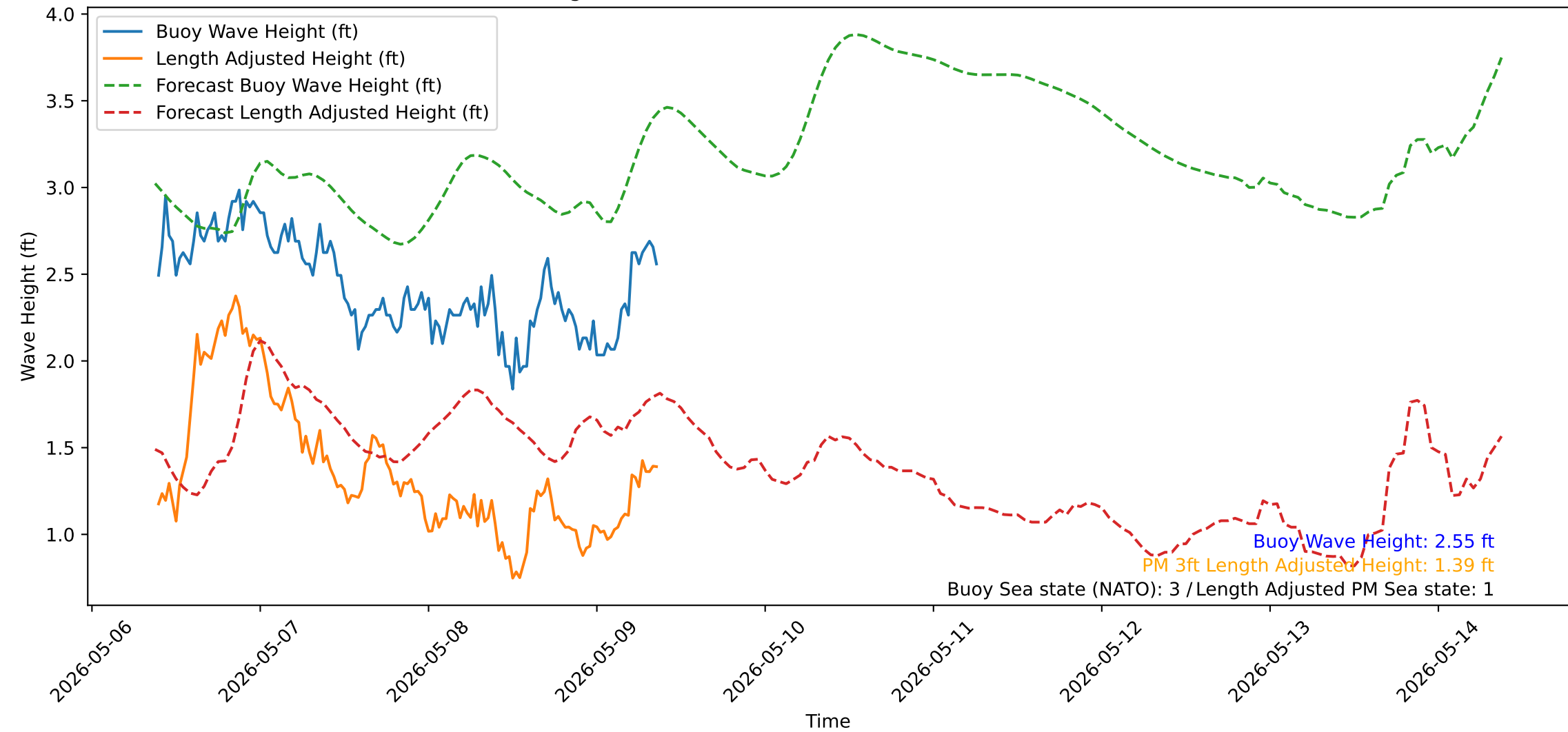
Wave Heights over Time for Green Beach at 2026-05-09 09:21:15
