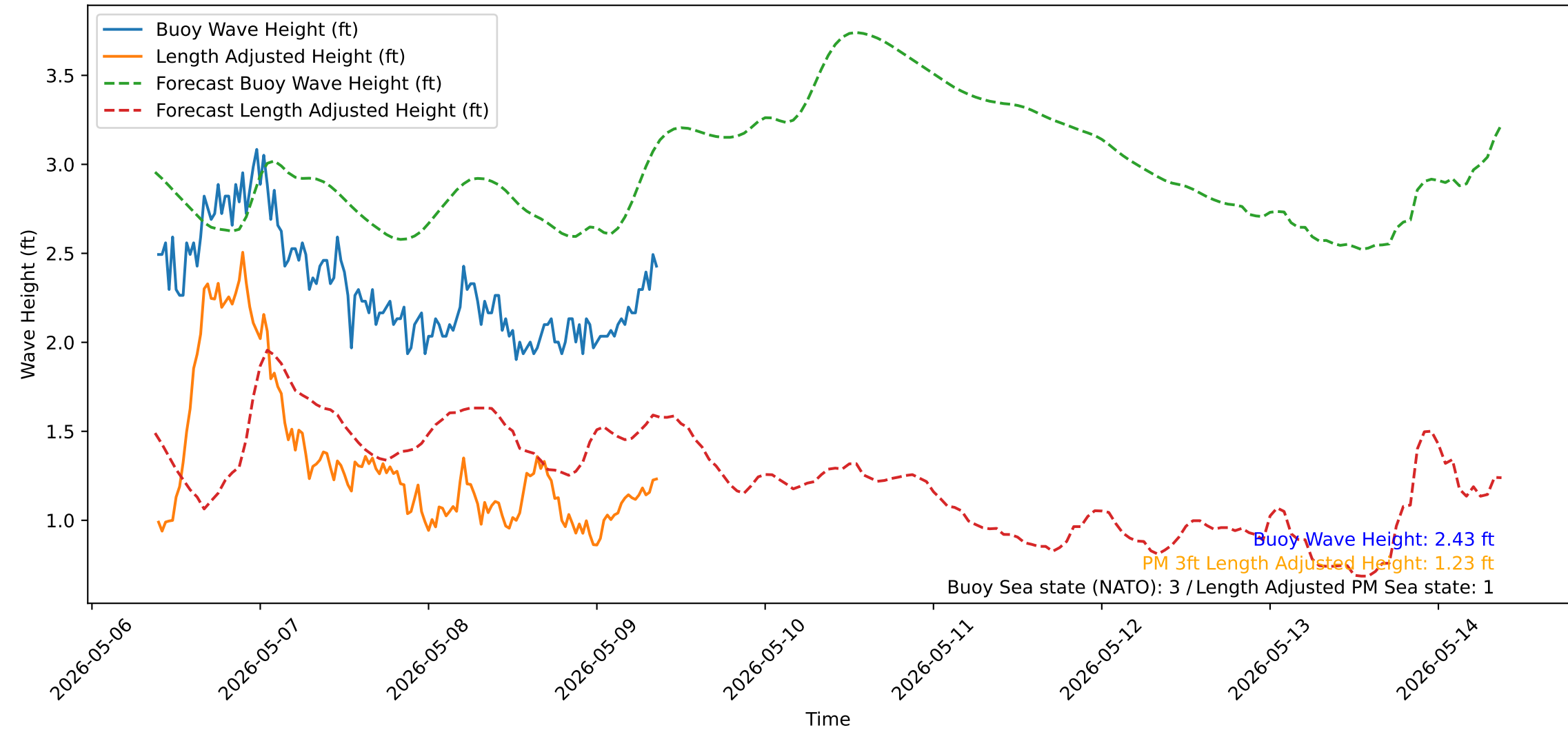
Wave Heights over Time for Red Beach at 2026-05-09 09:20:53
