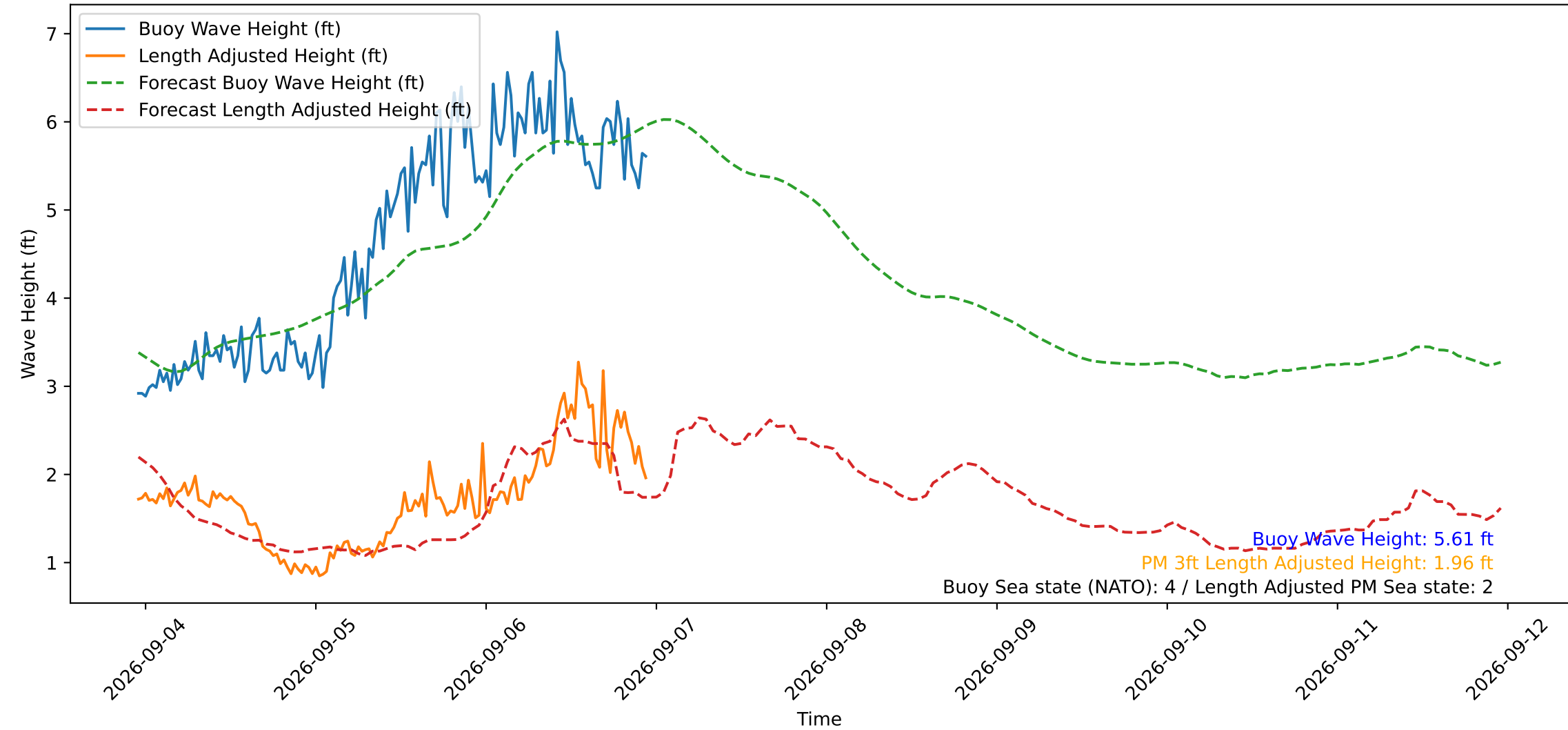
Wave Heights over Time for Oceanside Harbor at 2026-09-06 23:10:29
