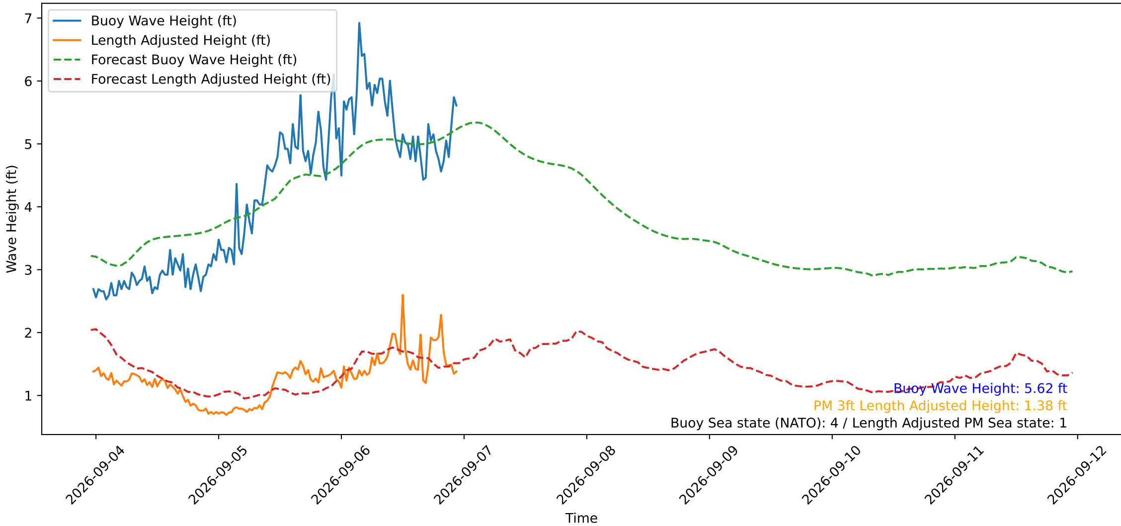
Wave Heights over Time for Red Beach at 2026-09-06 23:10:49
