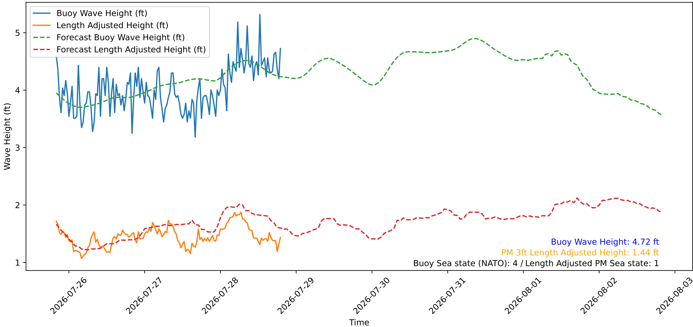
Wave Heights over Time for Oceanside Harbor at 2026-07-28 20:00:26
