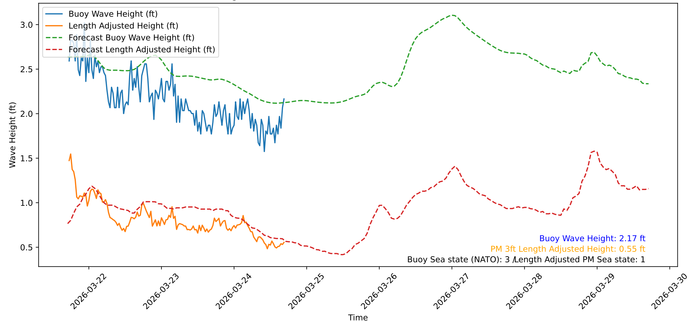
Wave Heights over Time for Oceanside Harbor at 2026-03-24 17:20:32
