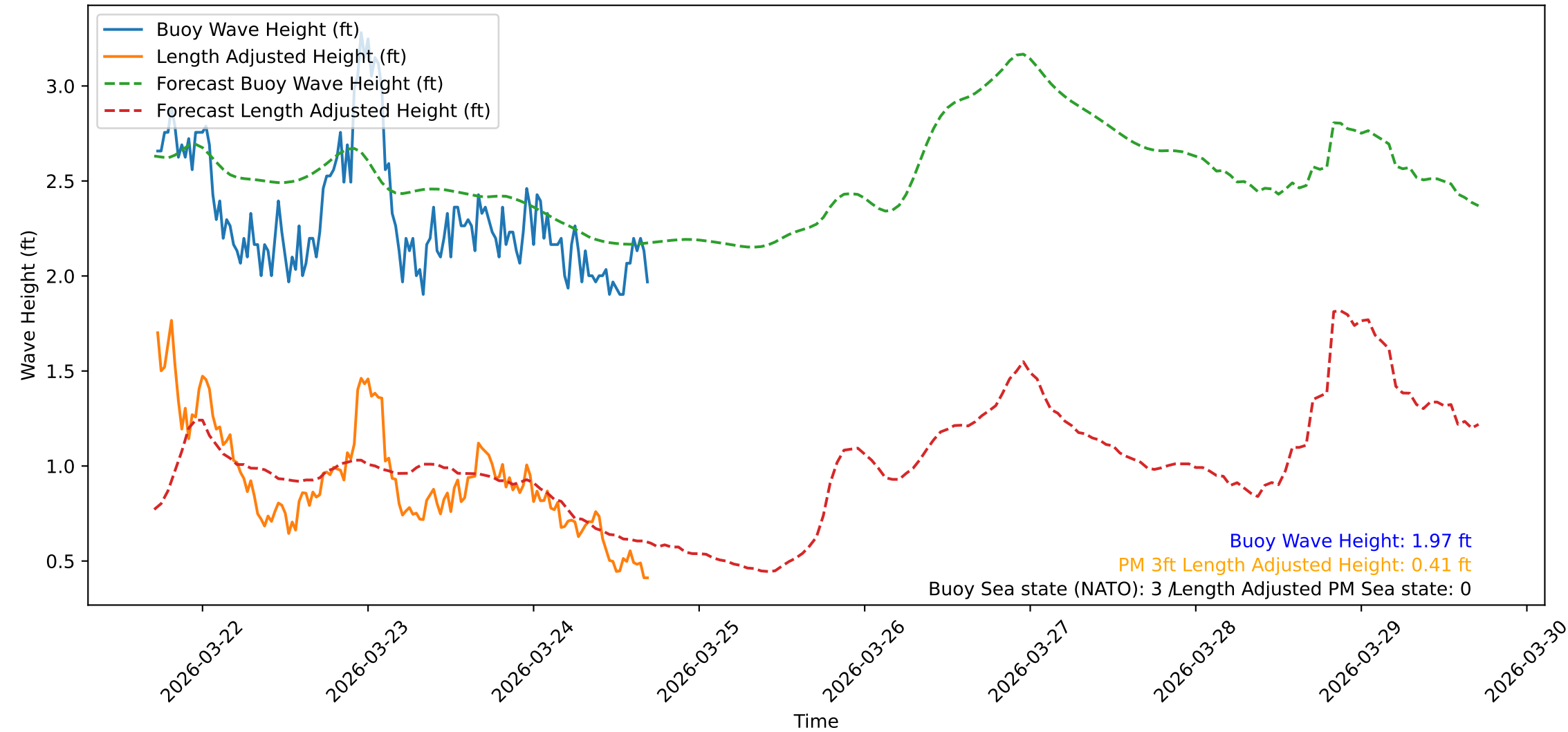
Wave Heights over Time for Green Beach at 2026-03-24 17:21:10
