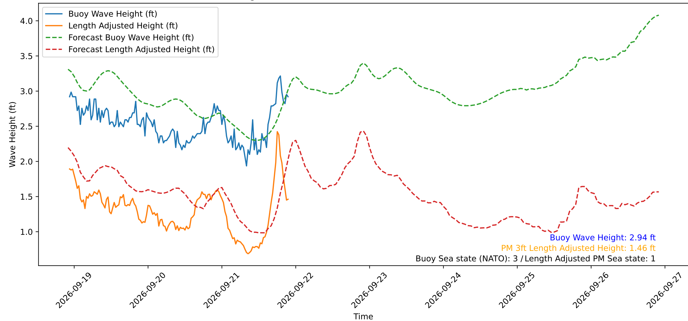
Wave Heights over Time for Green Beach at 2026-09-21 22:11:12
