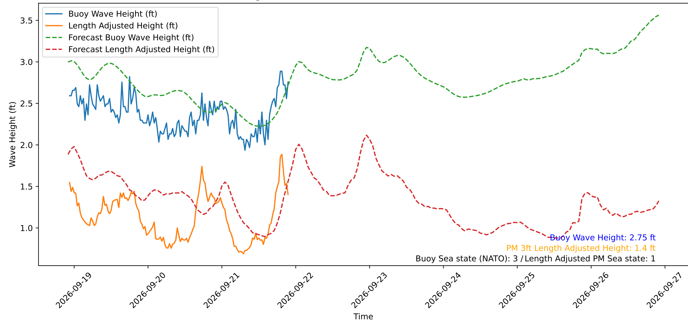
Wave Heights over Time for Red Beach at 2026-09-21 22:10:50
