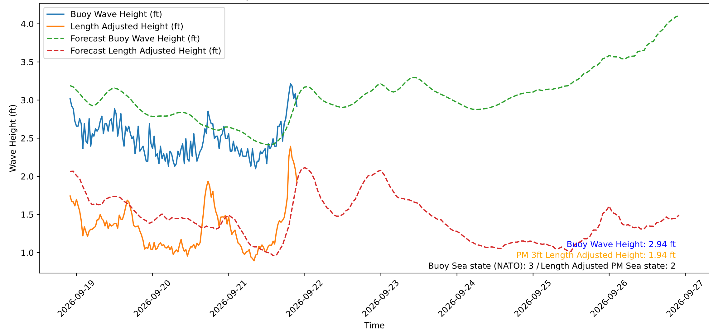
Wave Heights over Time for Oceanside Harbor at 2026-09-21 22:10:30
