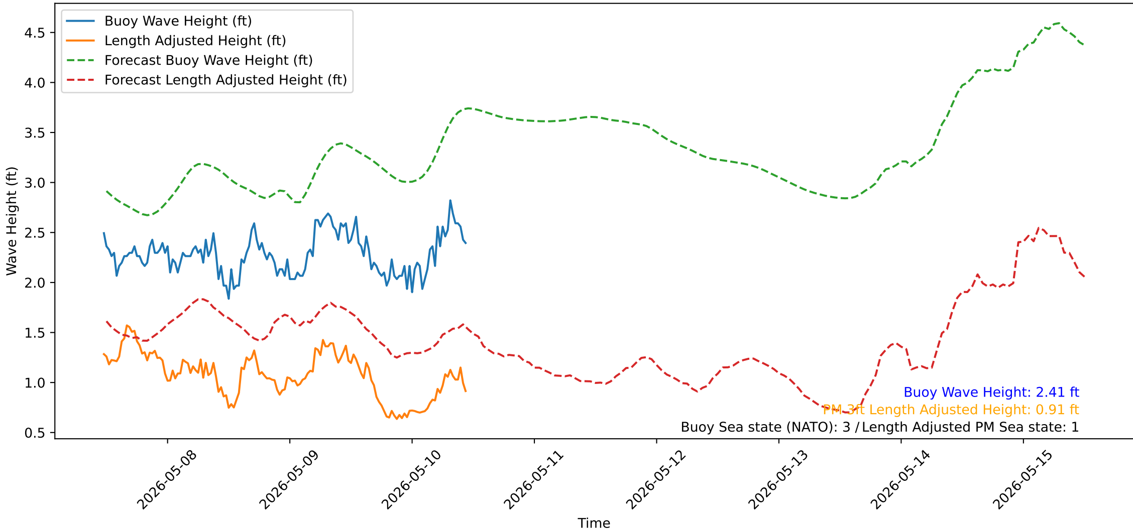
Wave Heights over Time for Green Beach at 2026-05-10 11:31:13
