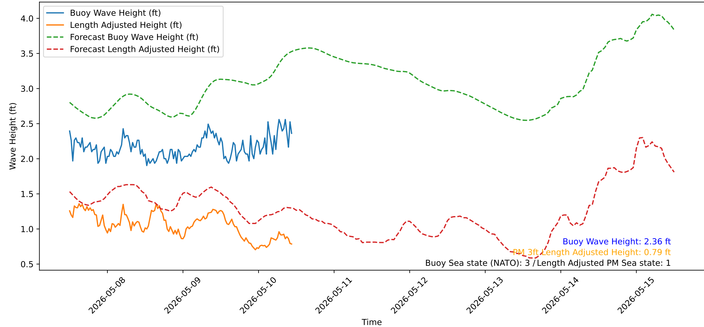
Wave Heights over Time for Red Beach at 2026-05-10 11:30:51
