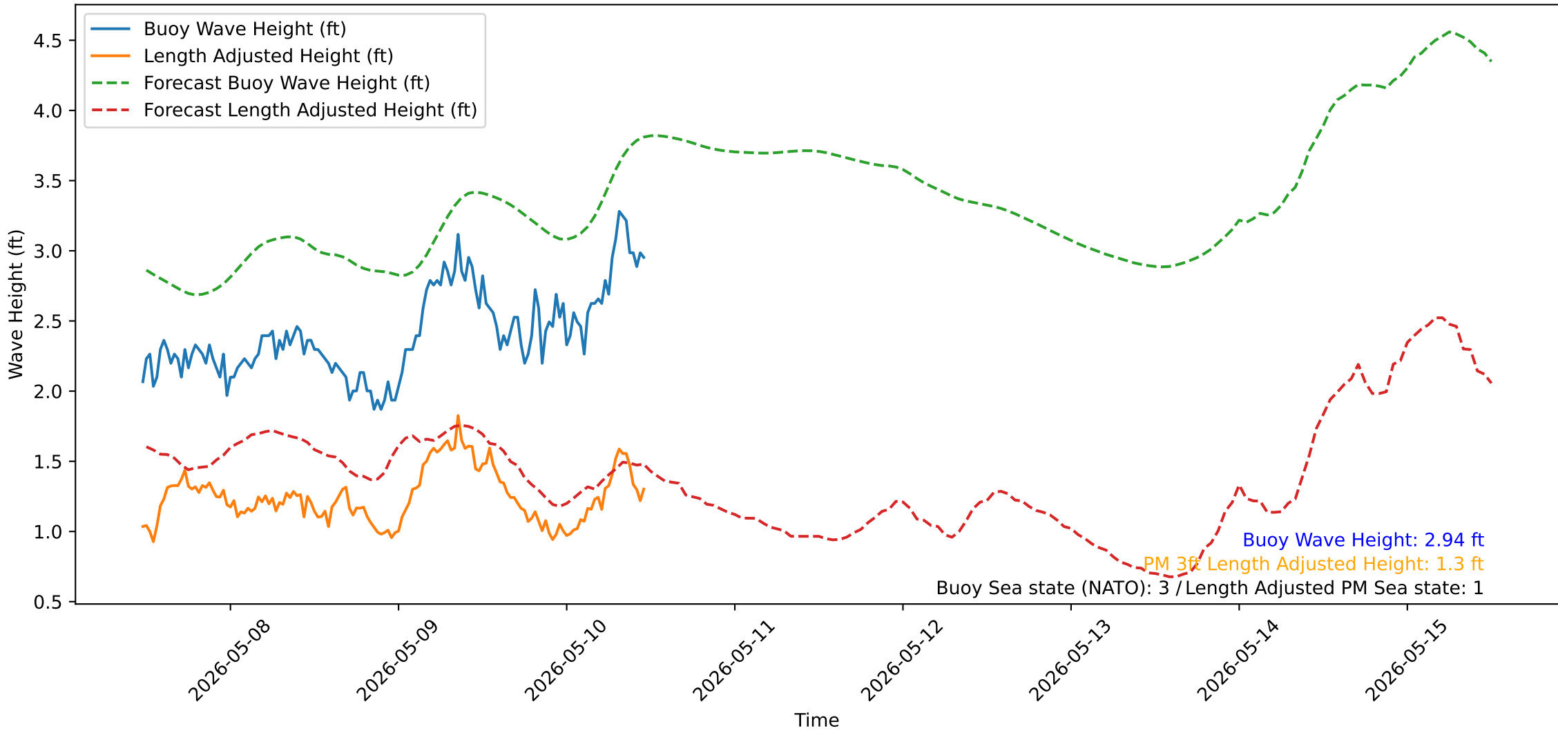
Wave Heights over Time for Oceanside Harbor at 2026-05-10 11:30:31
