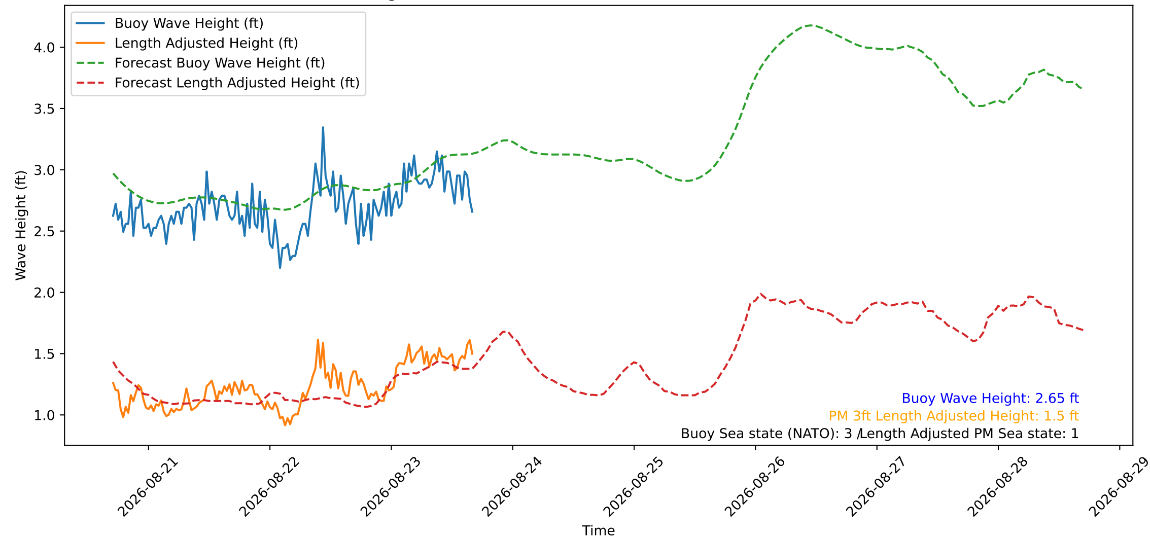
Wave Heights over Time for Oceanside Harbor at 2026-08-23 16:50:29
