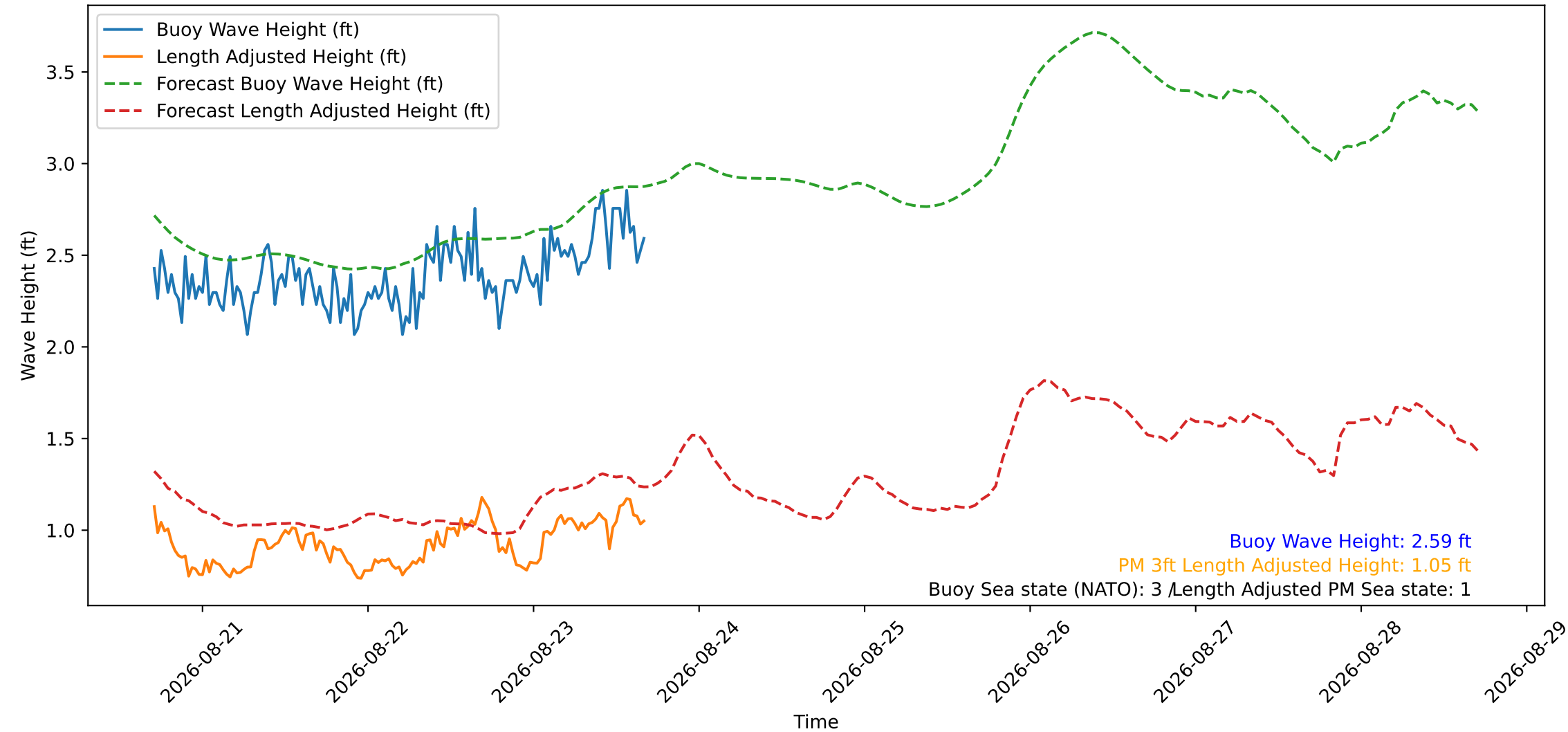
Wave Heights over Time for Red Beach at 2026-08-23 16:50:50
