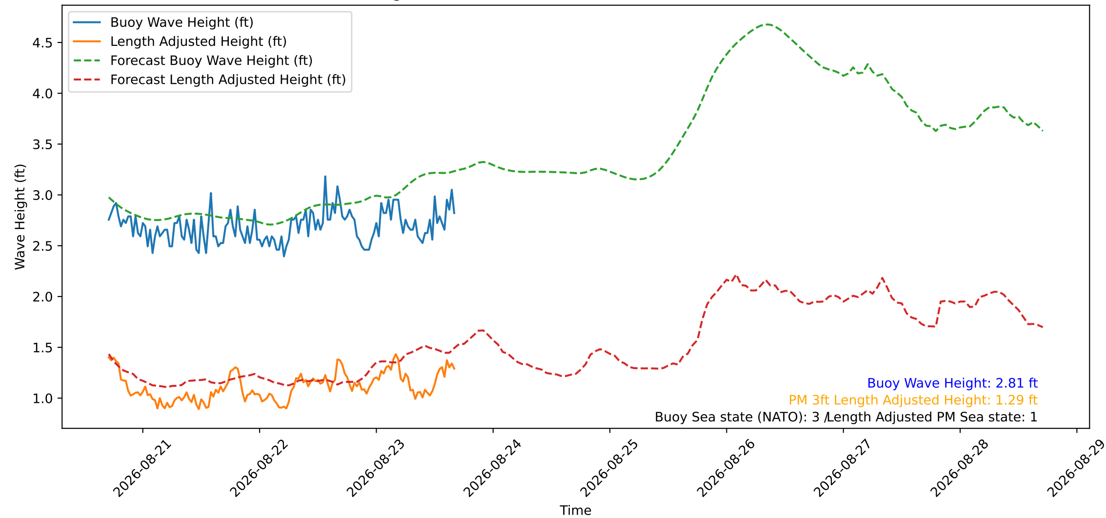
Wave Heights over Time for Green Beach at 2026-08-23 16:51:14
