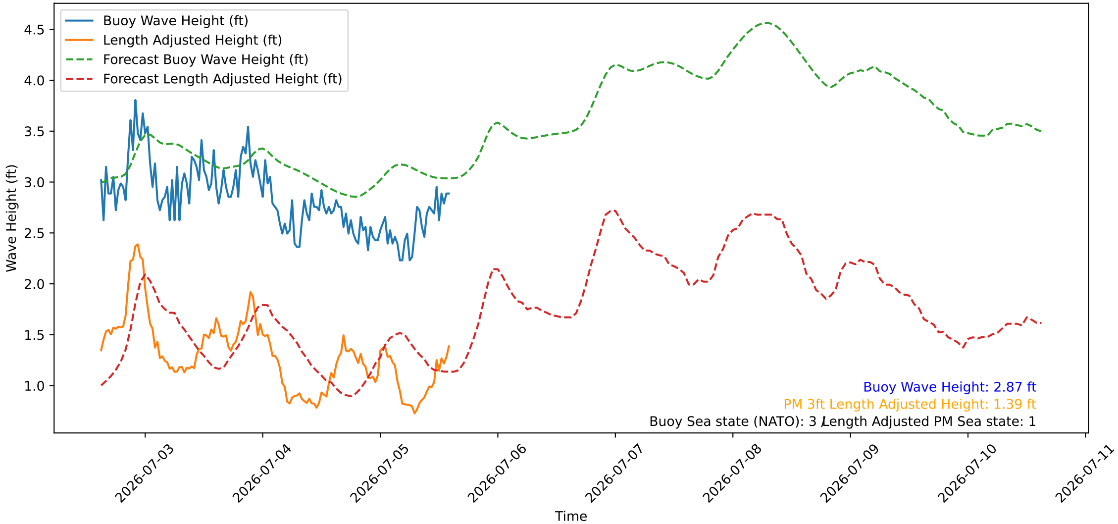
Wave Heights over Time for Red Beach at 2026-07-05 14:40:47
