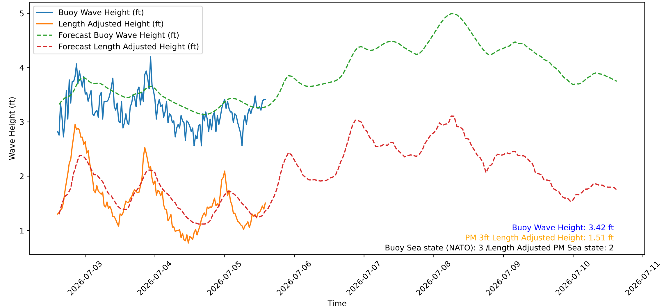
Wave Heights over Time for Green Beach at 2026-07-05 14:41:10
