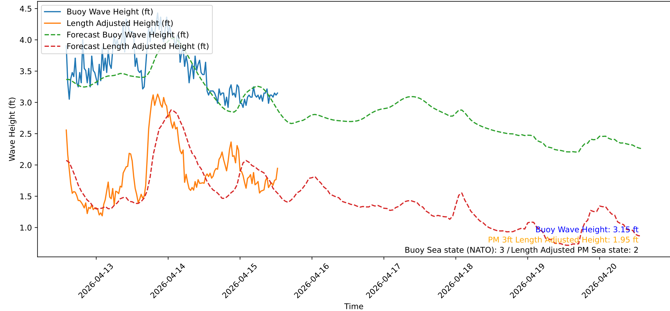
Wave Heights over Time for Red Beach at 2026-04-15 13:30:50
