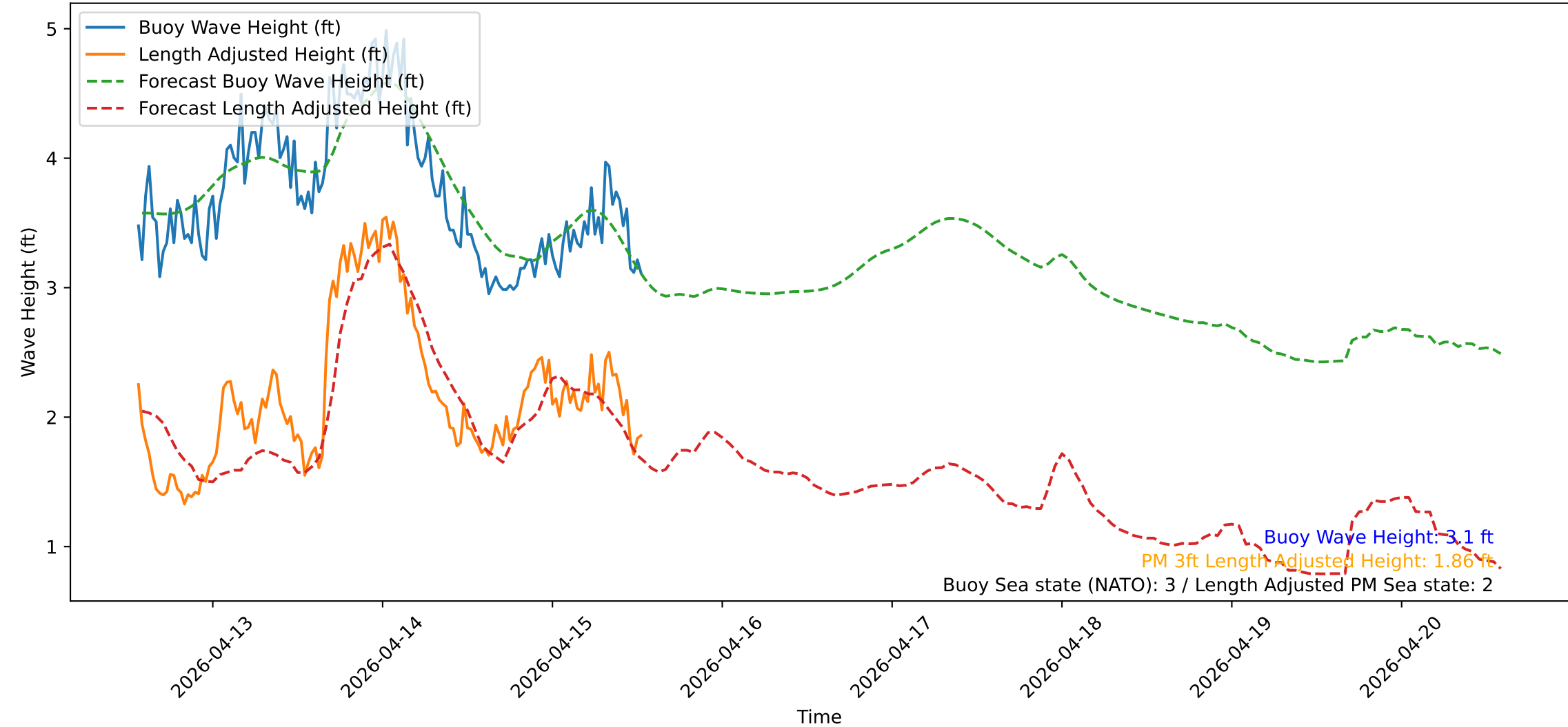
Wave Heights over Time for Green Beach at 2026-04-15 13:31:13
