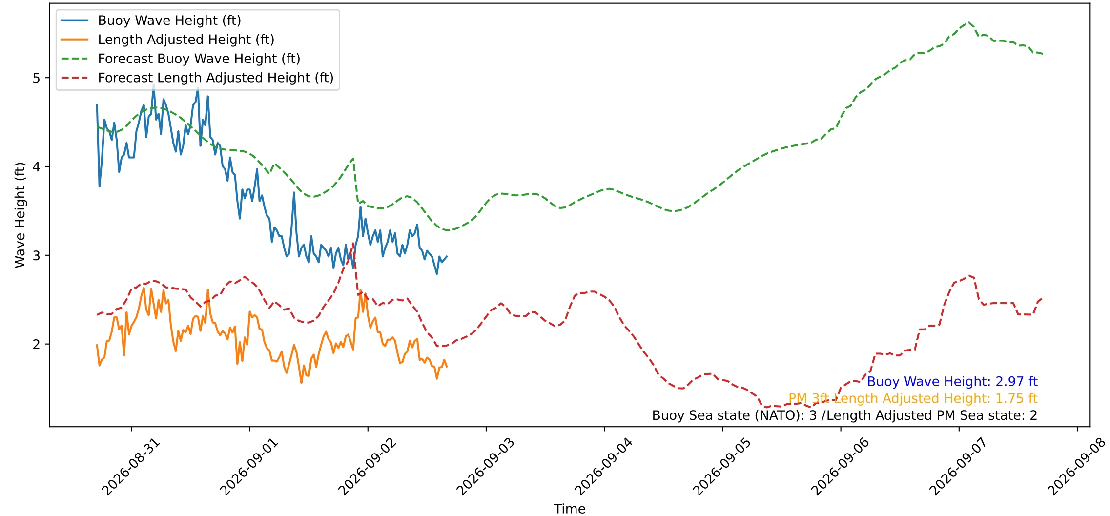
Wave Heights over Time for Oceanside Harbor at 2026-09-02 16:50:29
