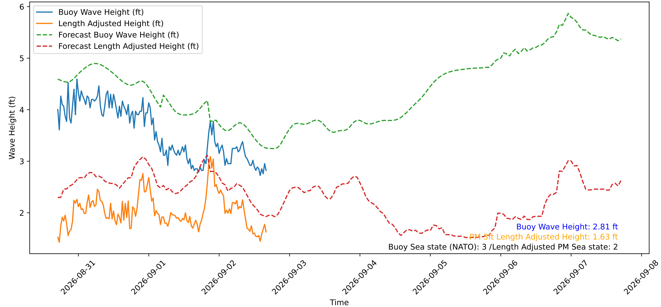
Wave Heights over Time for Green Beach at 2026-09-02 16:51:15
