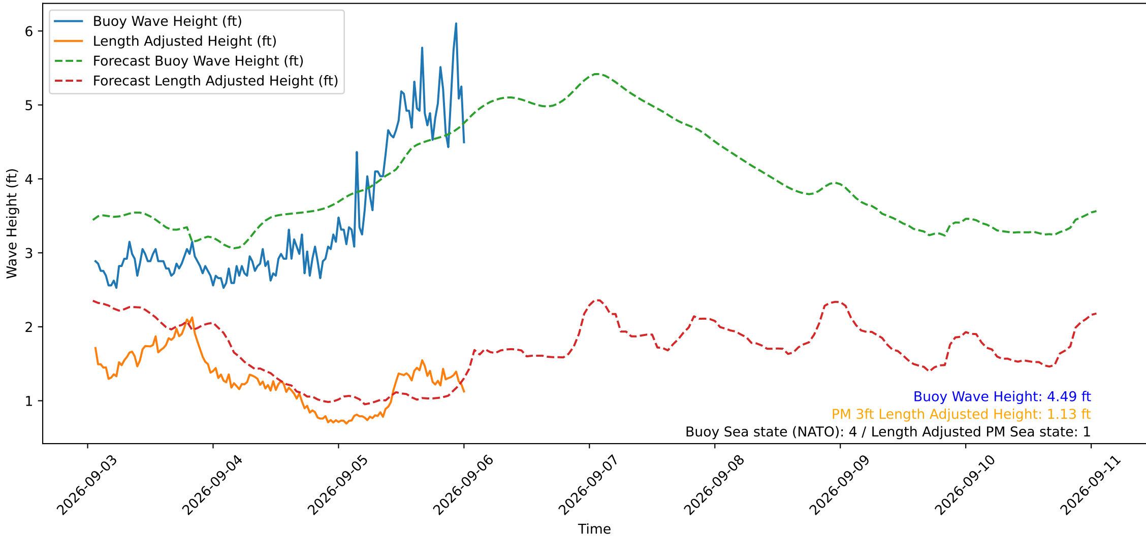
Wave Heights over Time for Red Beach at 2026-09-06 01:20:51
