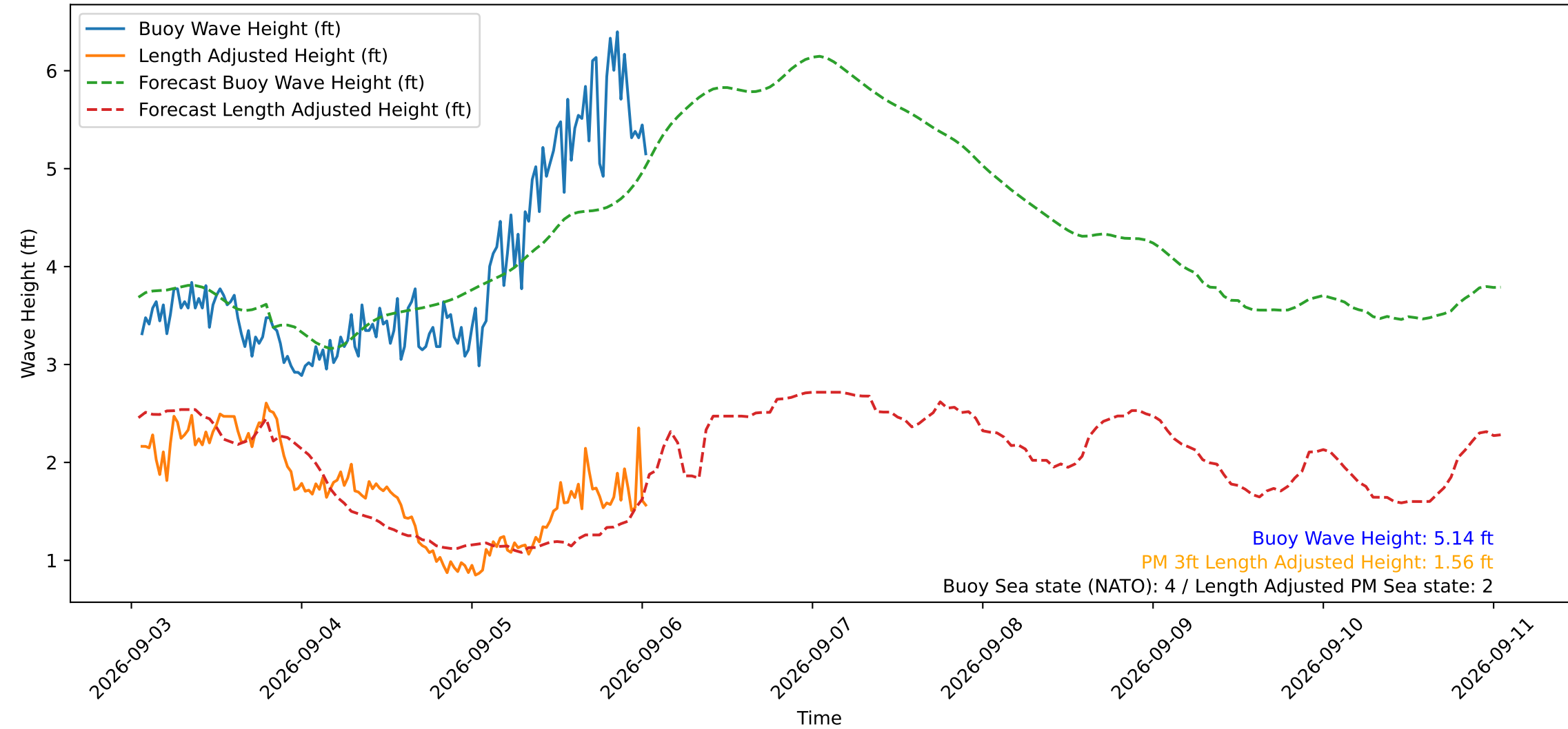
Wave Heights over Time for Oceanside Harbor at 2026-09-06 01:20:30
