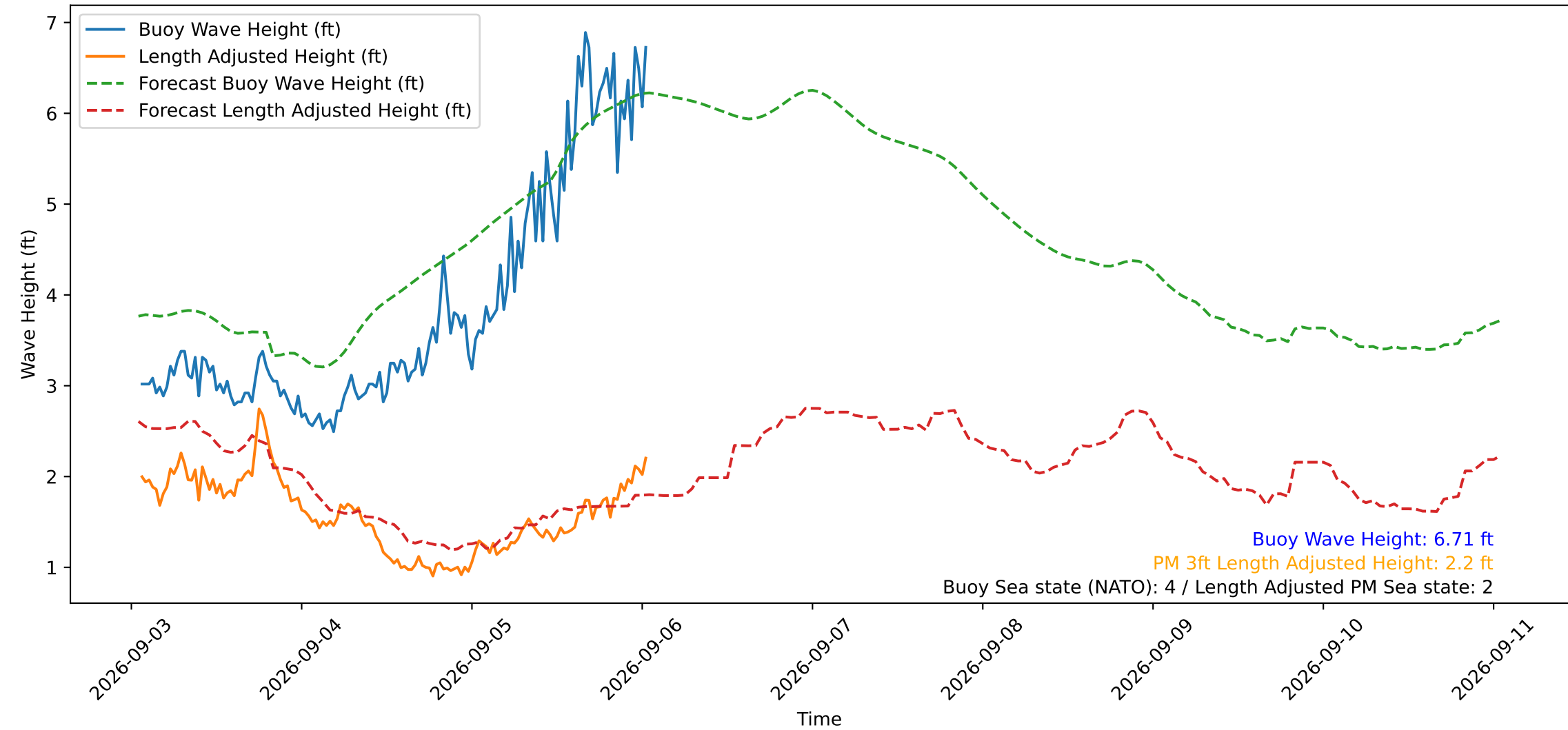
Wave Heights over Time for Green Beach at 2026-09-06 01:21:15
