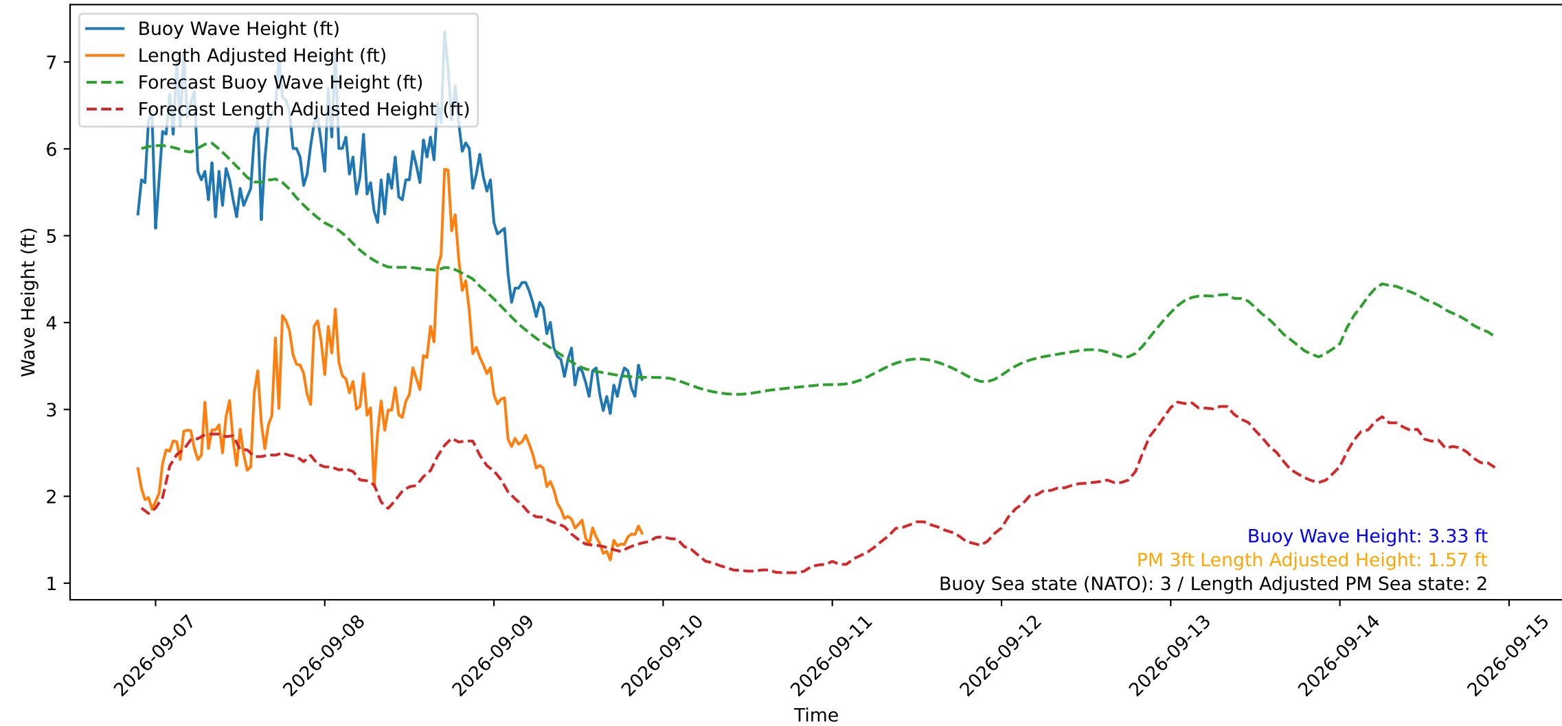
Wave Heights over Time for Oceanside Harbor at 2026-09-09 21:30:29
