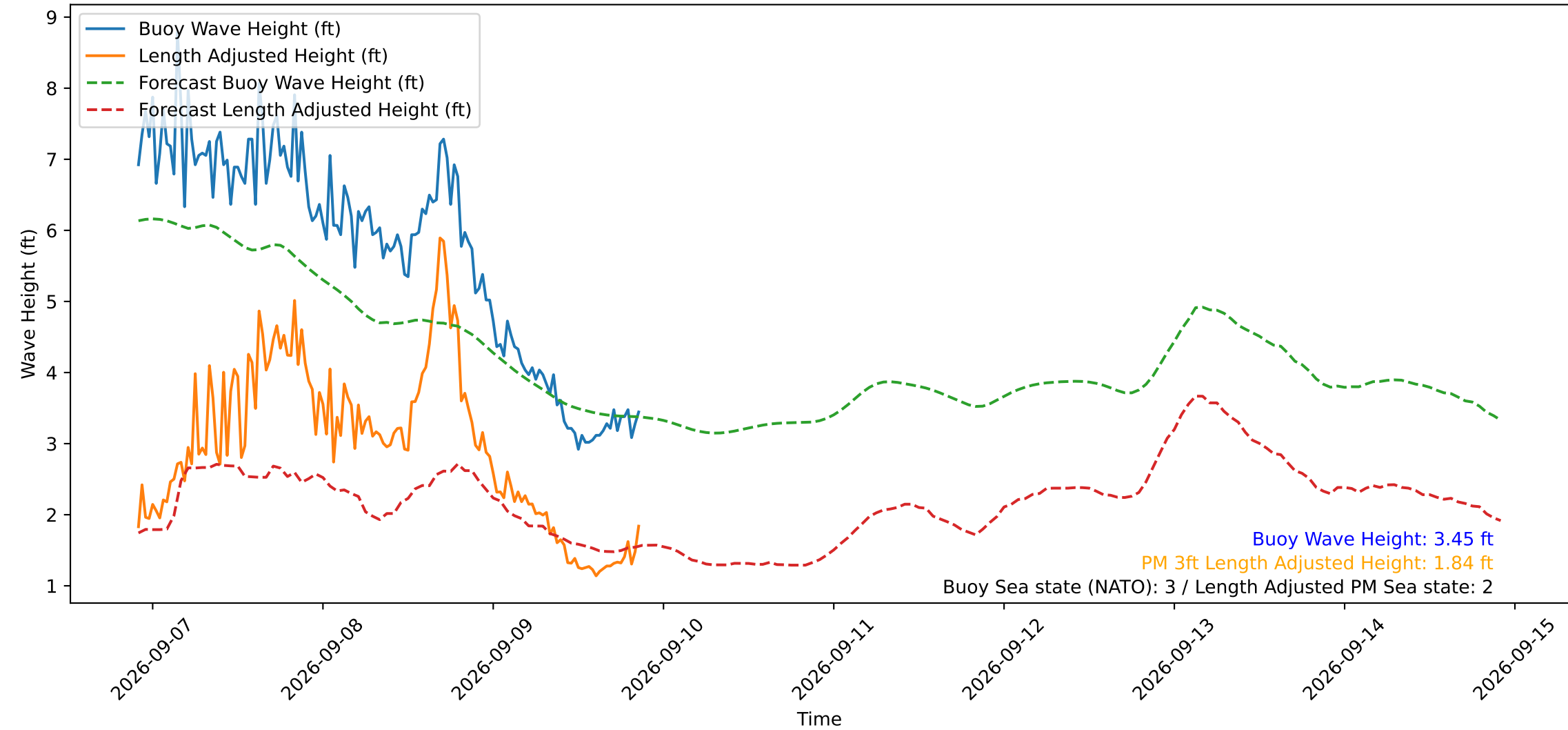
Wave Heights over Time for Green Beach at 2026-09-09 21:31:11
