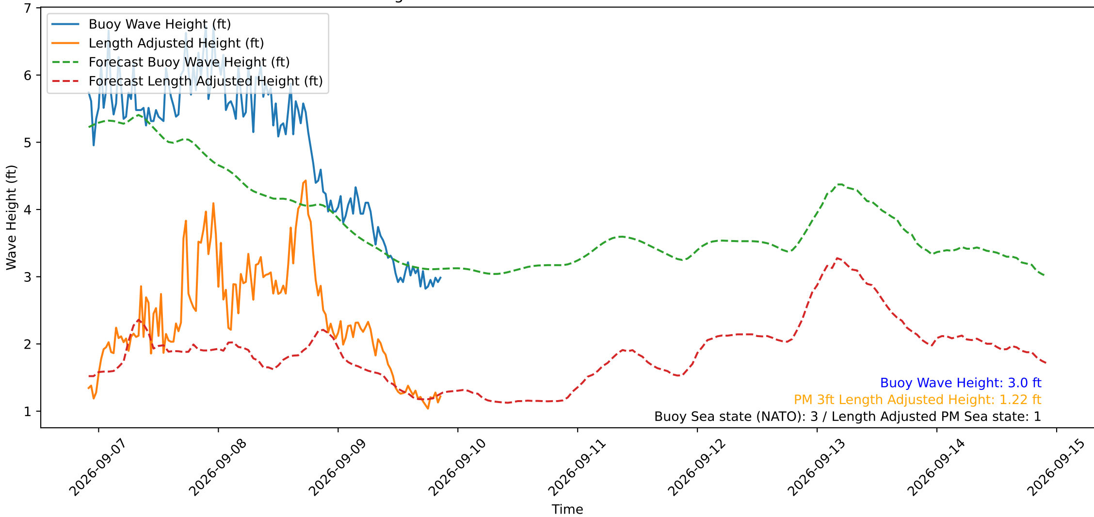
Wave Heights over Time for Red Beach at 2026-09-09 21:30:49
