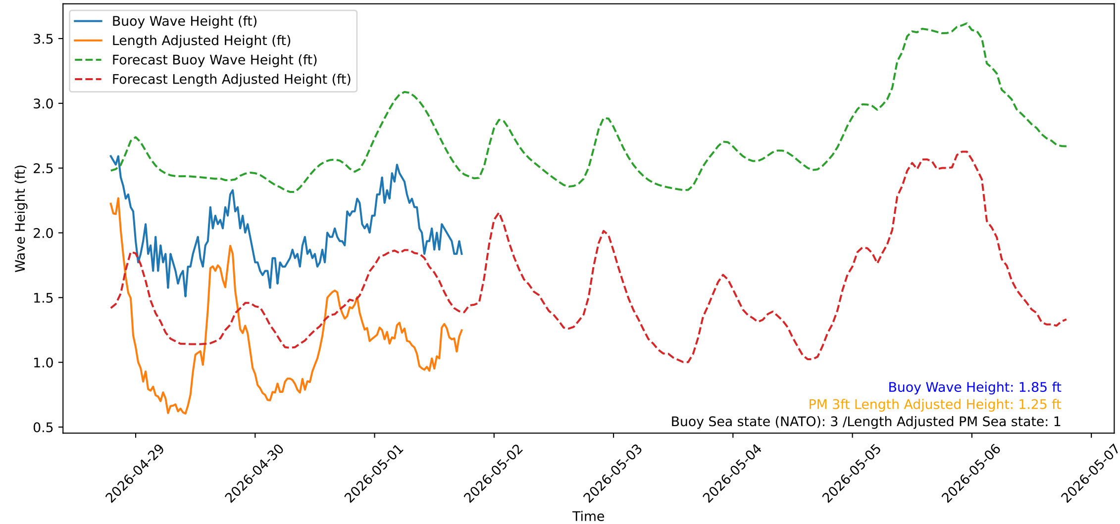
Wave Heights over Time for Red Beach at 2026-05-01 18:30:51
