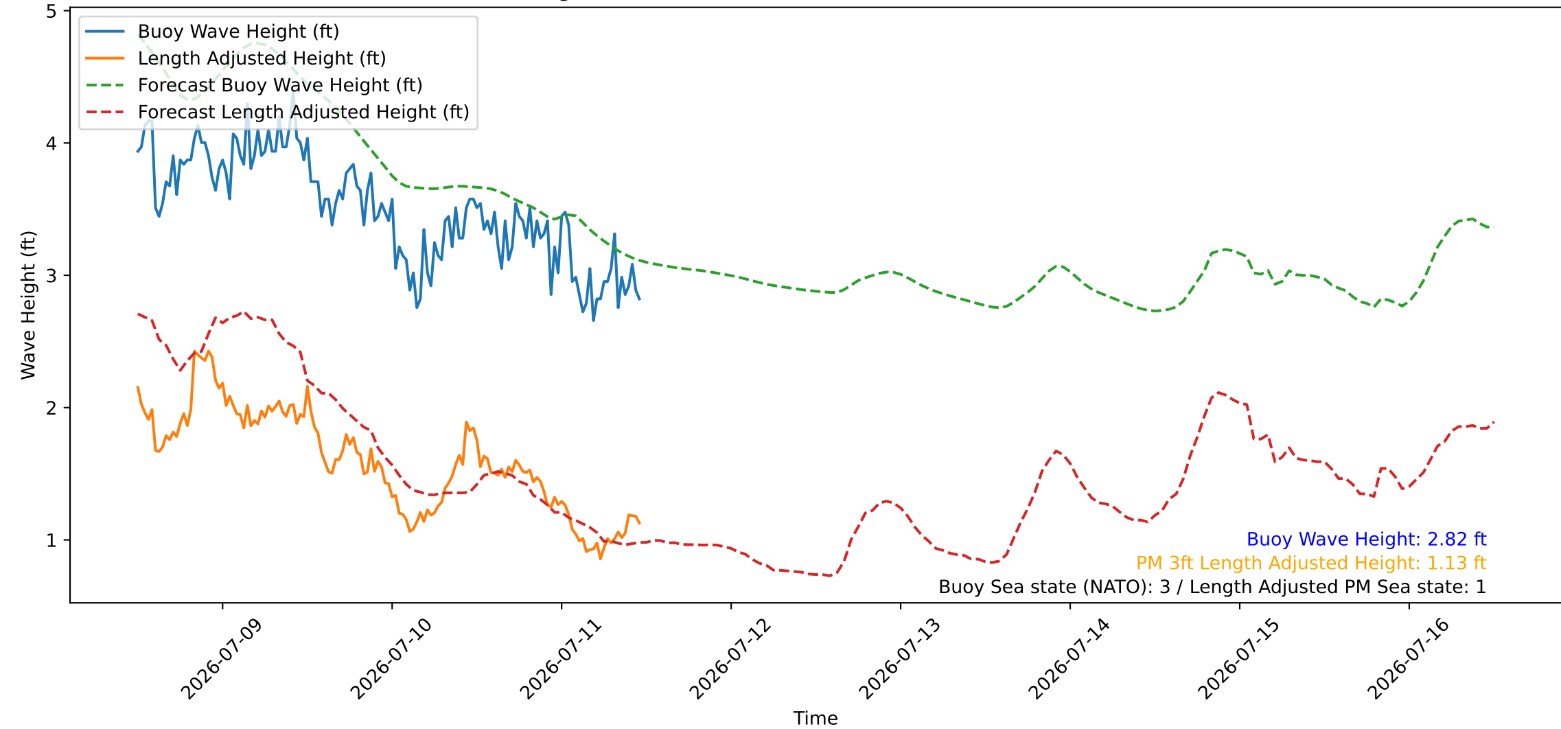
Wave Heights over Time for Green Beach at 2026-07-11 11:51:09
