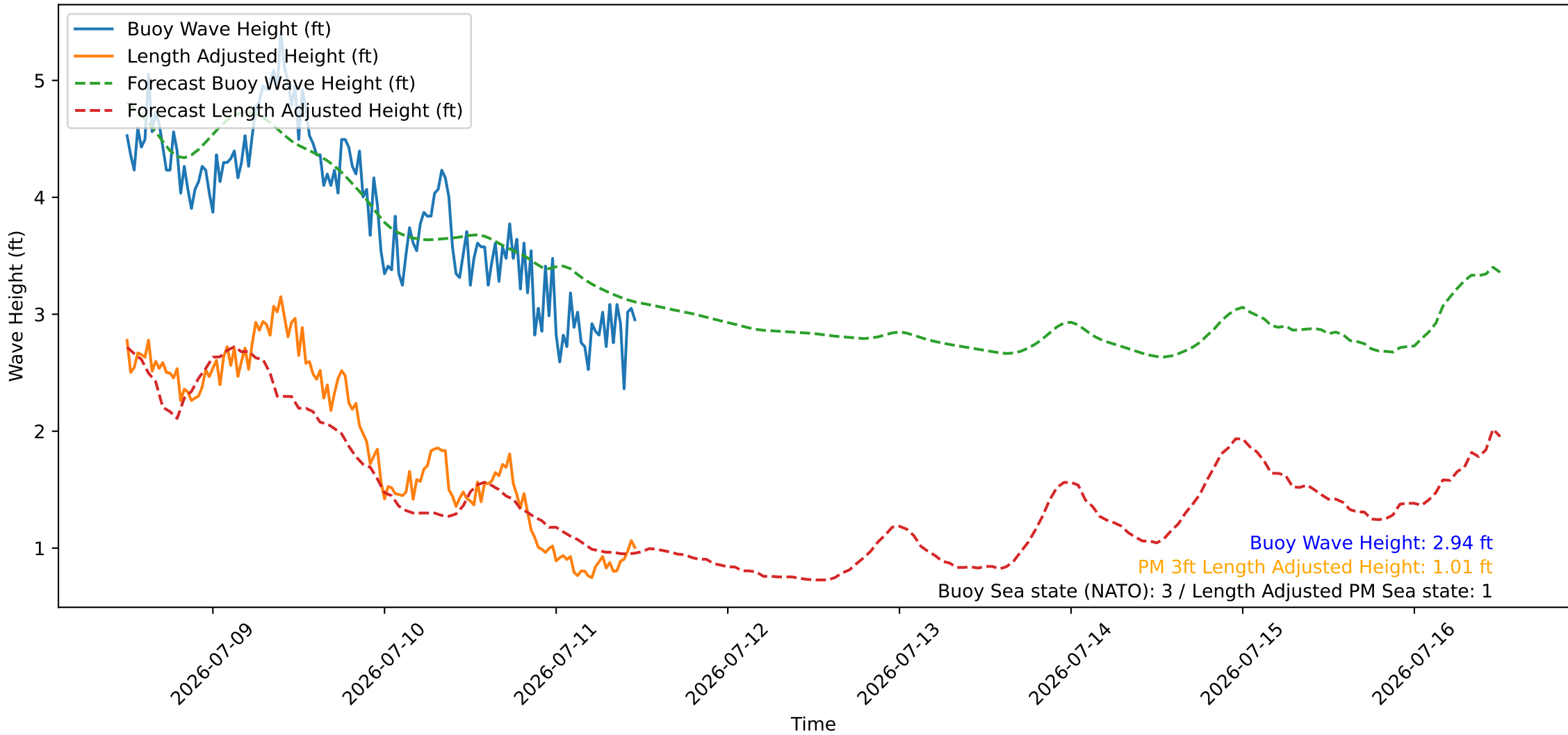
Wave Heights over Time for Oceanside Harbor at 2026-07-11 11:50:26
