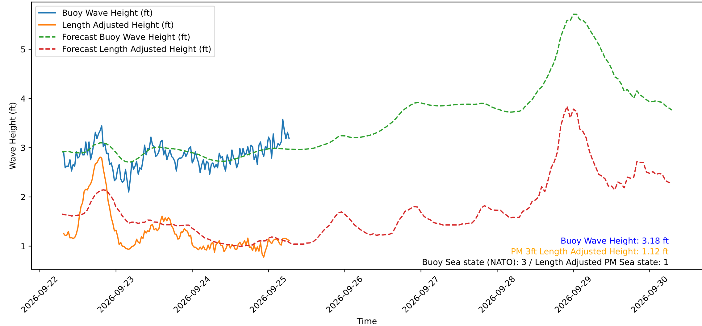
Wave Heights over Time for Green Beach at 2026-09-25 07:11:12
