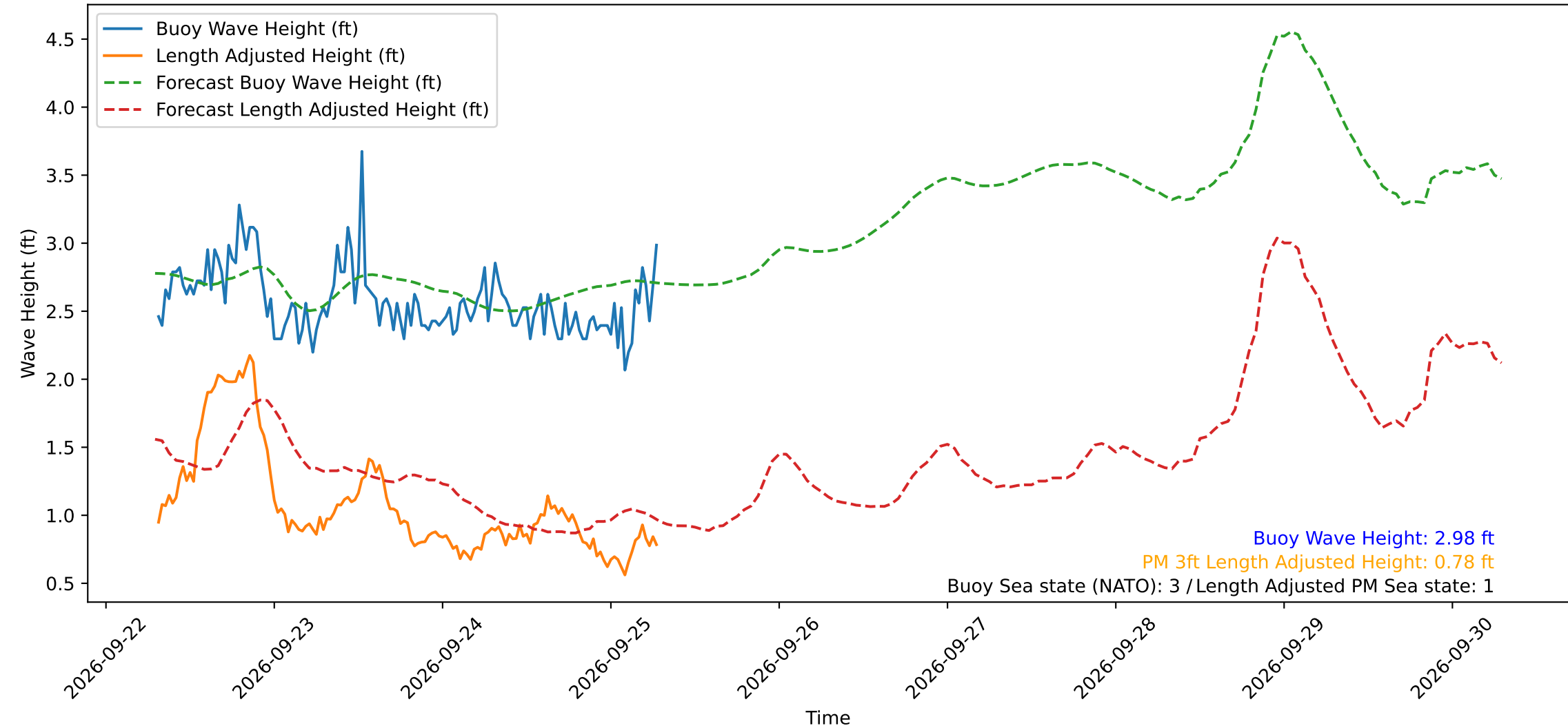
Wave Heights over Time for Red Beach at 2026-09-25 07:10:49
