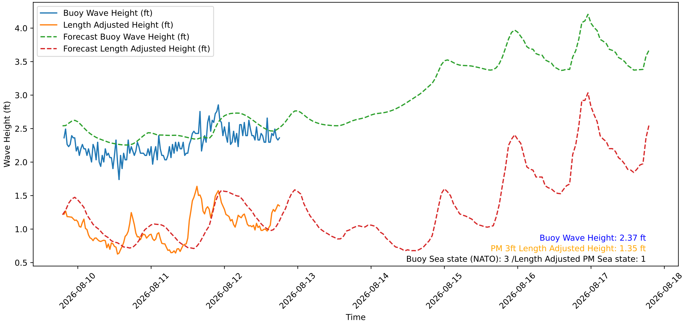
Wave Heights over Time for Red Beach at 2026-08-12 19:00:46
