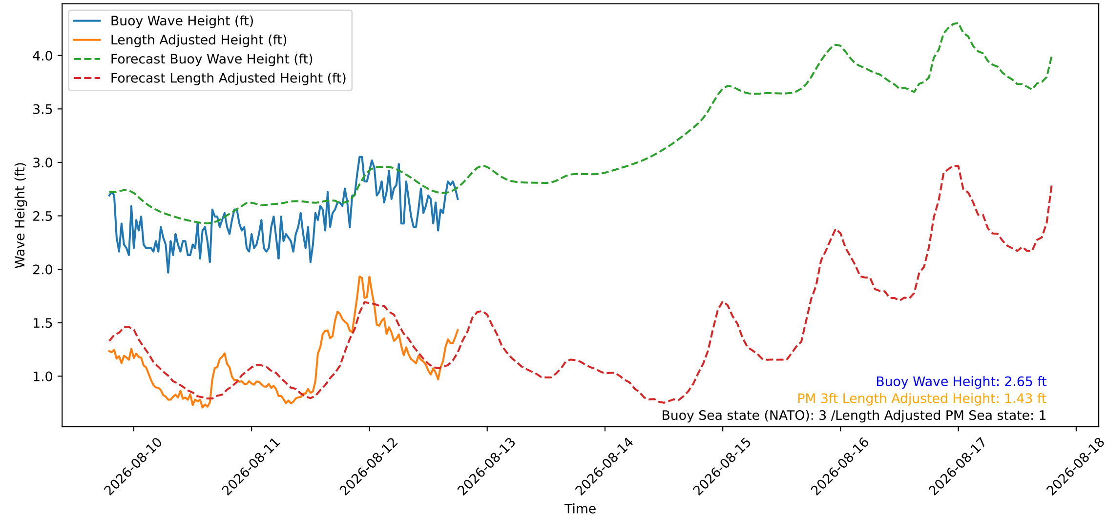
Wave Heights over Time for Oceanside Harbor at 2026-08-12 19:00:27
