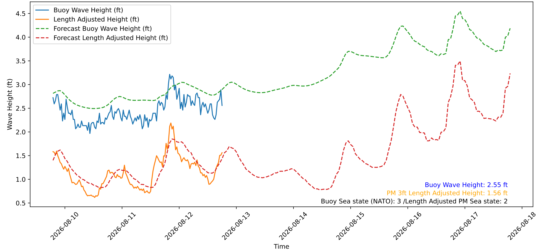
Wave Heights over Time for Green Beach at 2026-08-12 19:01:09
