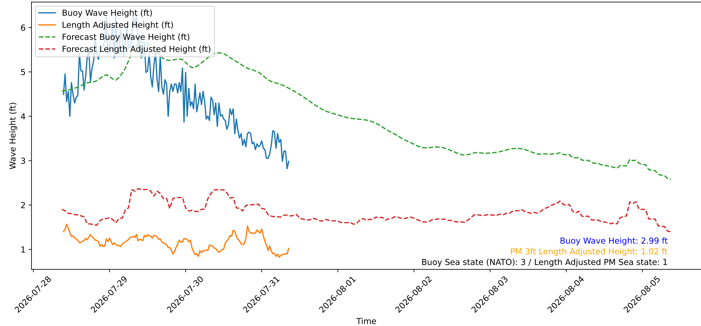
Wave Heights over Time for Green Beach at 2026-07-31 09:21:11
