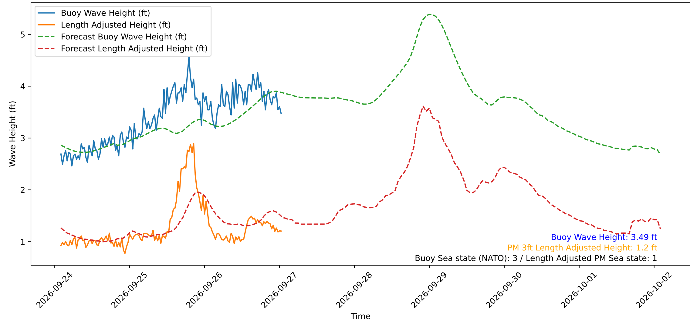
Wave Heights over Time for Green Beach at 2026-09-27 01:51:16
