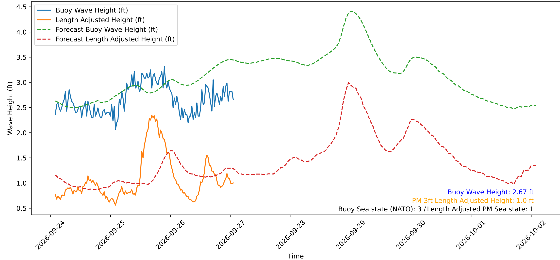
Wave Heights over Time for Red Beach at 2026-09-27 01:50:51
