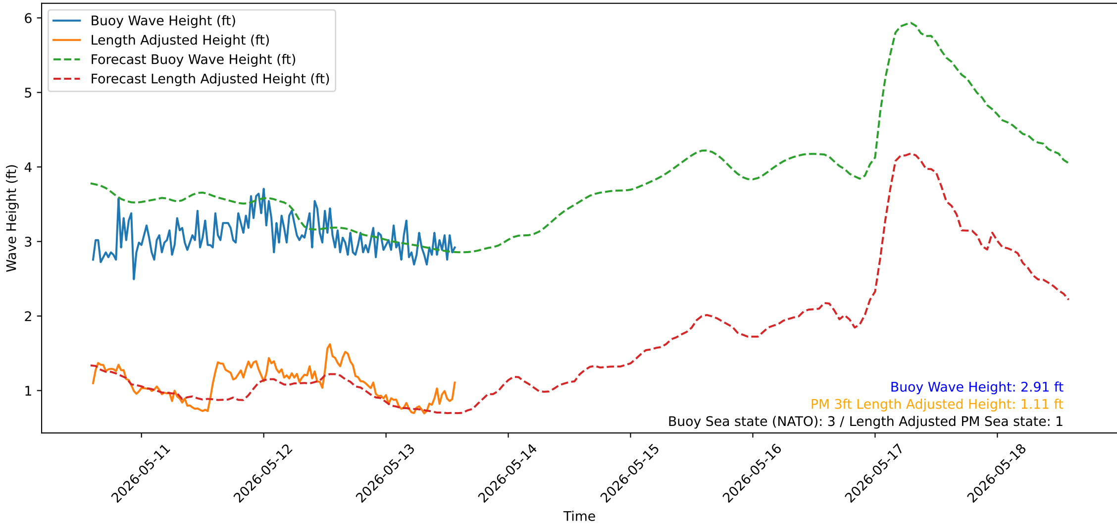
Wave Heights over Time for Oceanside Harbor at 2026-05-13 14:20:31
